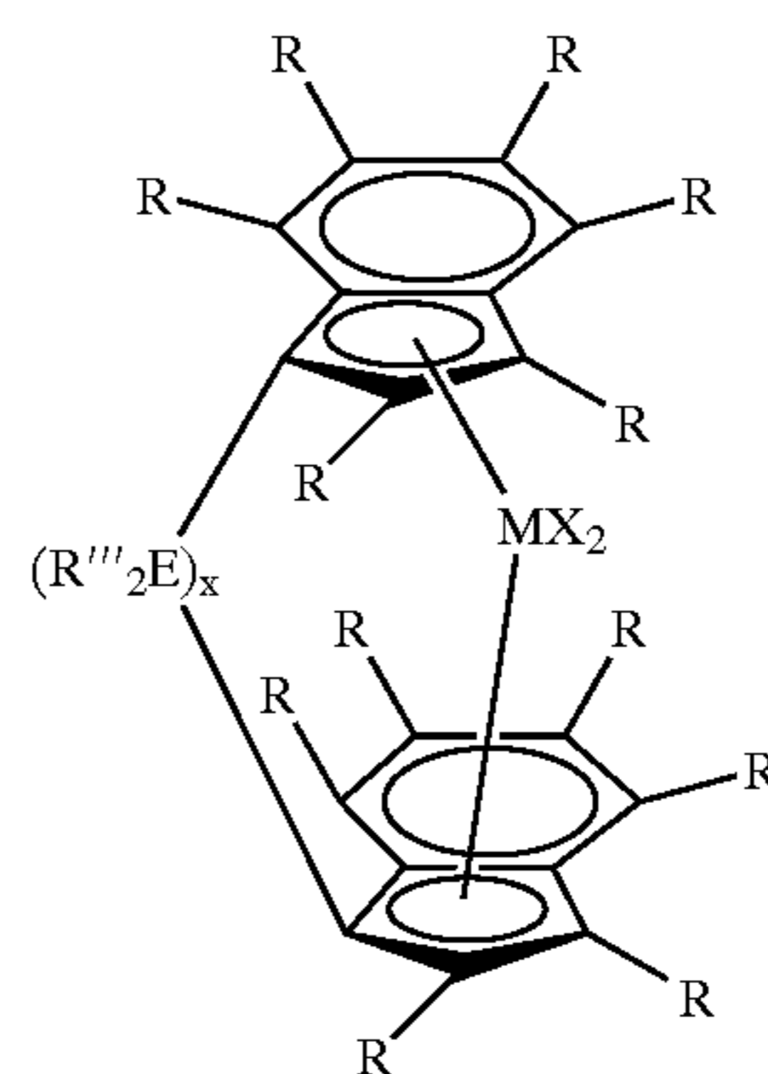
meso bis(indenyl) metallocene
