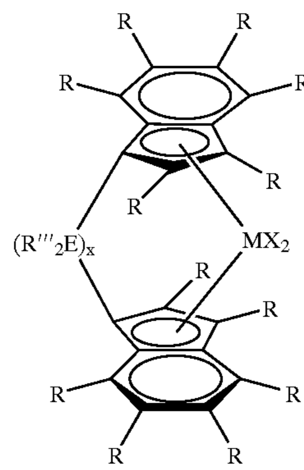
rac bis(indenyl) metallocene
