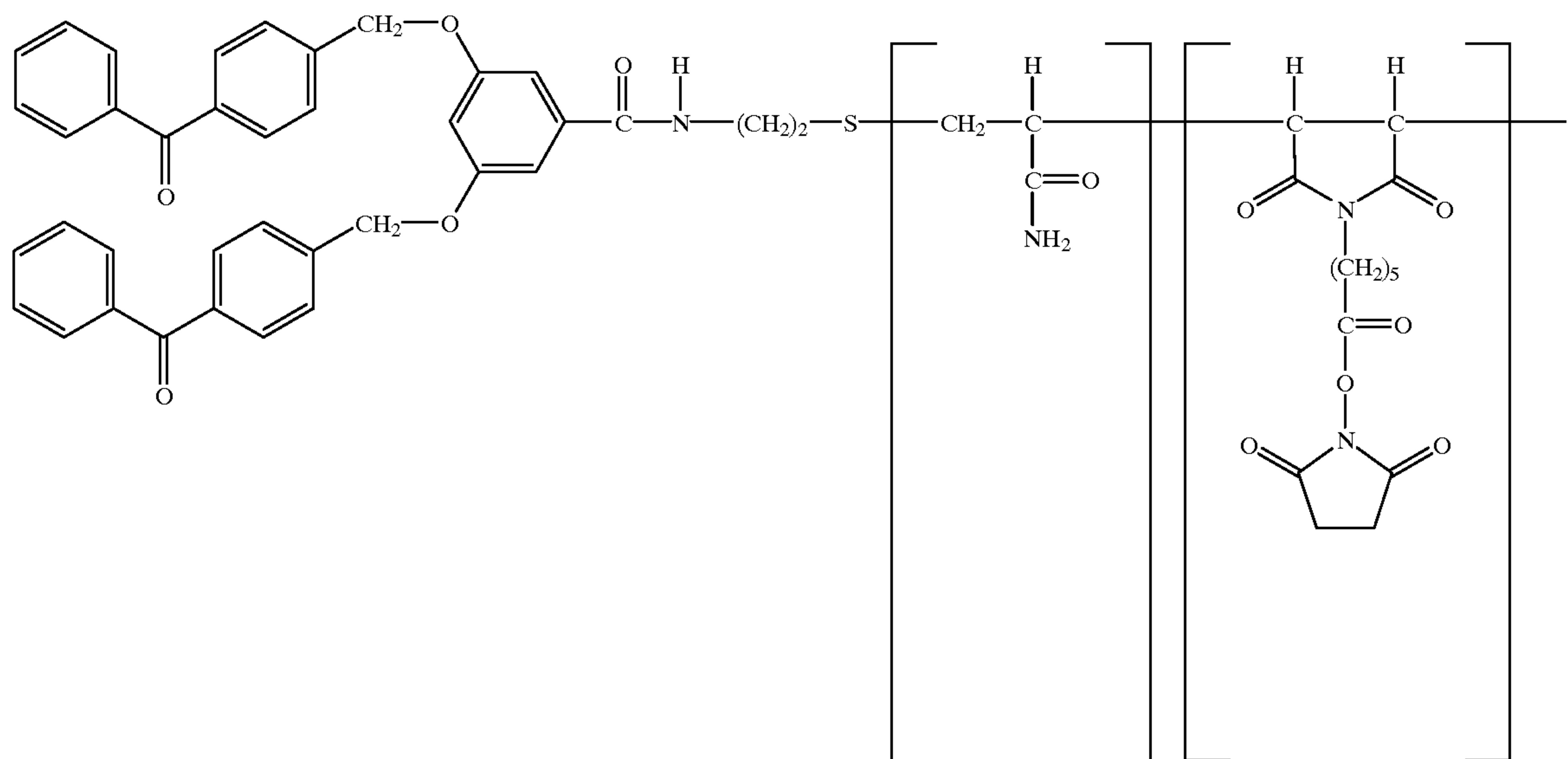
COMPOUND XII
