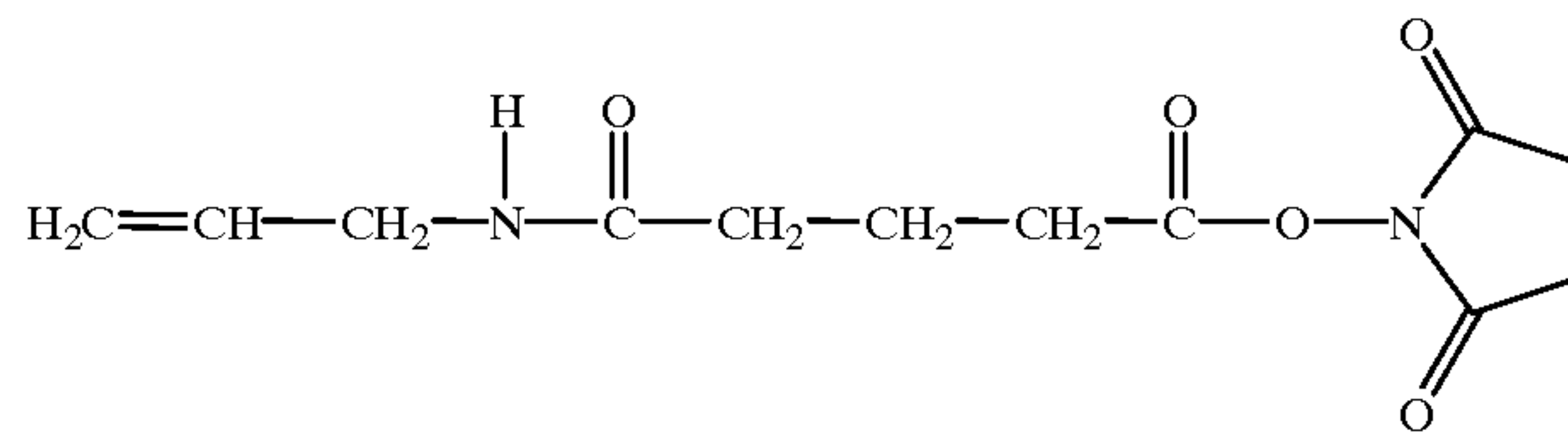
COMPOUND XIV
