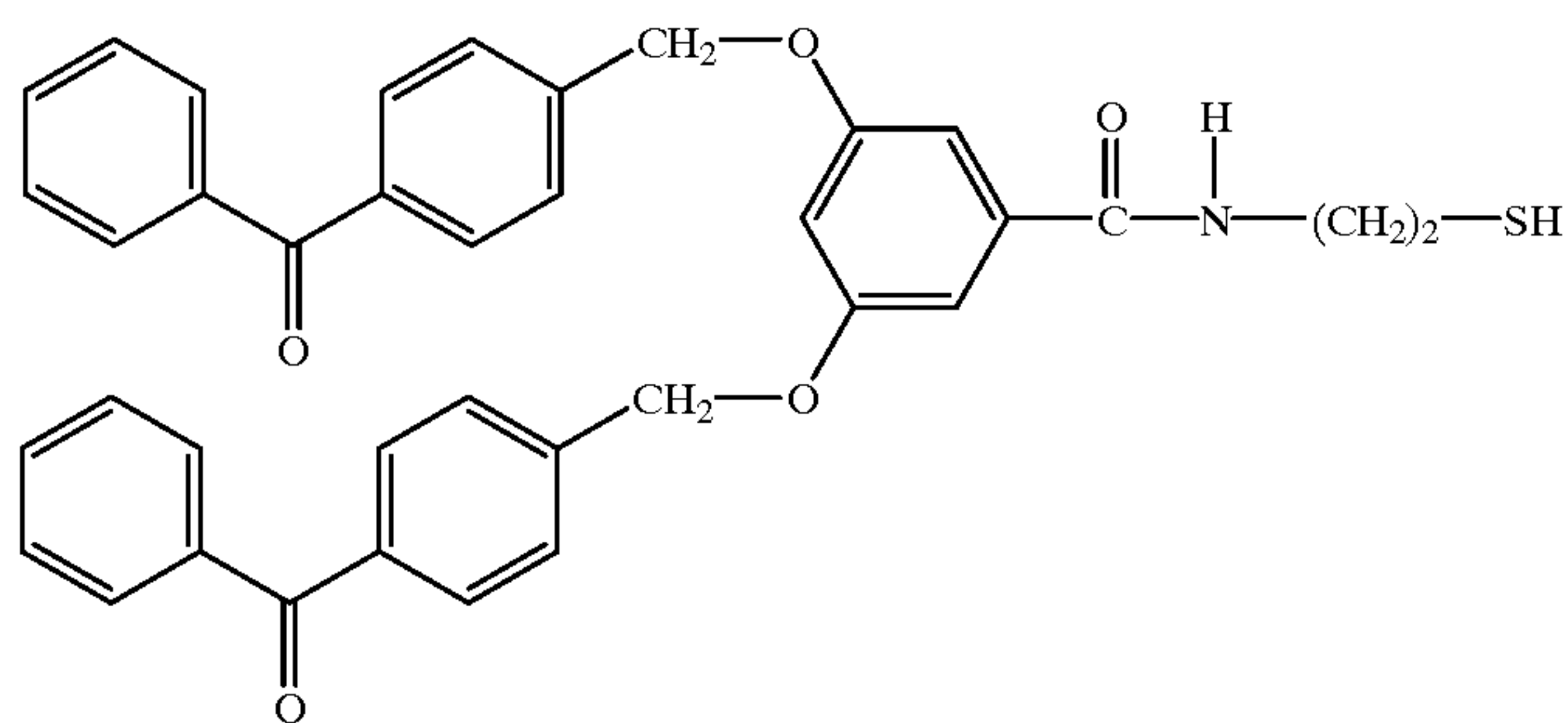
COMPOUND VII
