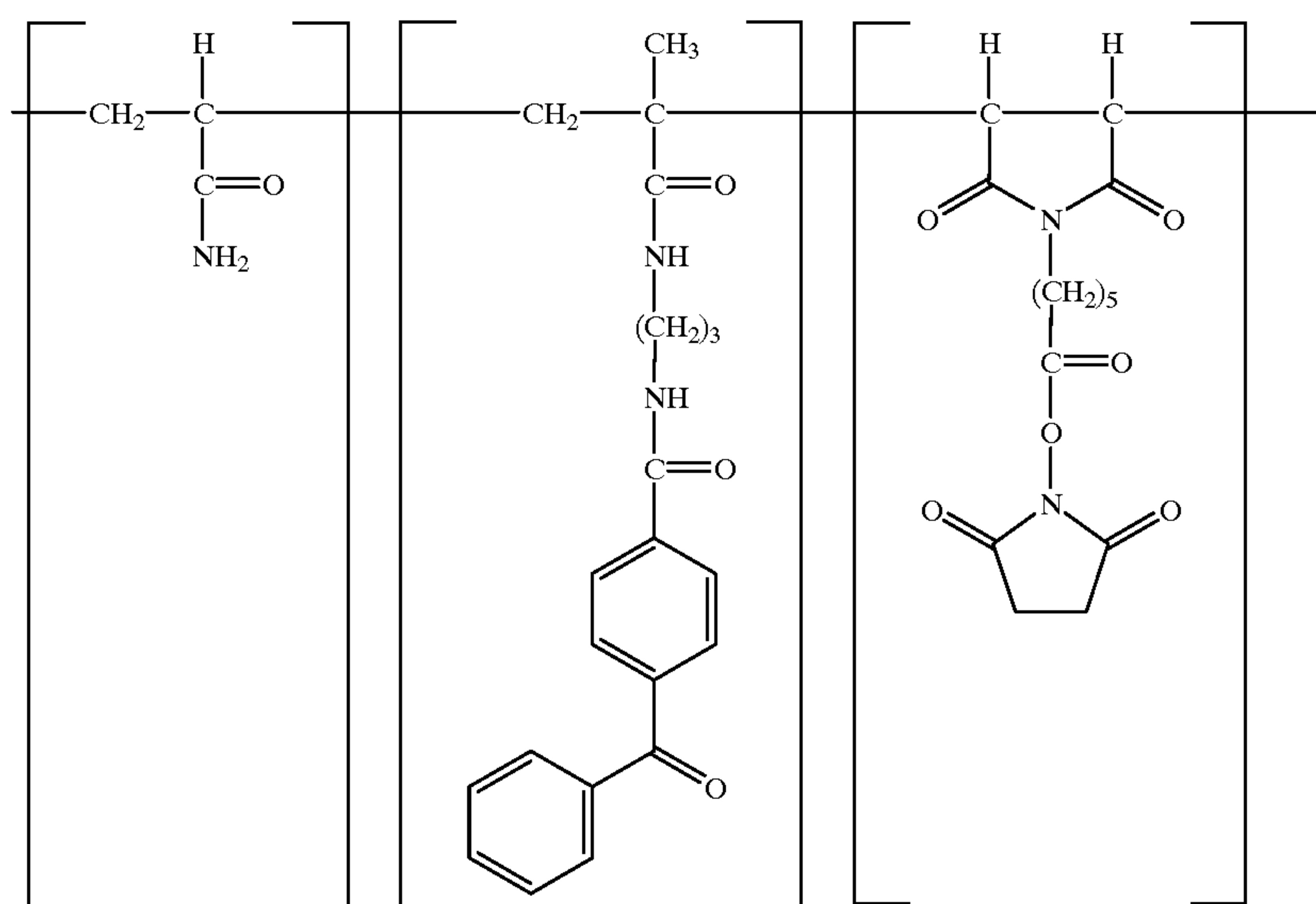
COMPOUND IX
