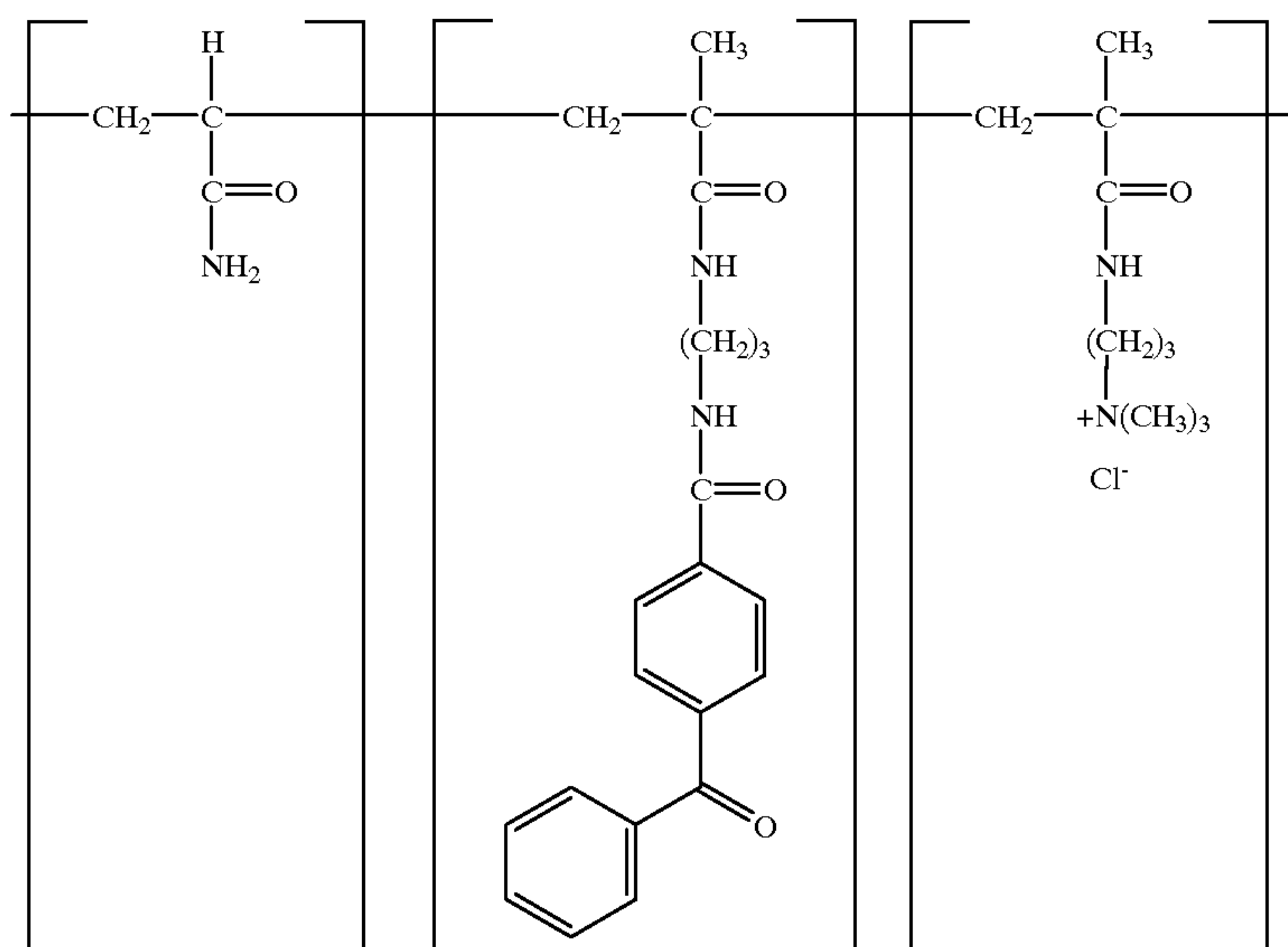
COMPOUND X
