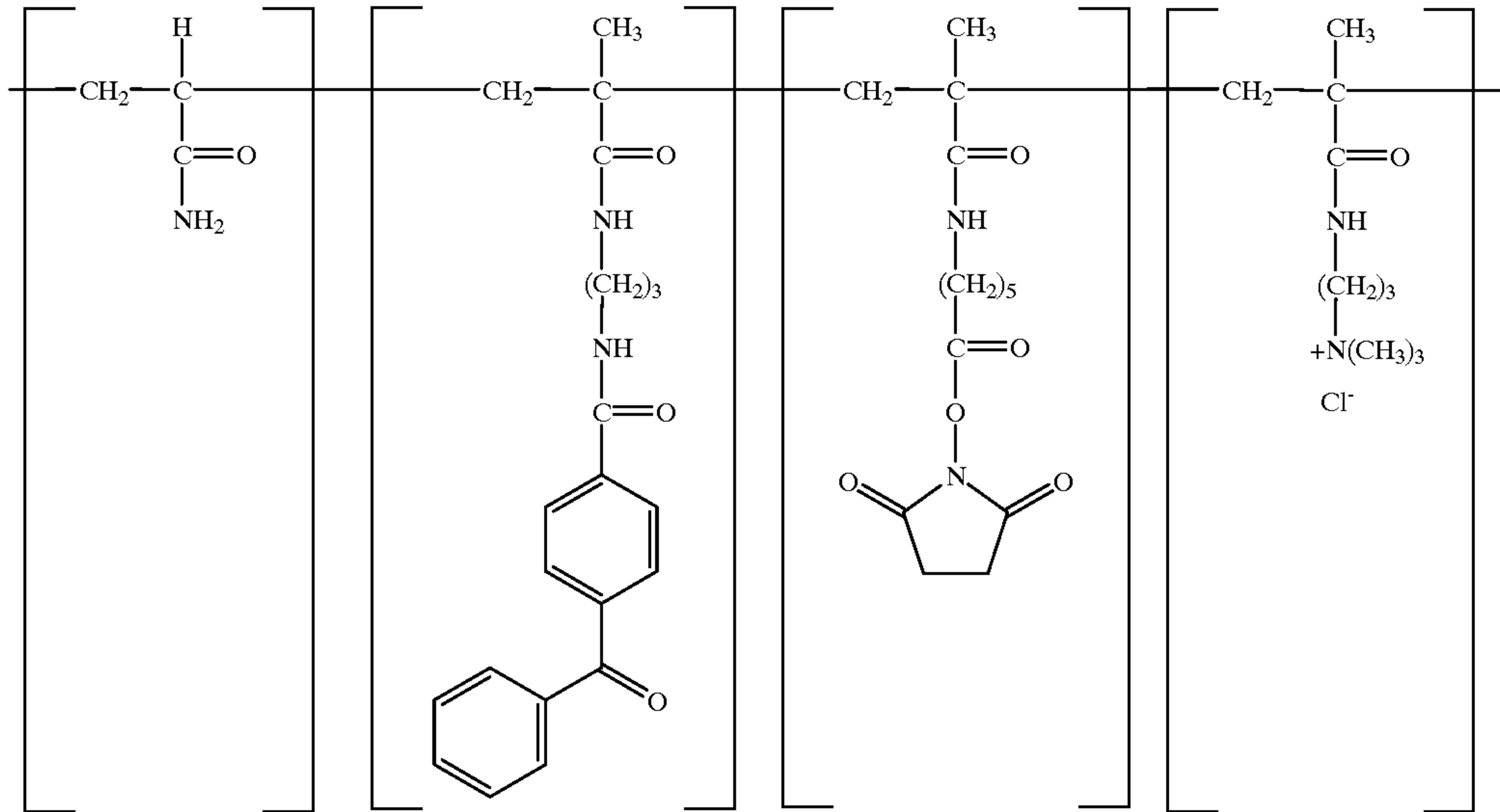
COMPOUND XI
