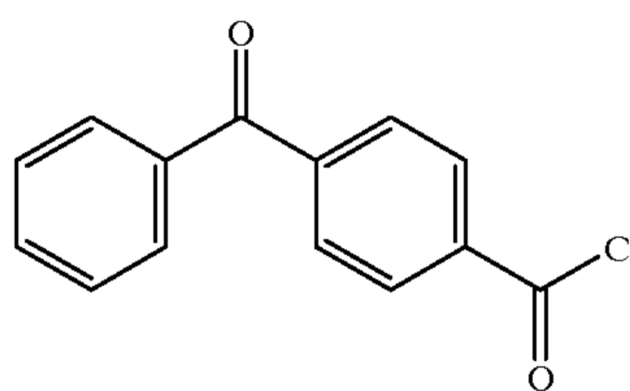
COMPOUND I
