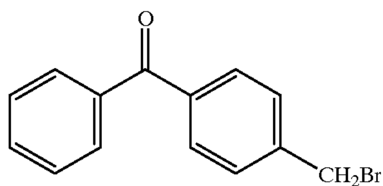
COMPOUND VI
