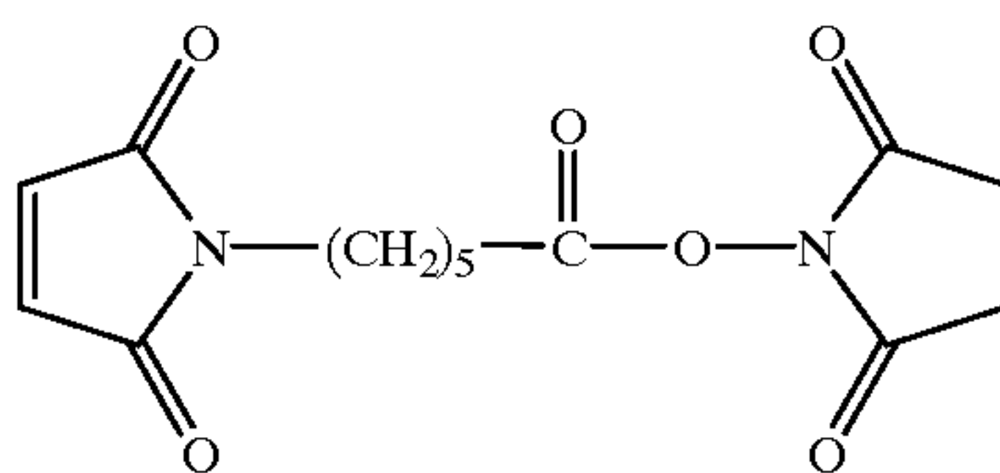
COMPOUND IV
