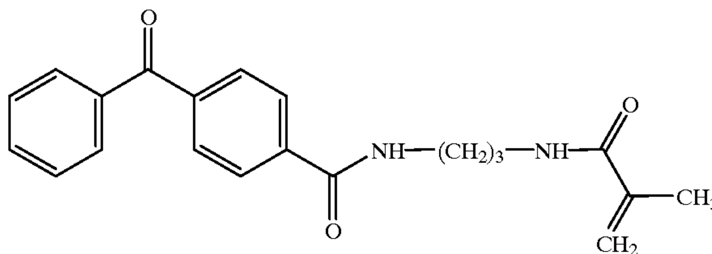
COMPOUND III
