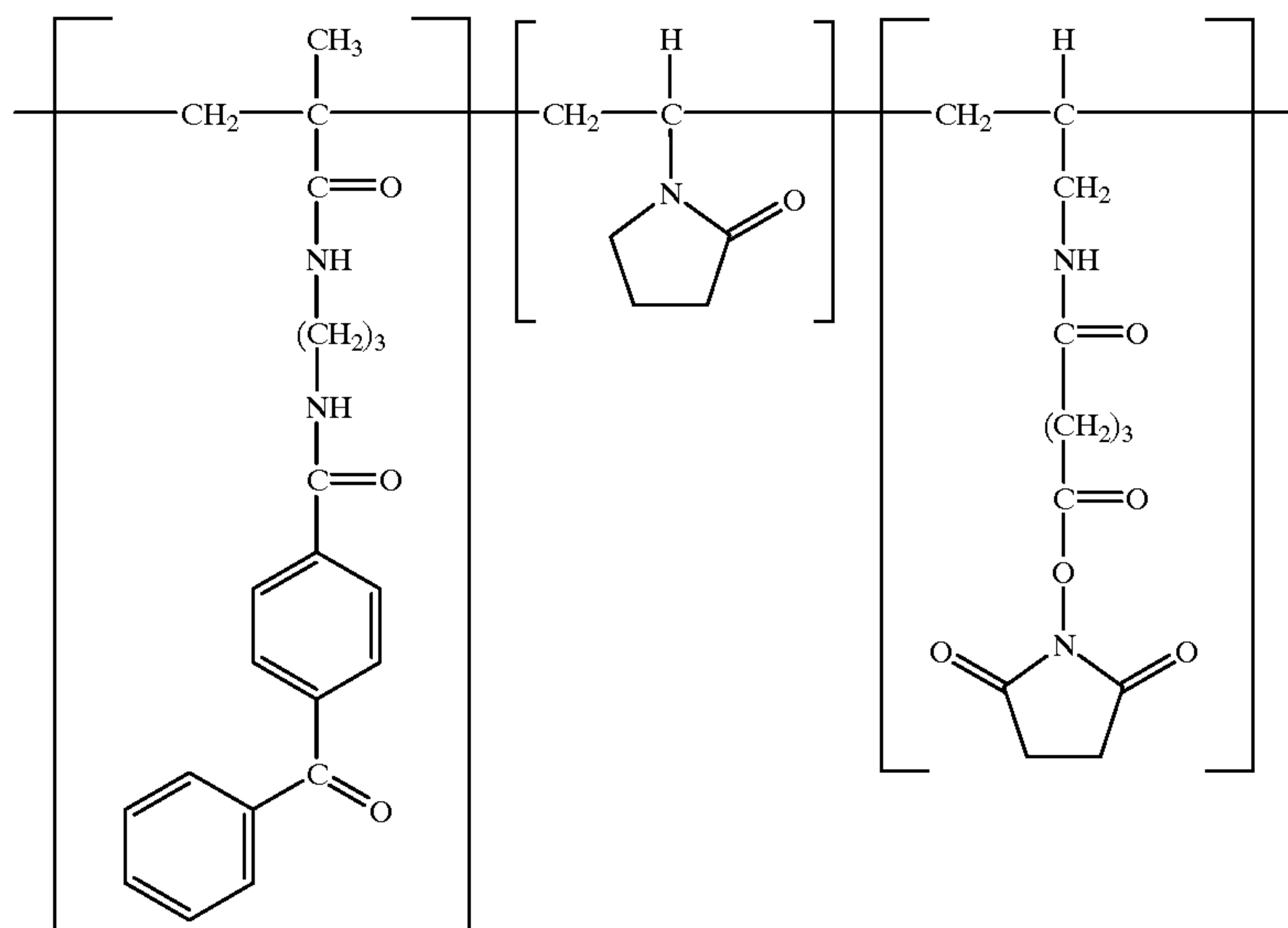
Compound XV
