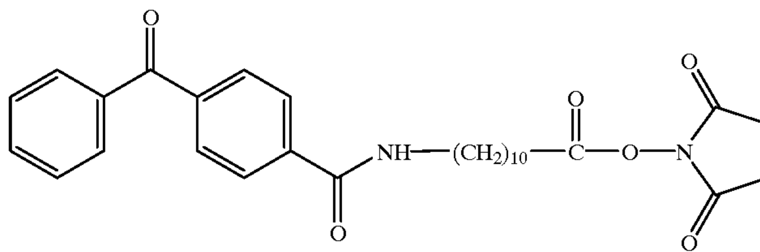
COMPOUND VIII
