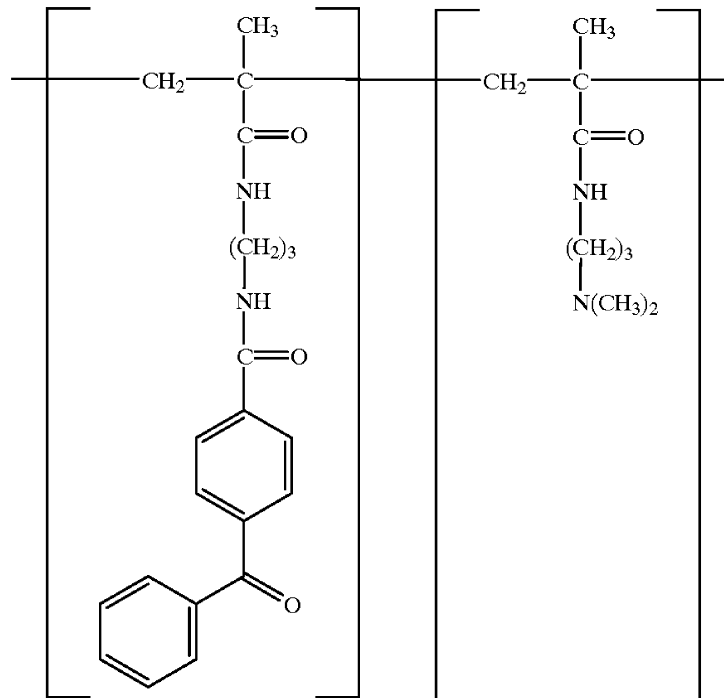
COMPOUND XIII
