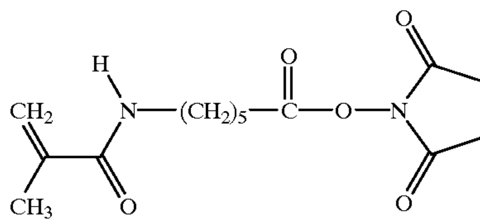
COMPOUND V
