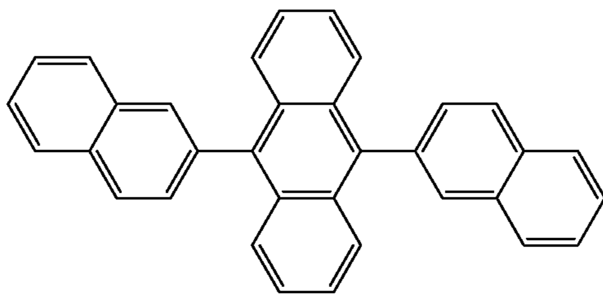
Compound 26
