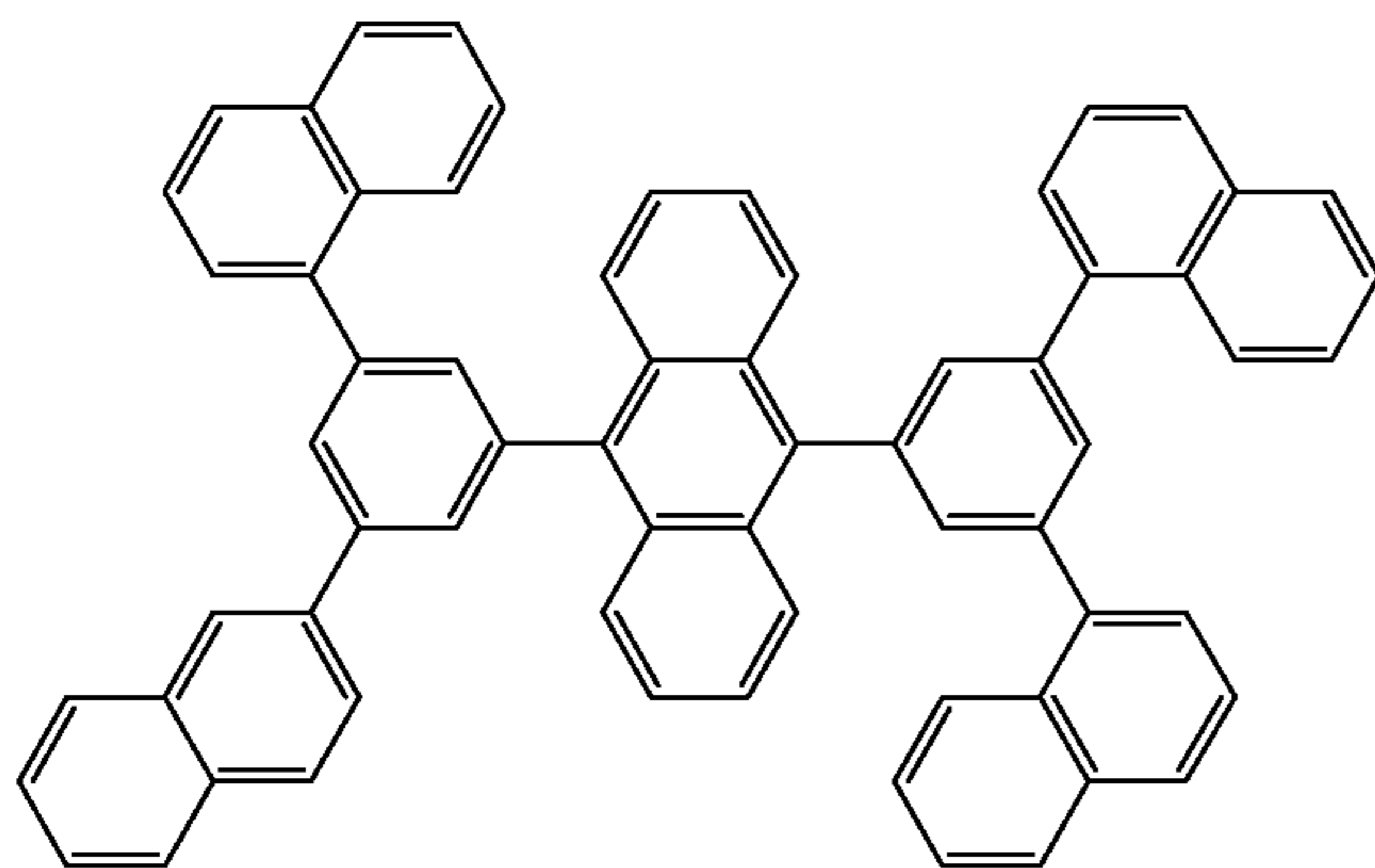
Compound 21
