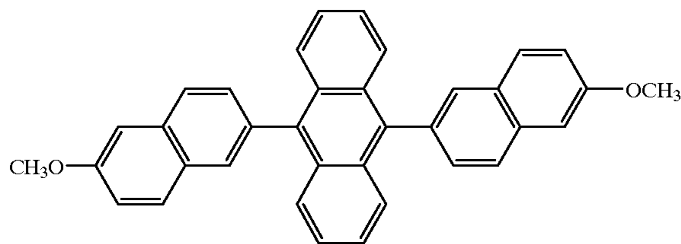
Compound 43
