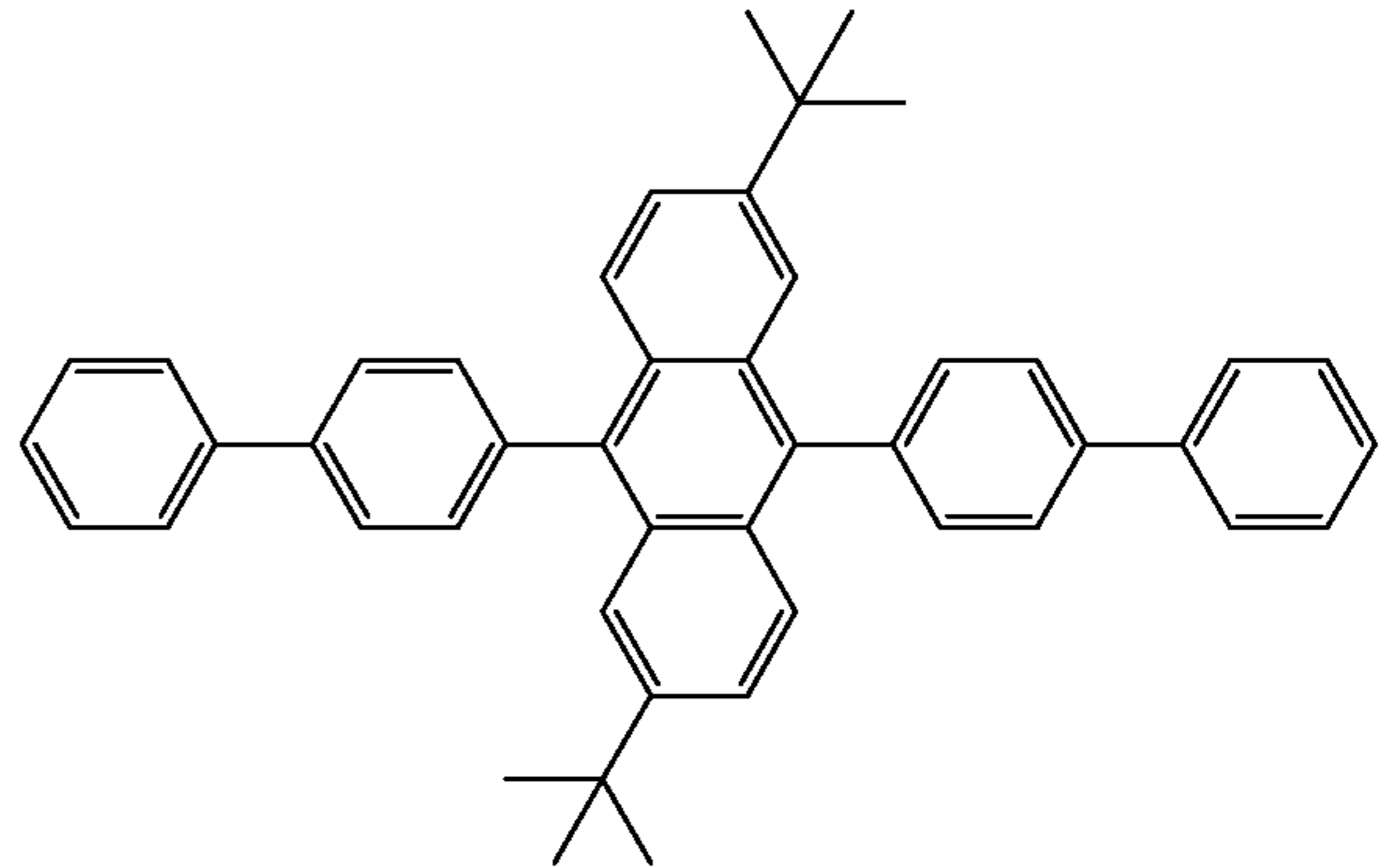
Compound 11
