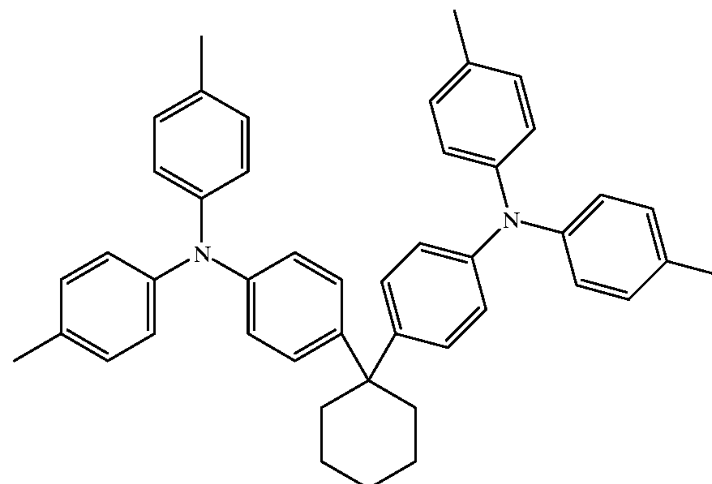
Compound 1
