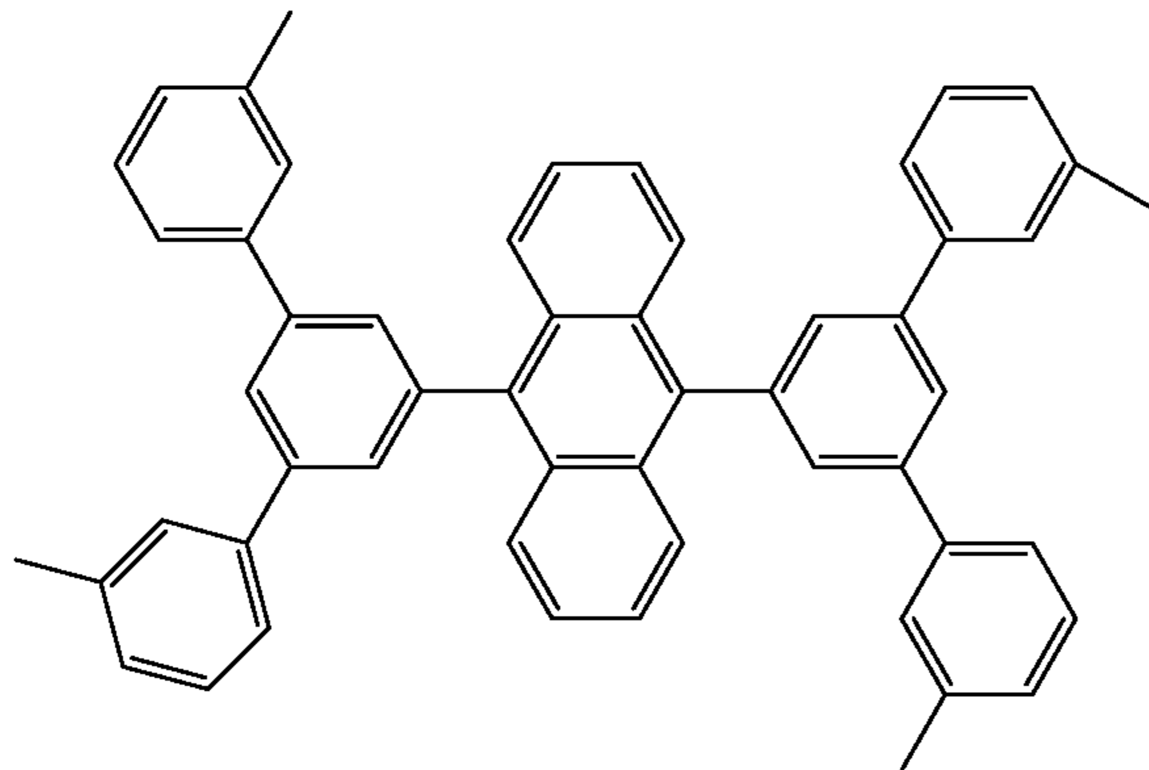
Compound 20
