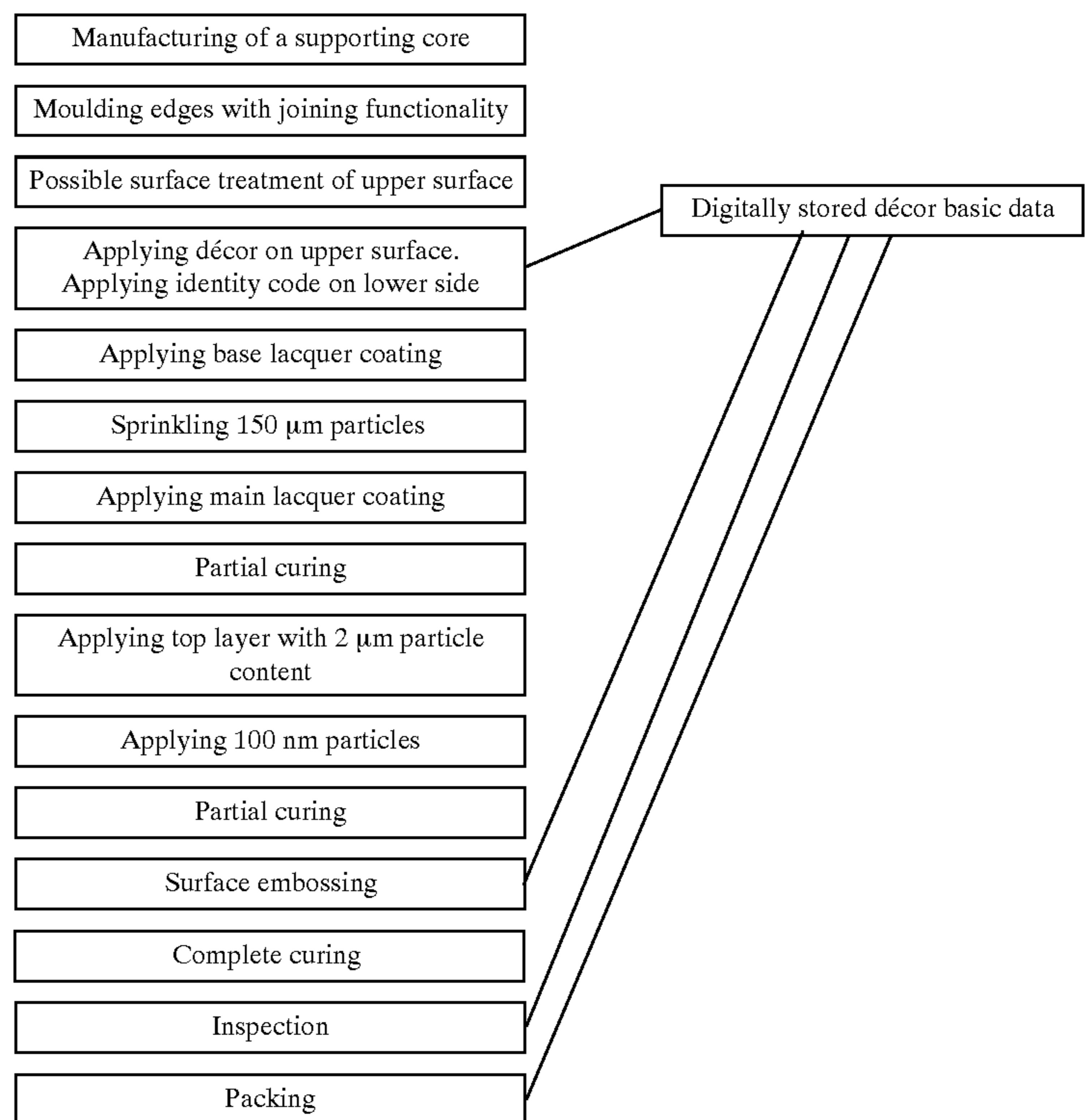
Process scheme 1.
