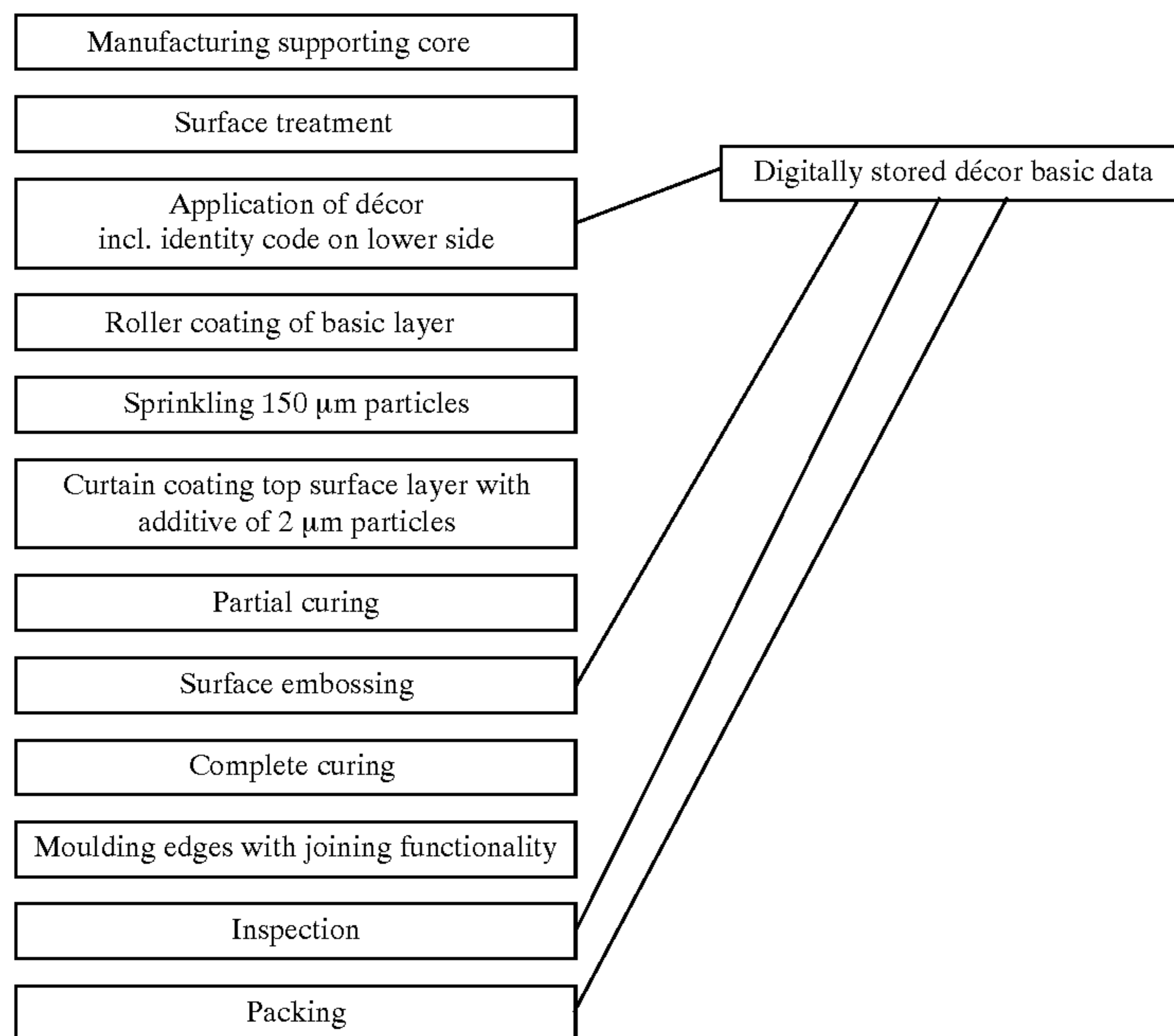
Process scheme 2
