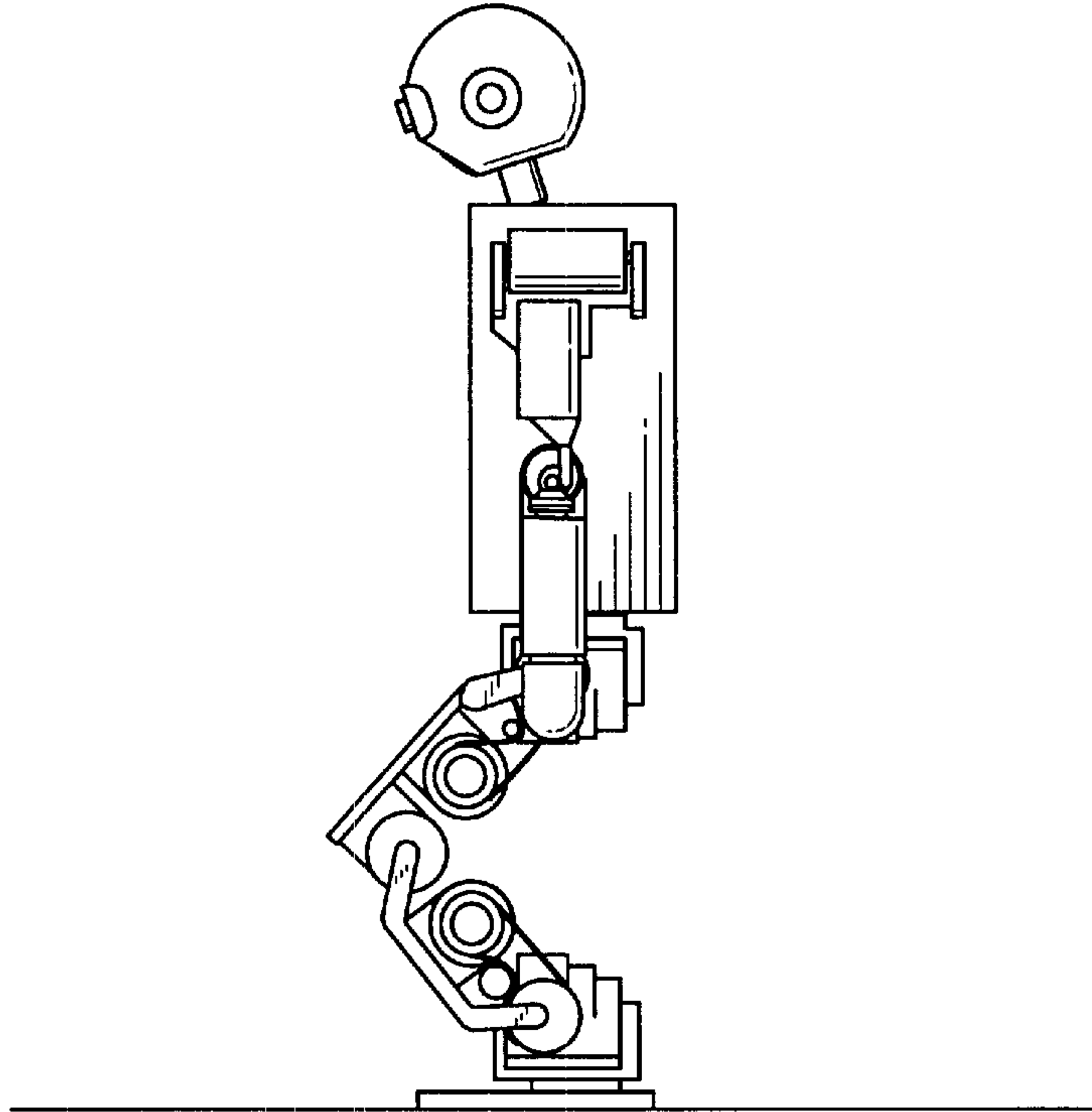
FIG. 47 (PRIOR ART)
