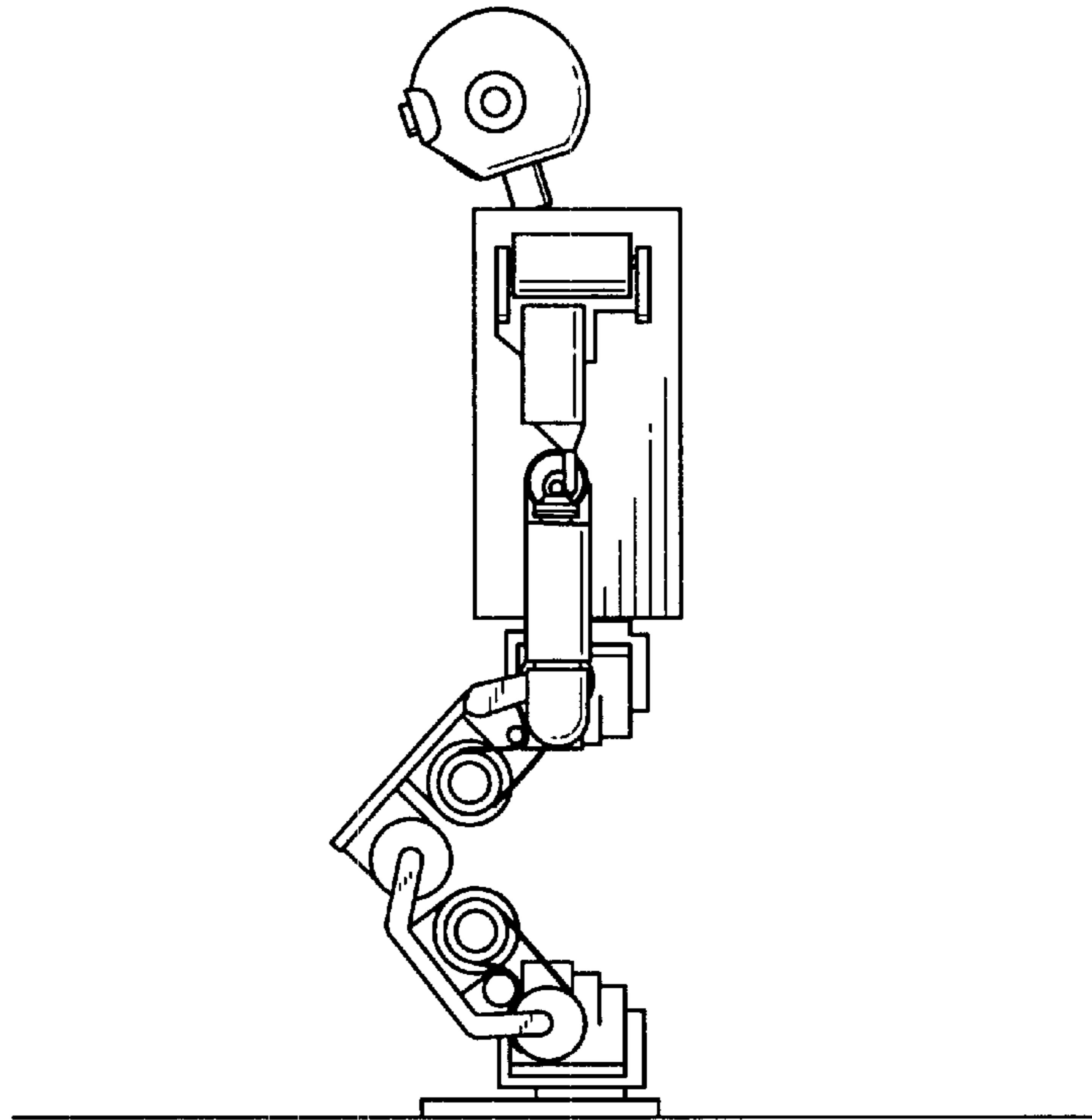
FIG. 47 (PRIOR ART)
