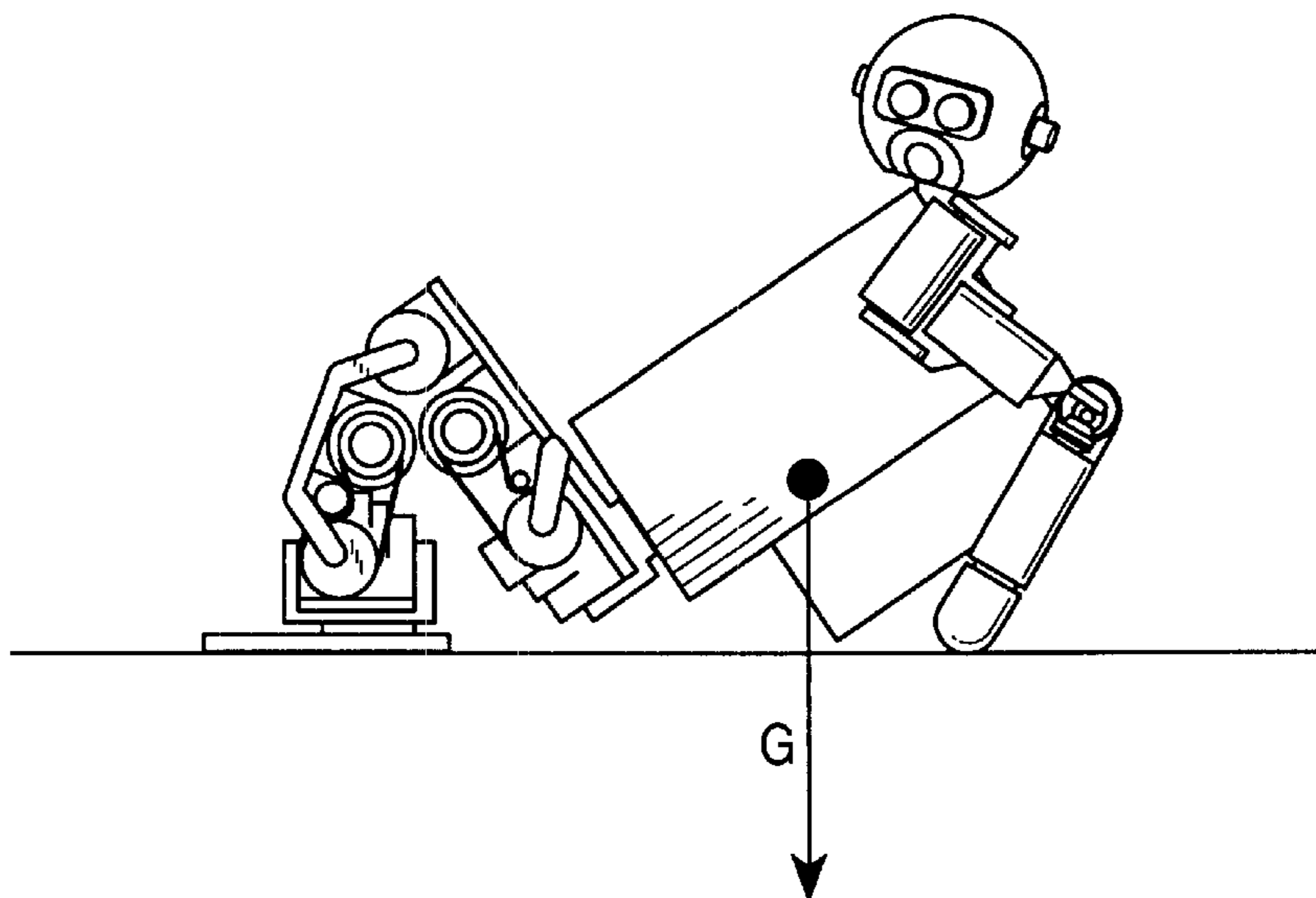
FIG. 48 (PRIOR ART)
