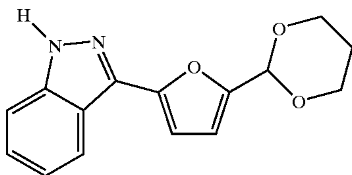
3-(5-(1,3-Dioxan-2-yl)furan-2-yl)indazole
