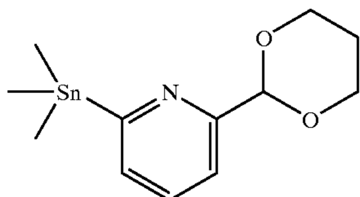
2-(1,3-Dioxan-2-yl)-6-trimethylstannylpyridine
