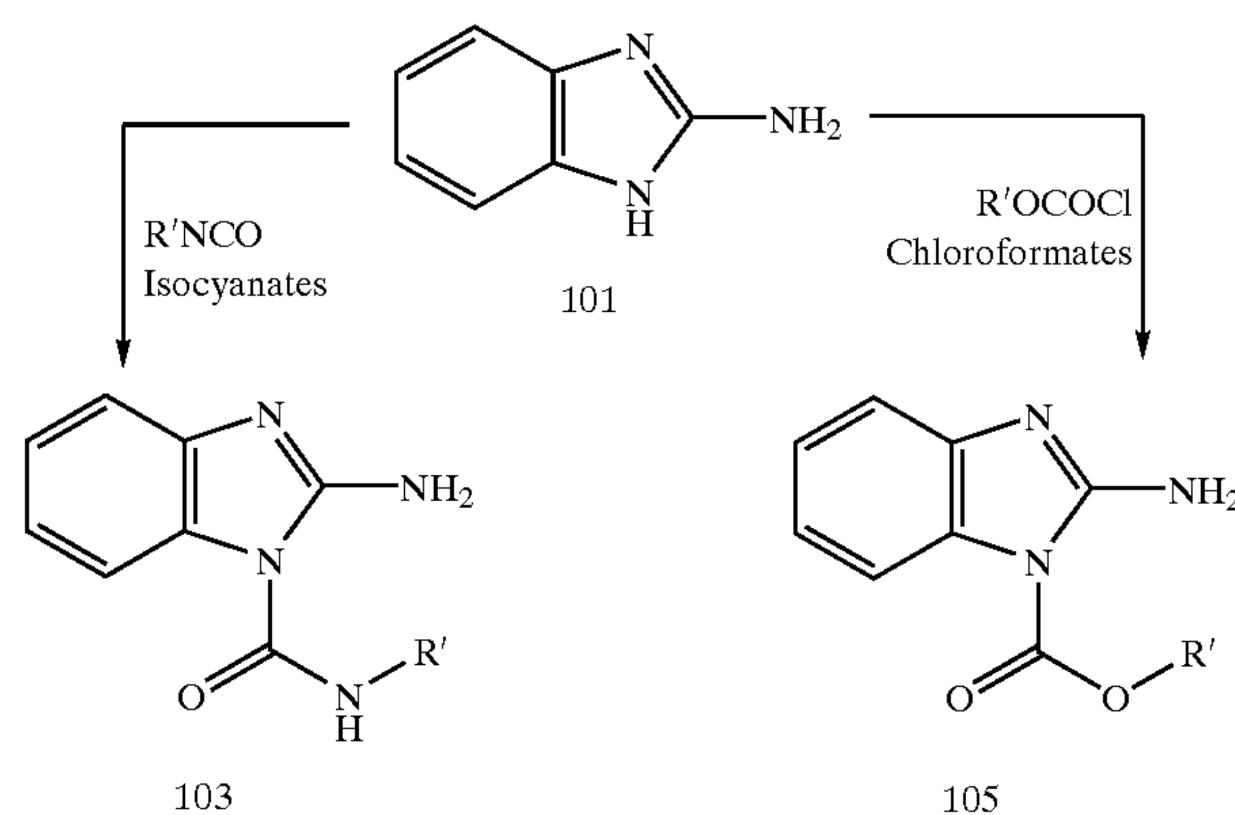
Reaction Scheme 1
