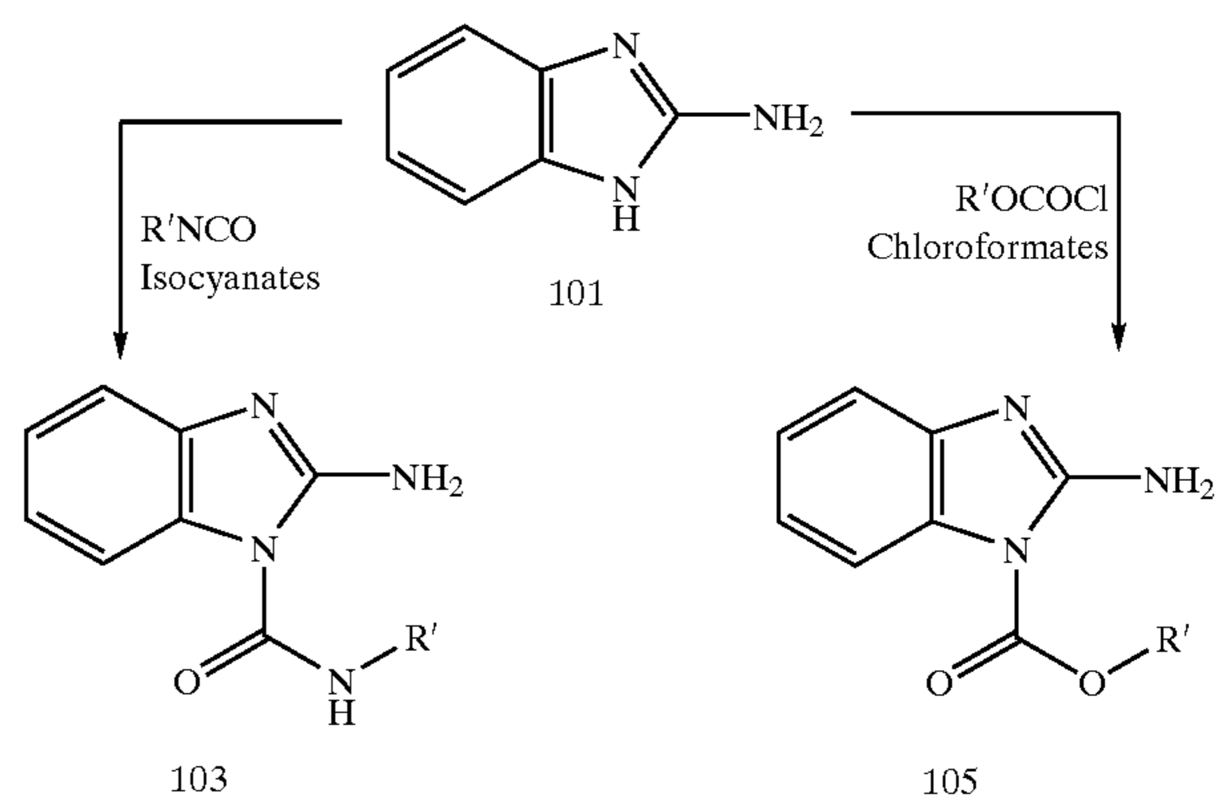
Reaction Scheme 1
