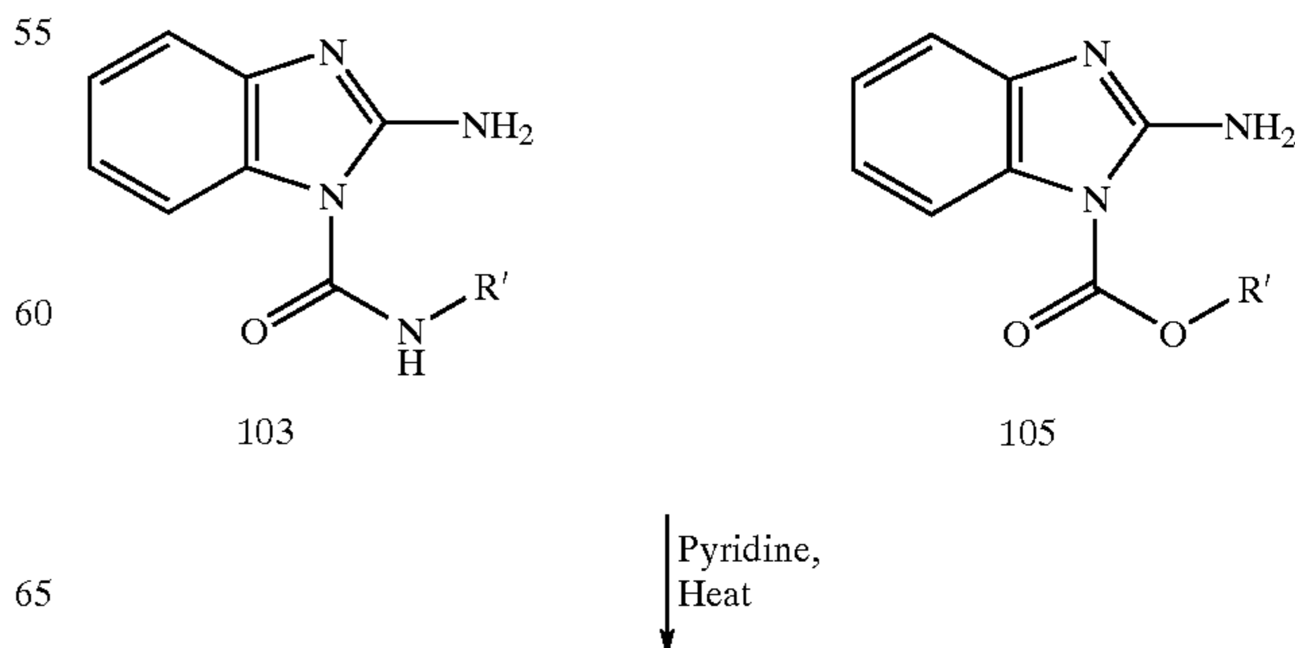
Reaction Scheme 2
