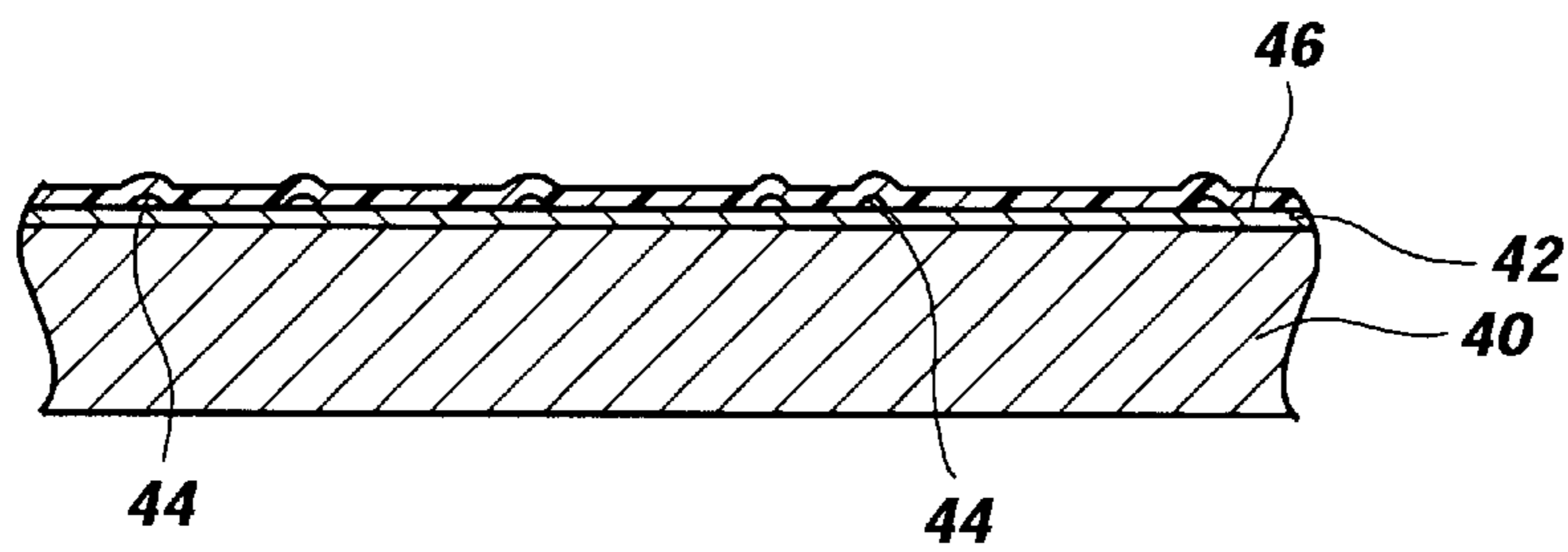
Fig. 4 (PRIOR ART)
