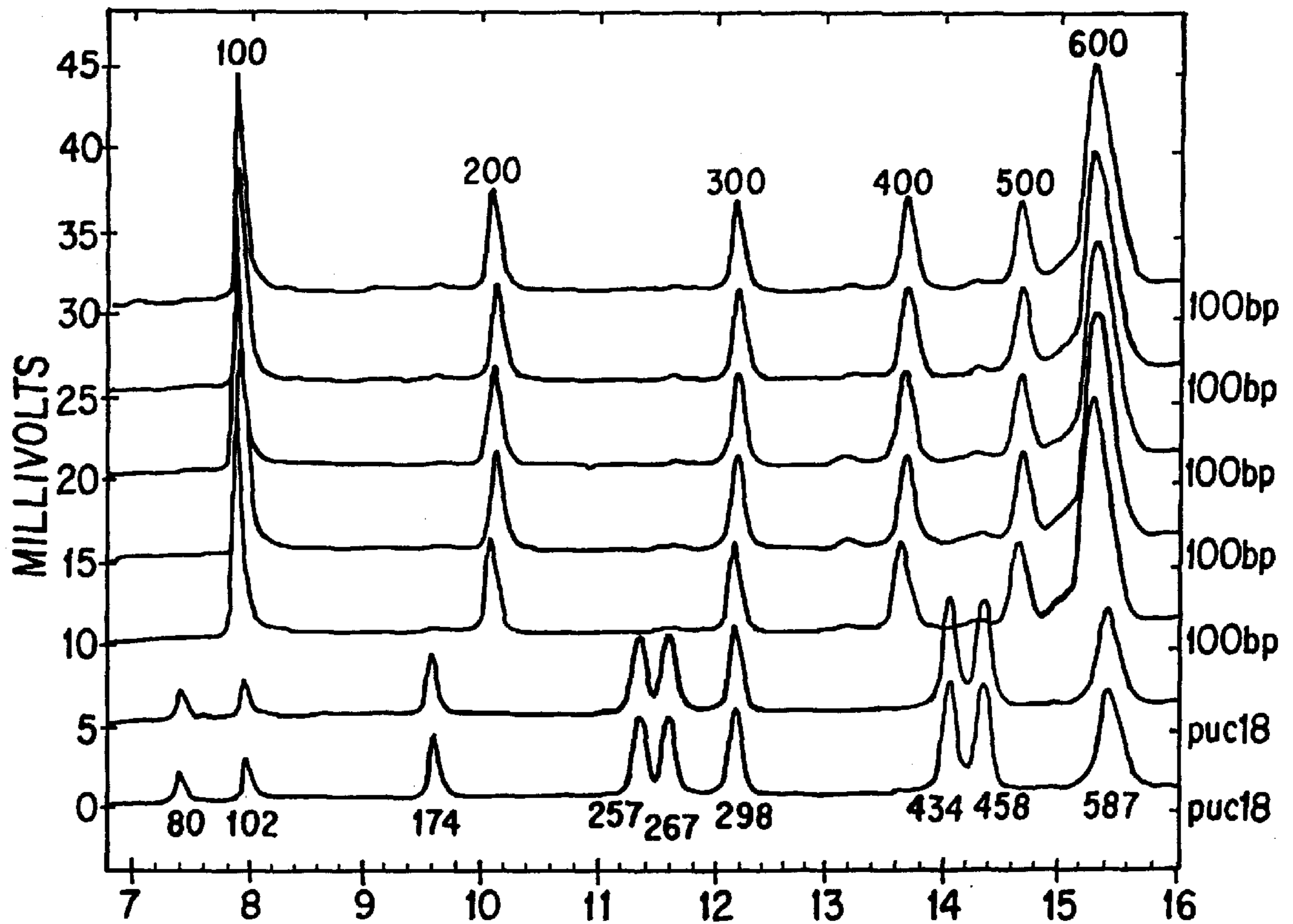
Fig.5 TIME (MINUTES) Chromatograms are offset by 5 millivolts
