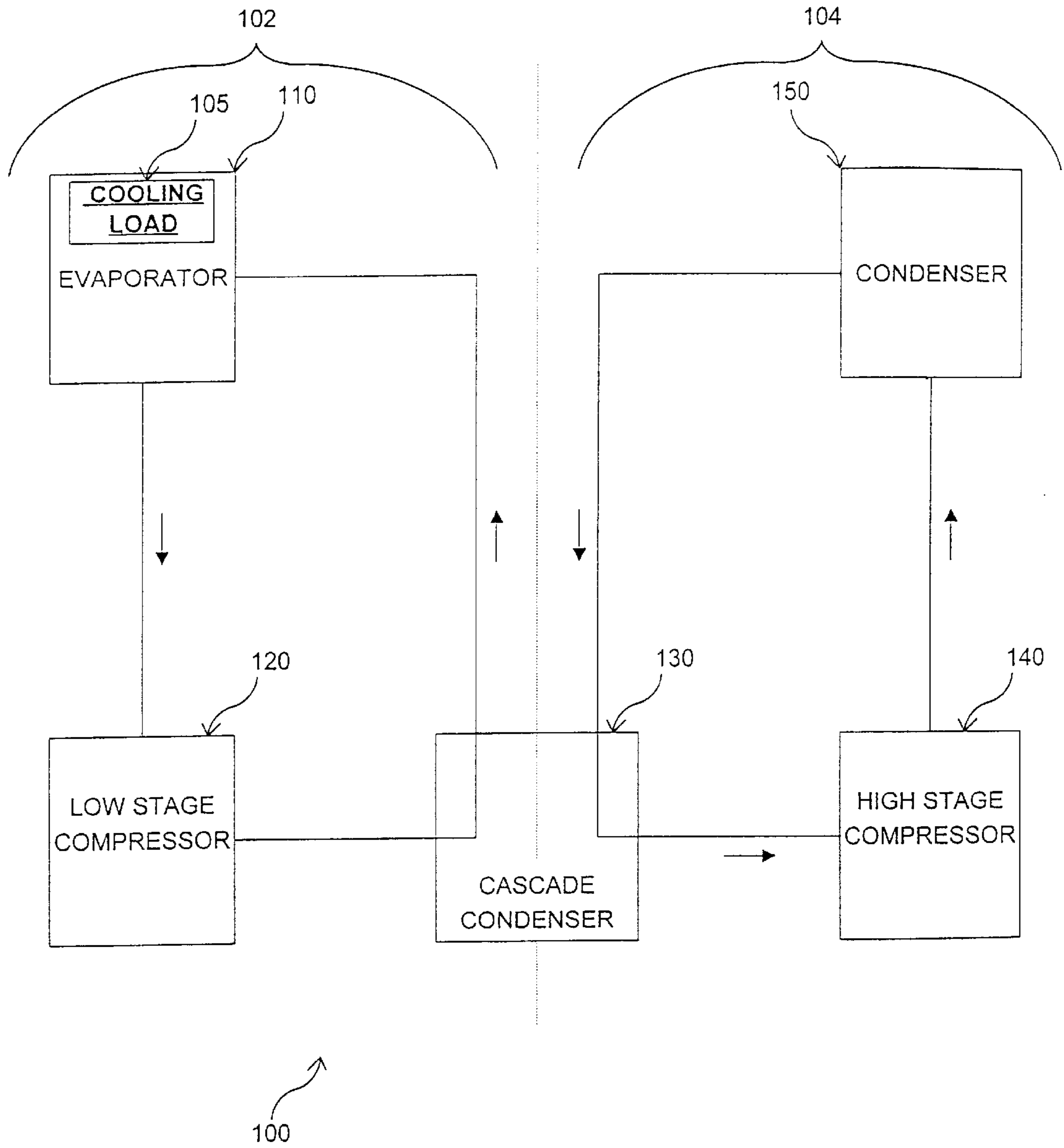
CONVENTIONAL CASCADE SYSTEM
