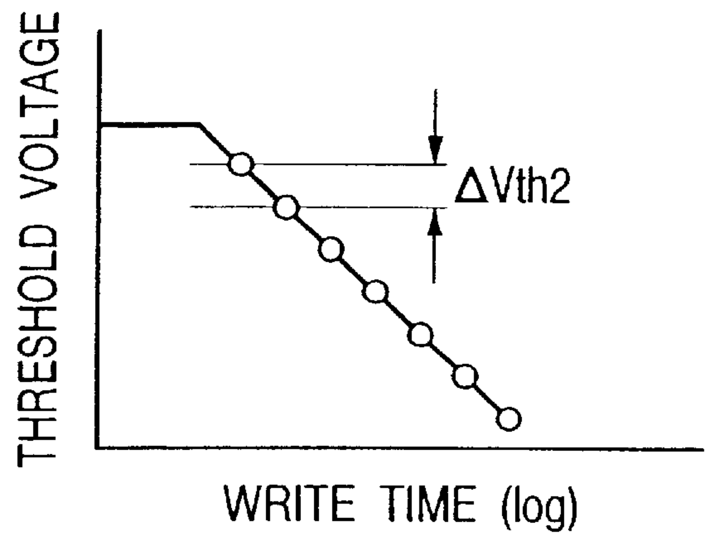
WRITE CHARACTERISTIC
