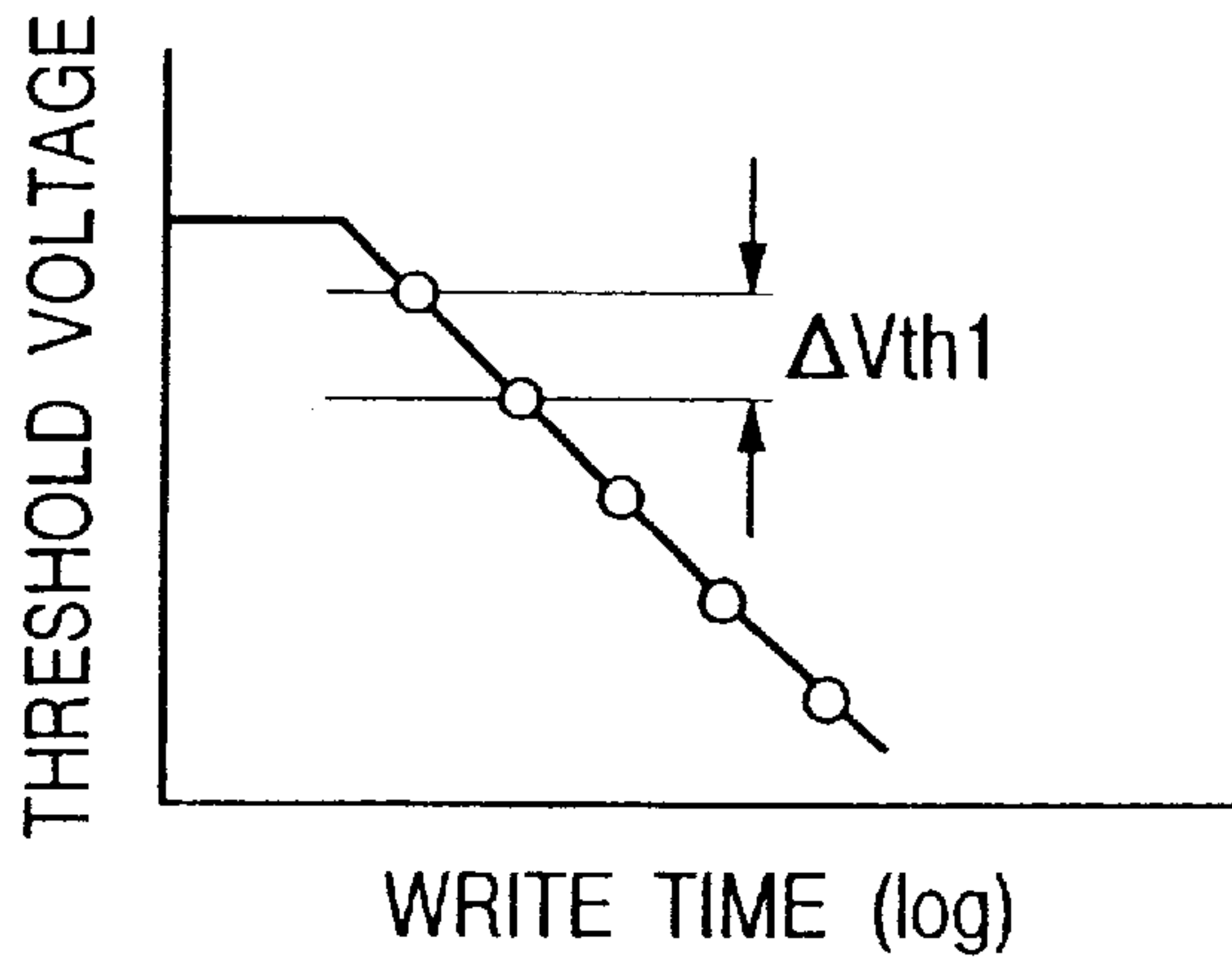
WRITE CHARACTERISTIC
