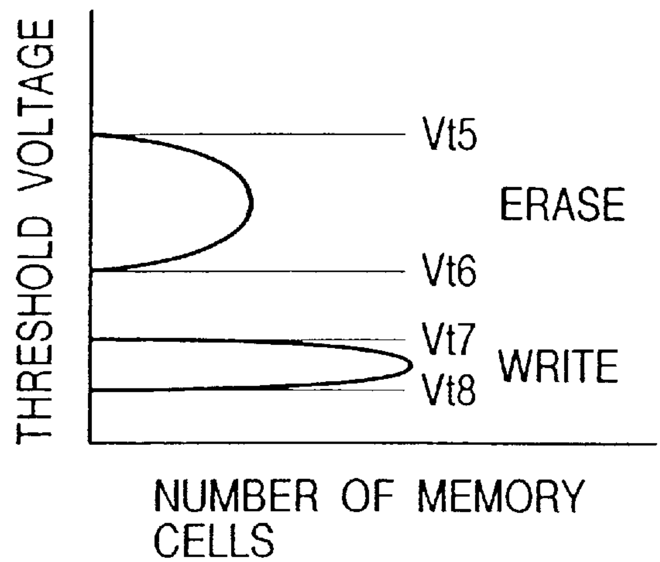
THRESHOLD VOLTAGE DISTRIBUTION
