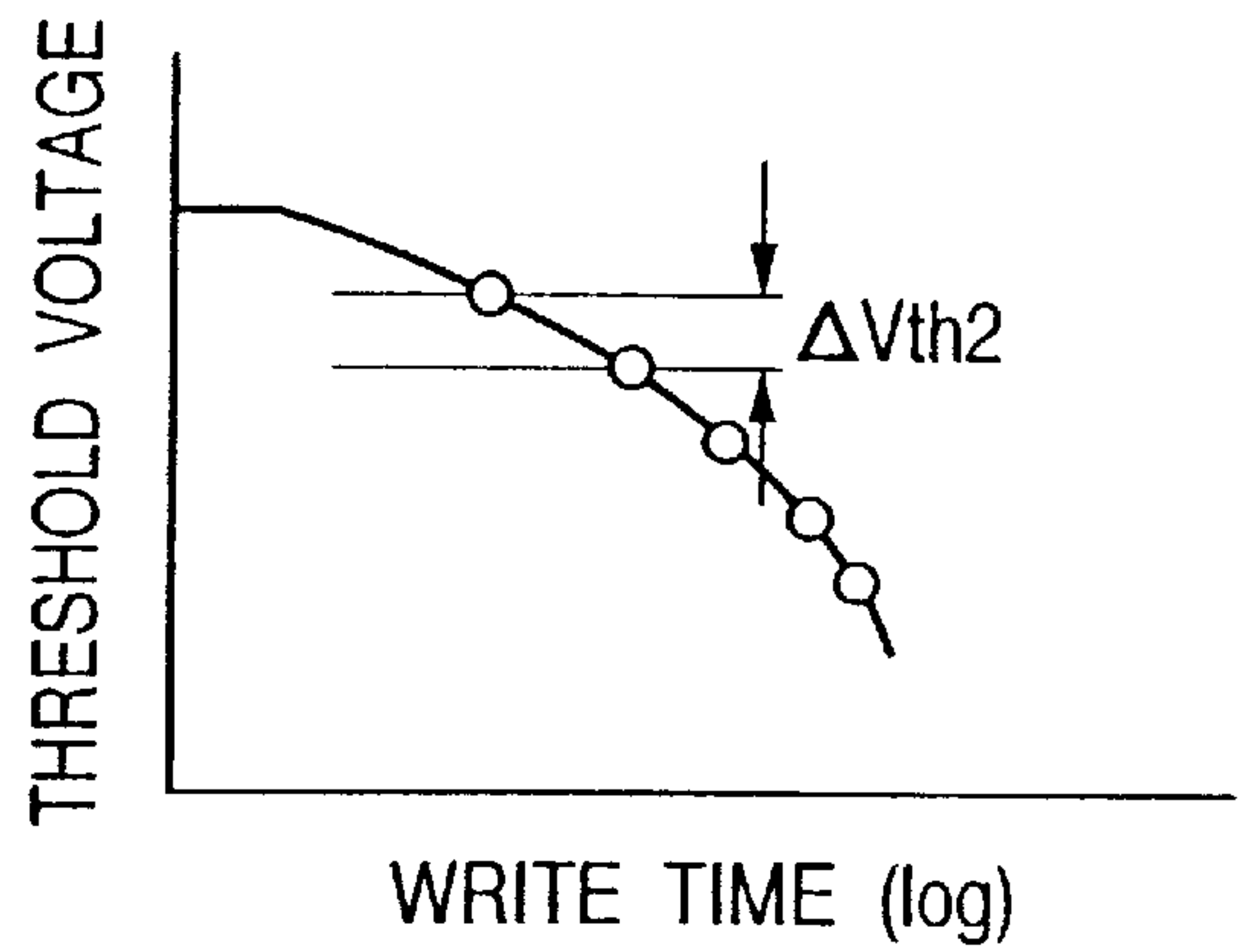
WRITE CHARACTERISTIC
