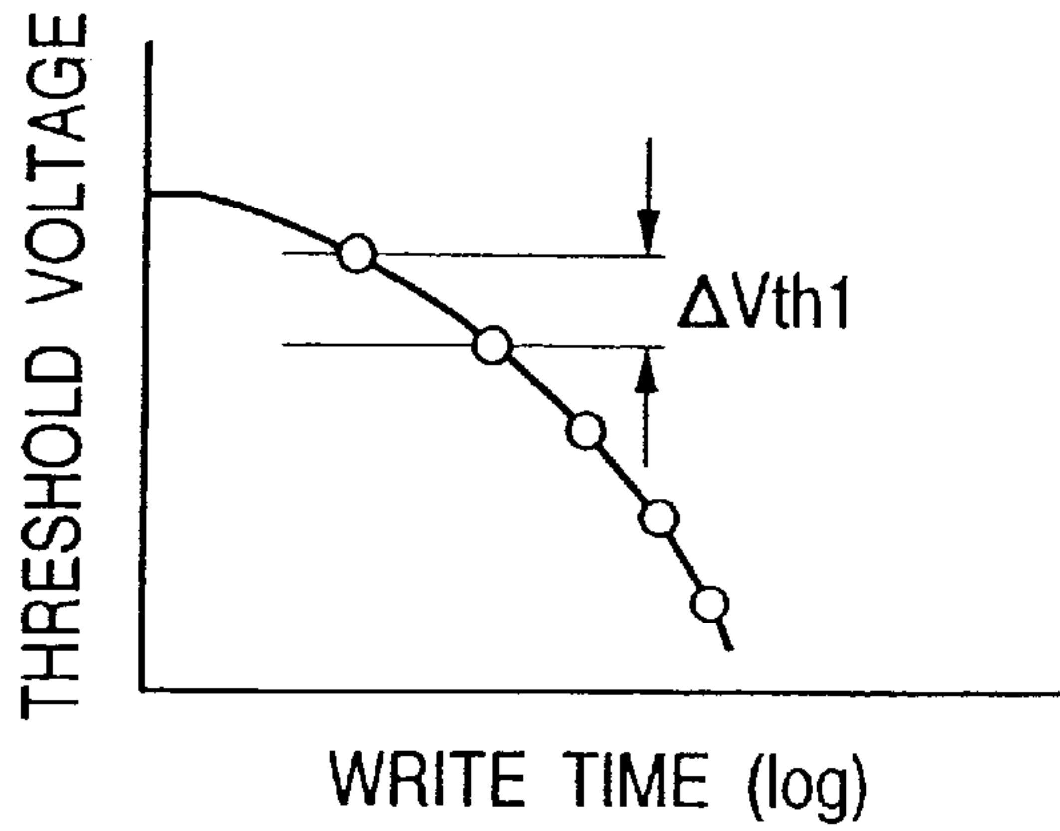
WRITE CHARACTERISTIC
