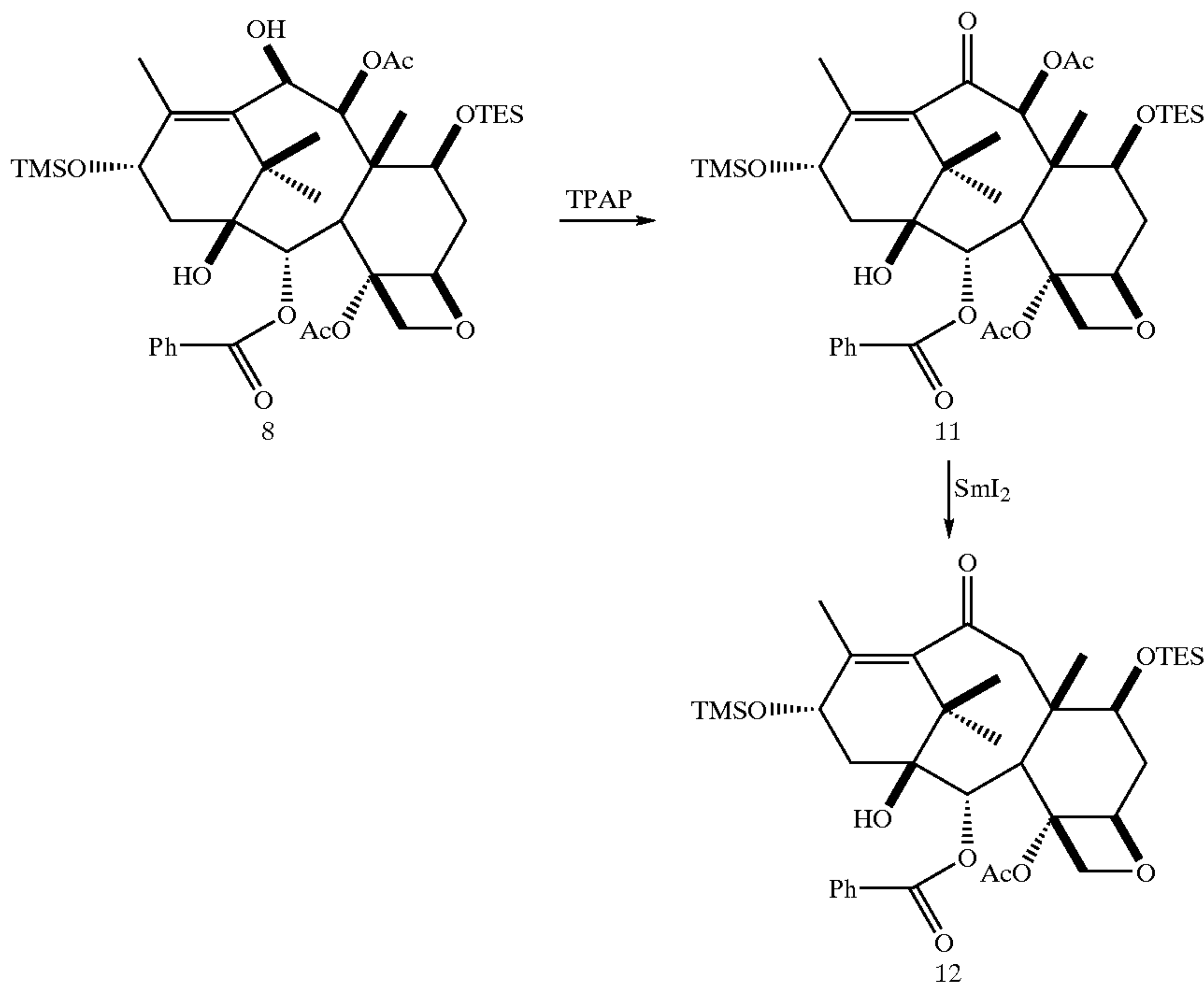
REACTION SCHEME 3
