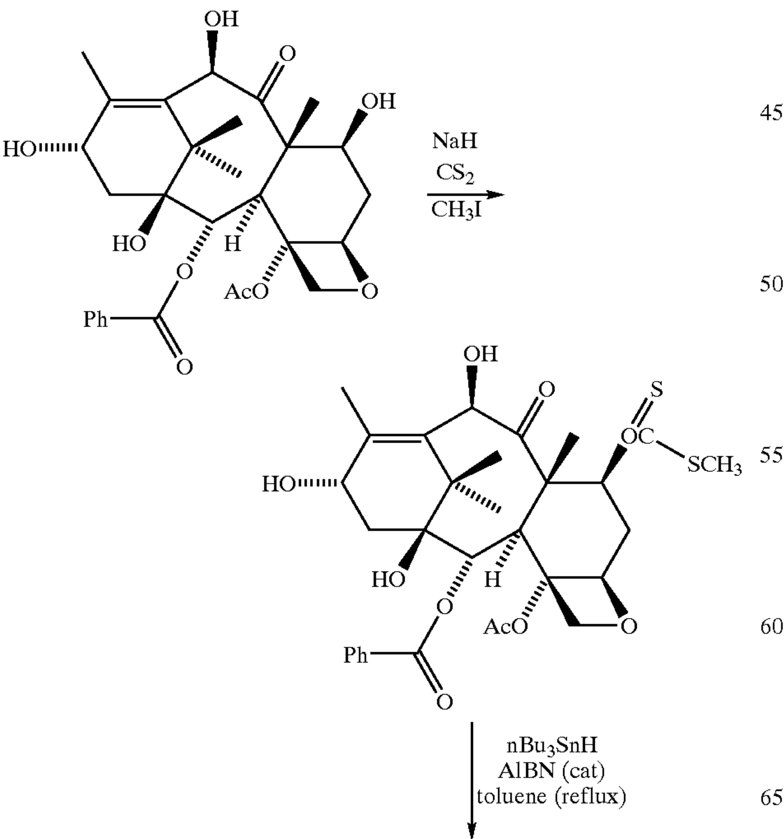
REACTION SCHEME 11
