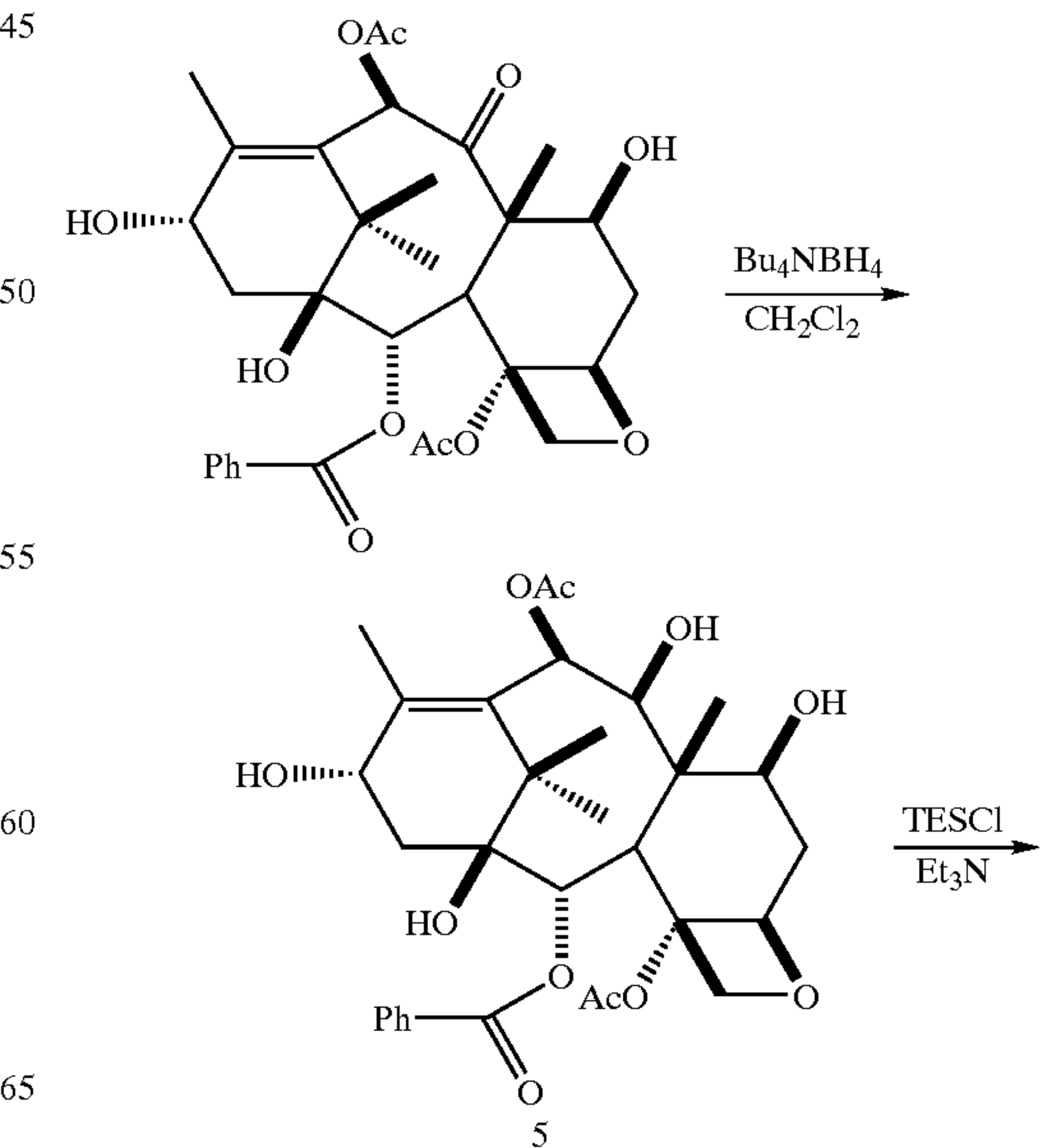
REACTION SCHEME 1
