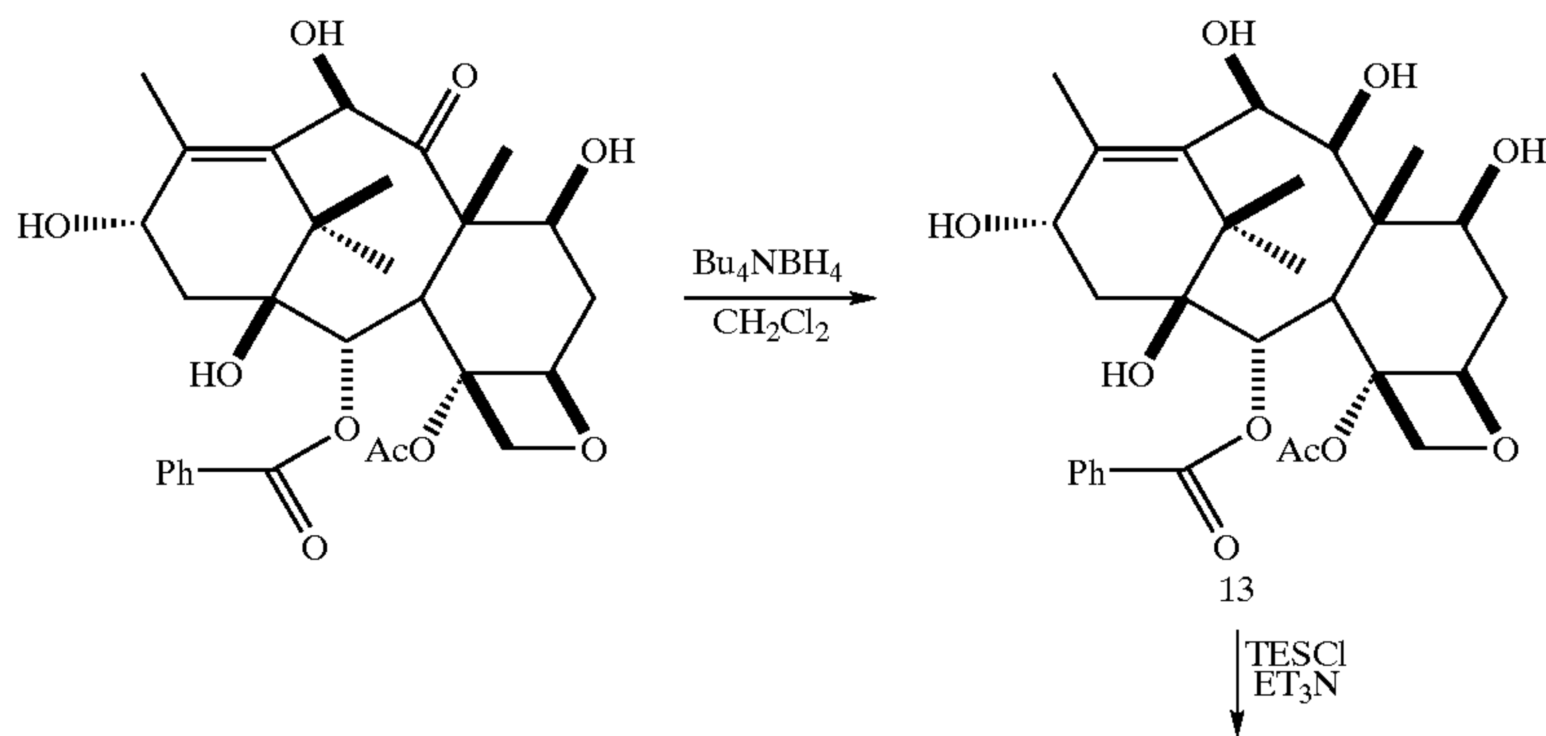
REACTION SCHEME 4
