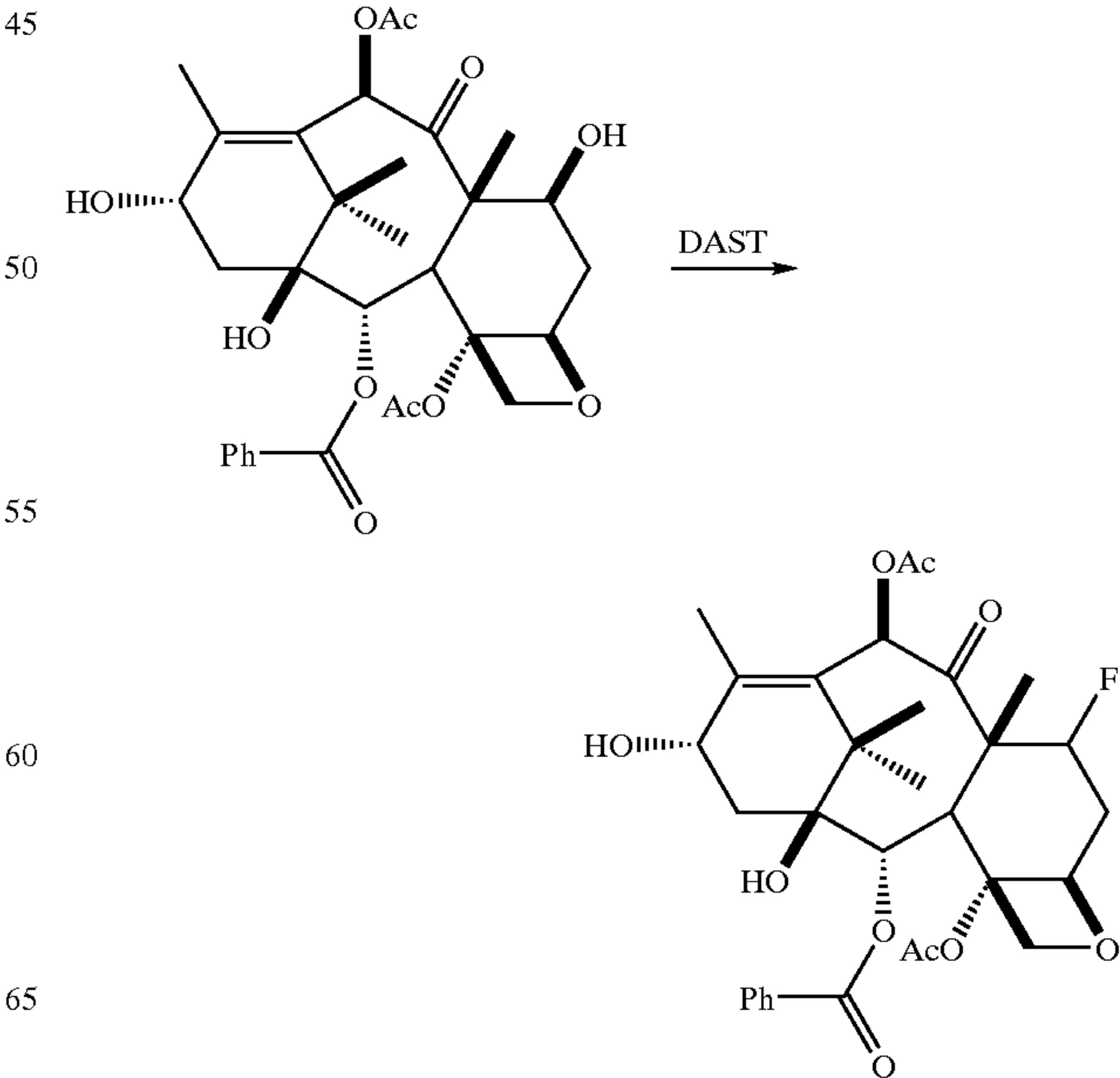
REACTION SCHEME 12
