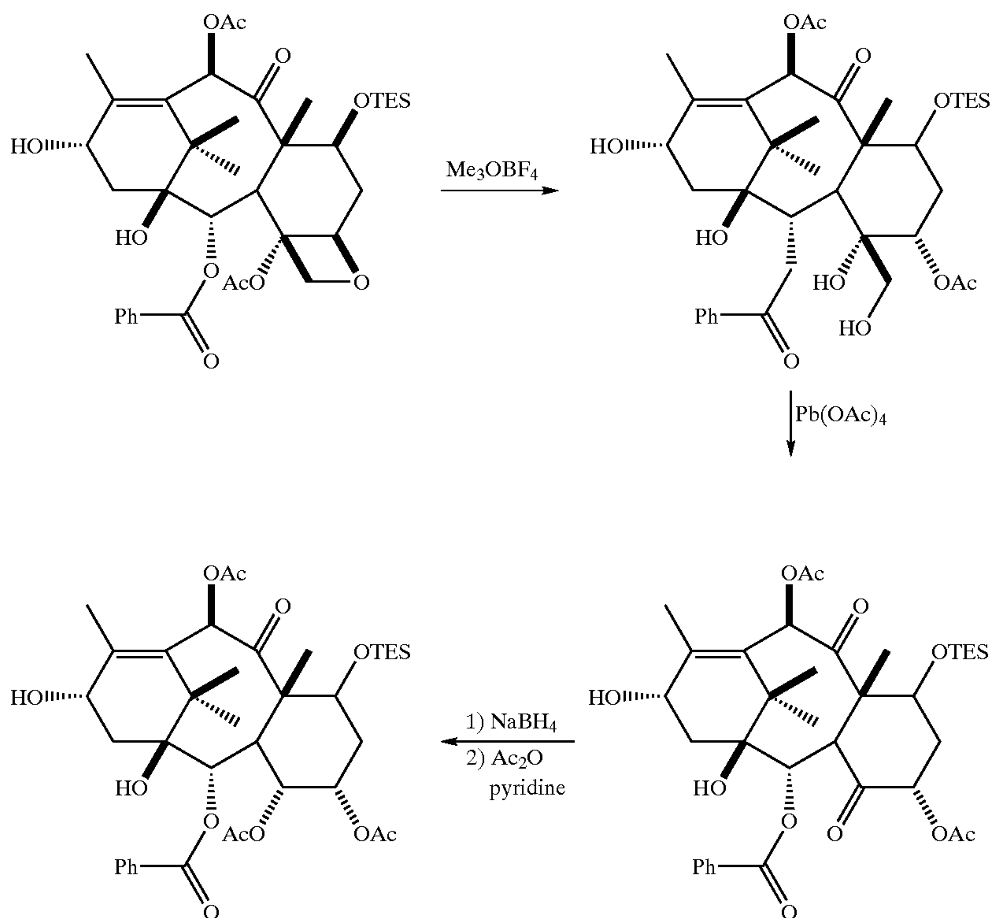
REACTION SCHEME 13
