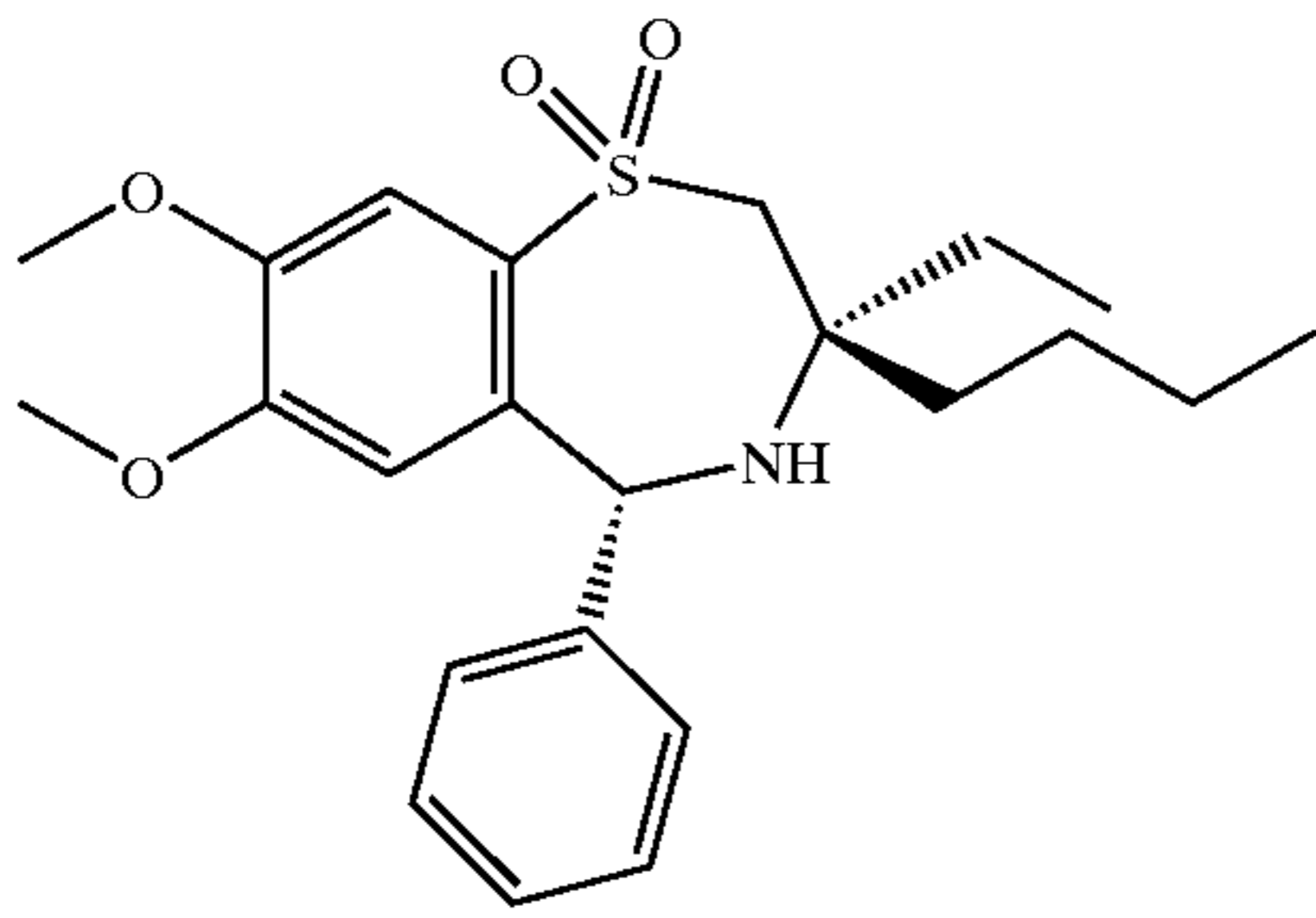
(3R,5R)-3-butyl-3-ethyl-2,3,4,5-tetrahydro-,7,8-dimethoxy-5-phenyl-1,4-benzothiazepine 1,1-dioxide
