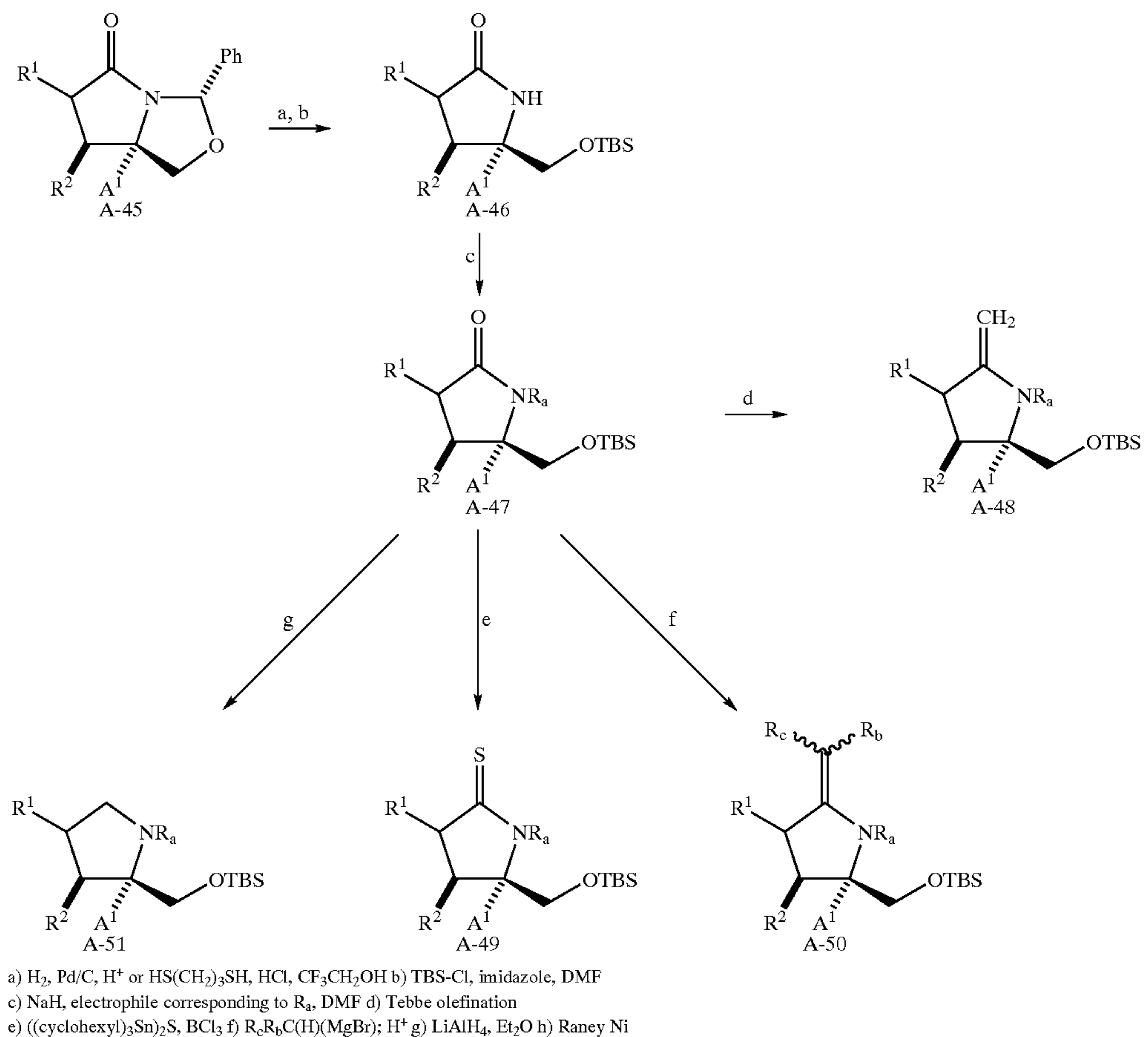
Scheme 8
