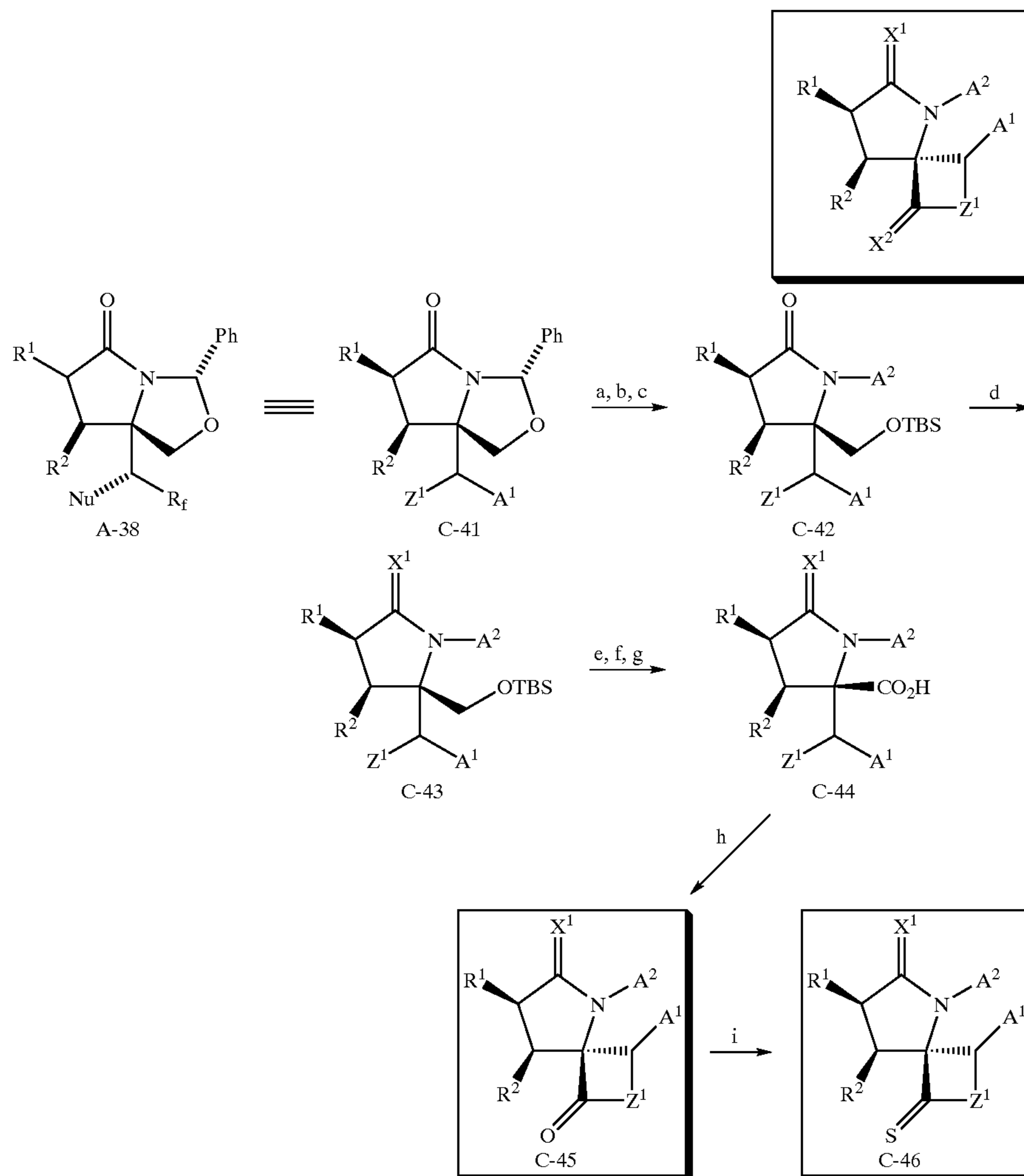
Scheme 25
