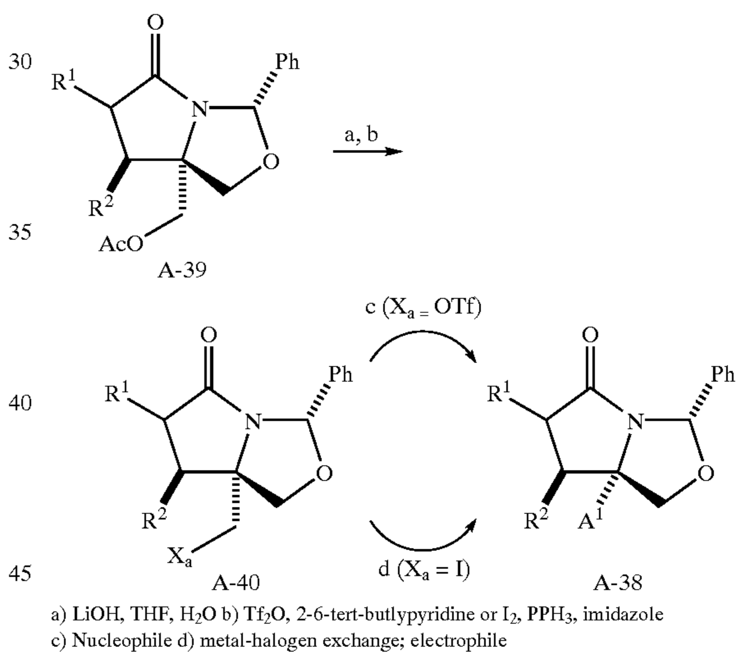
Scheme 6
