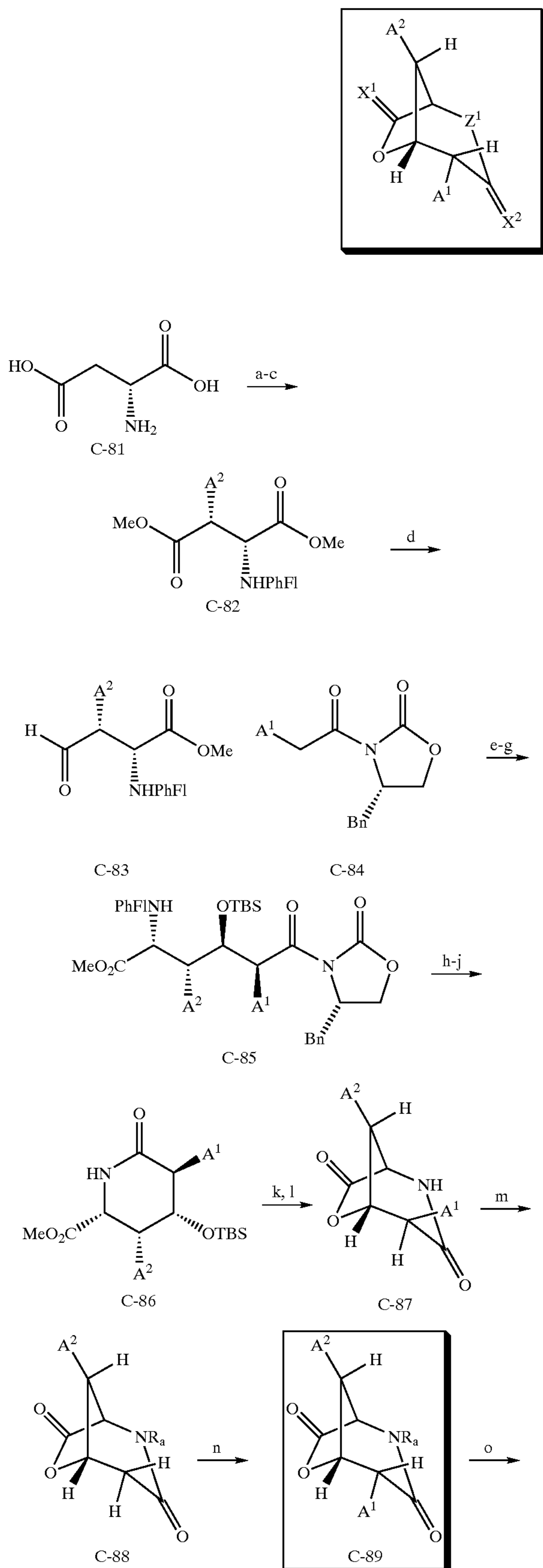
Scheme 29
