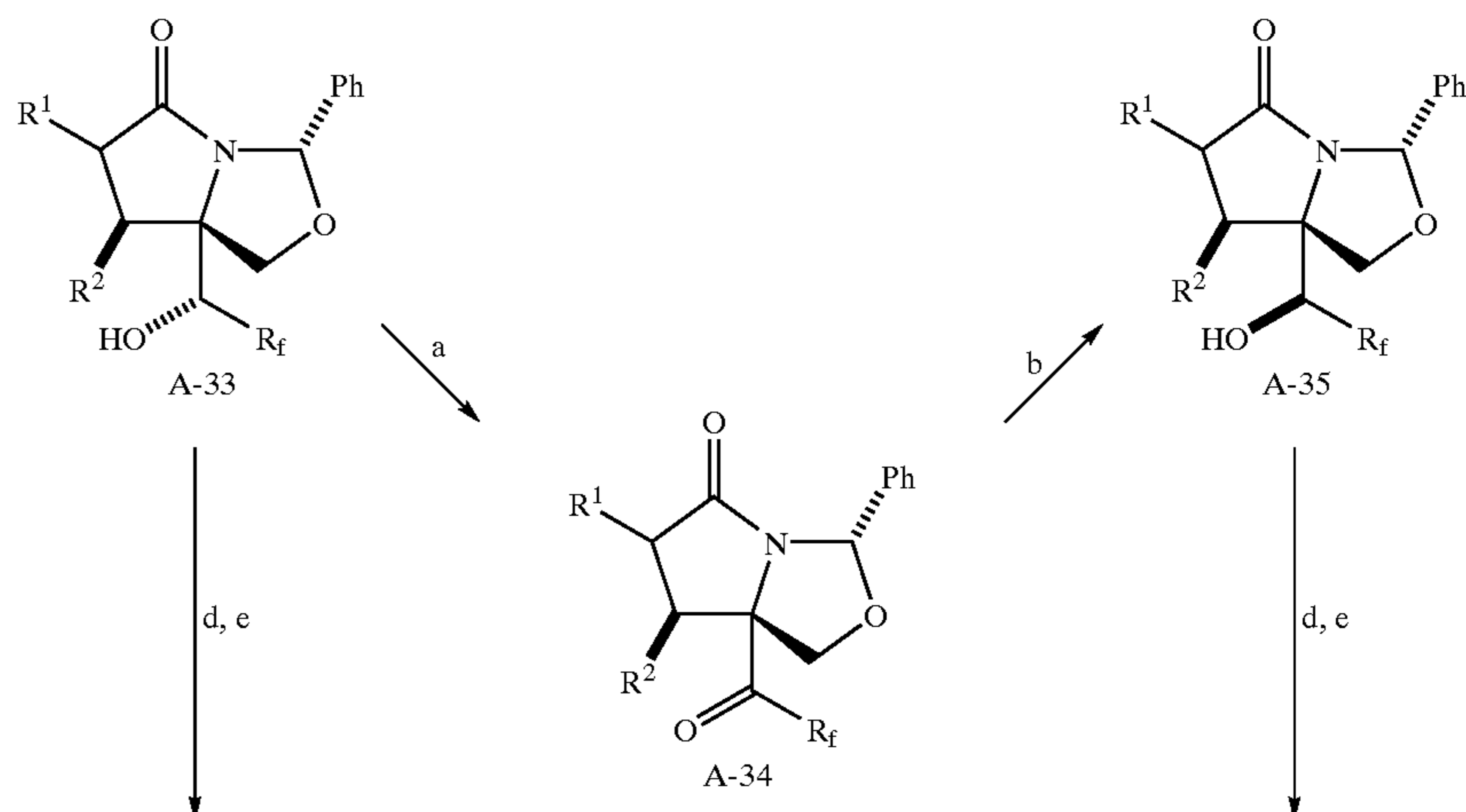
Scheme 5
