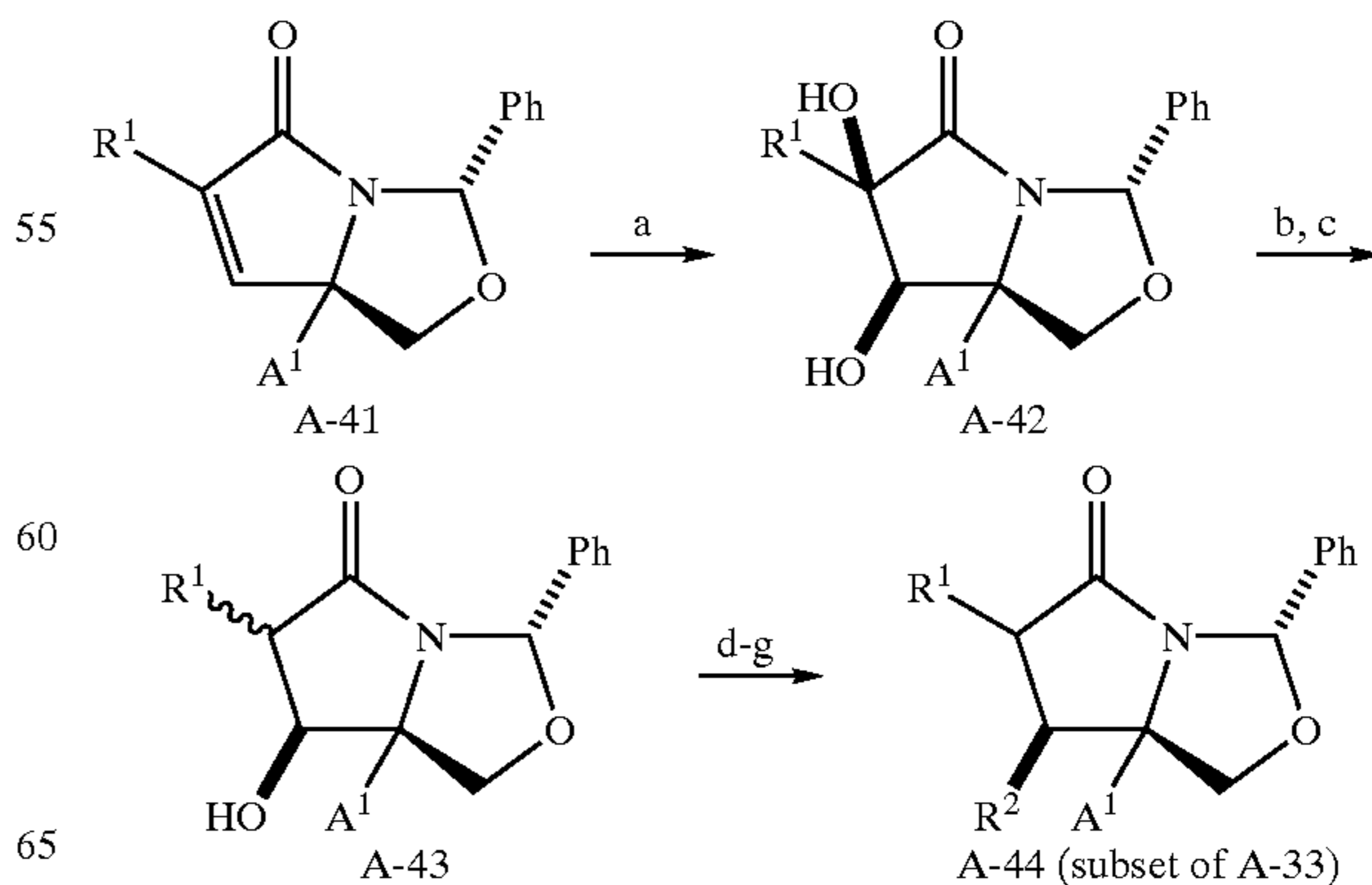
Scheme 7
