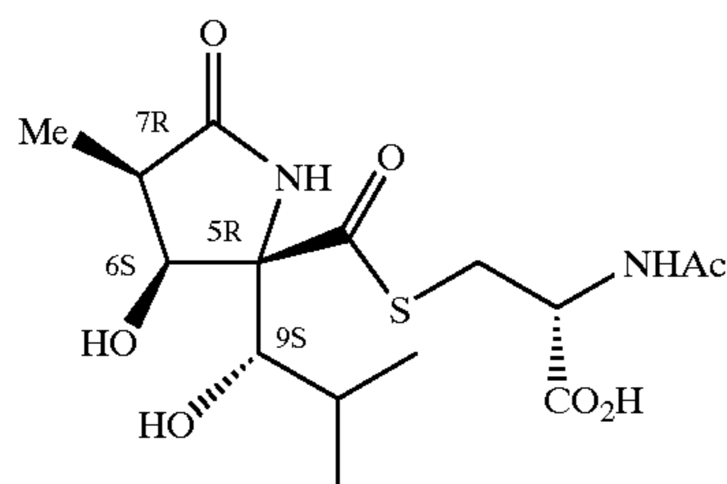
Lactacystin
