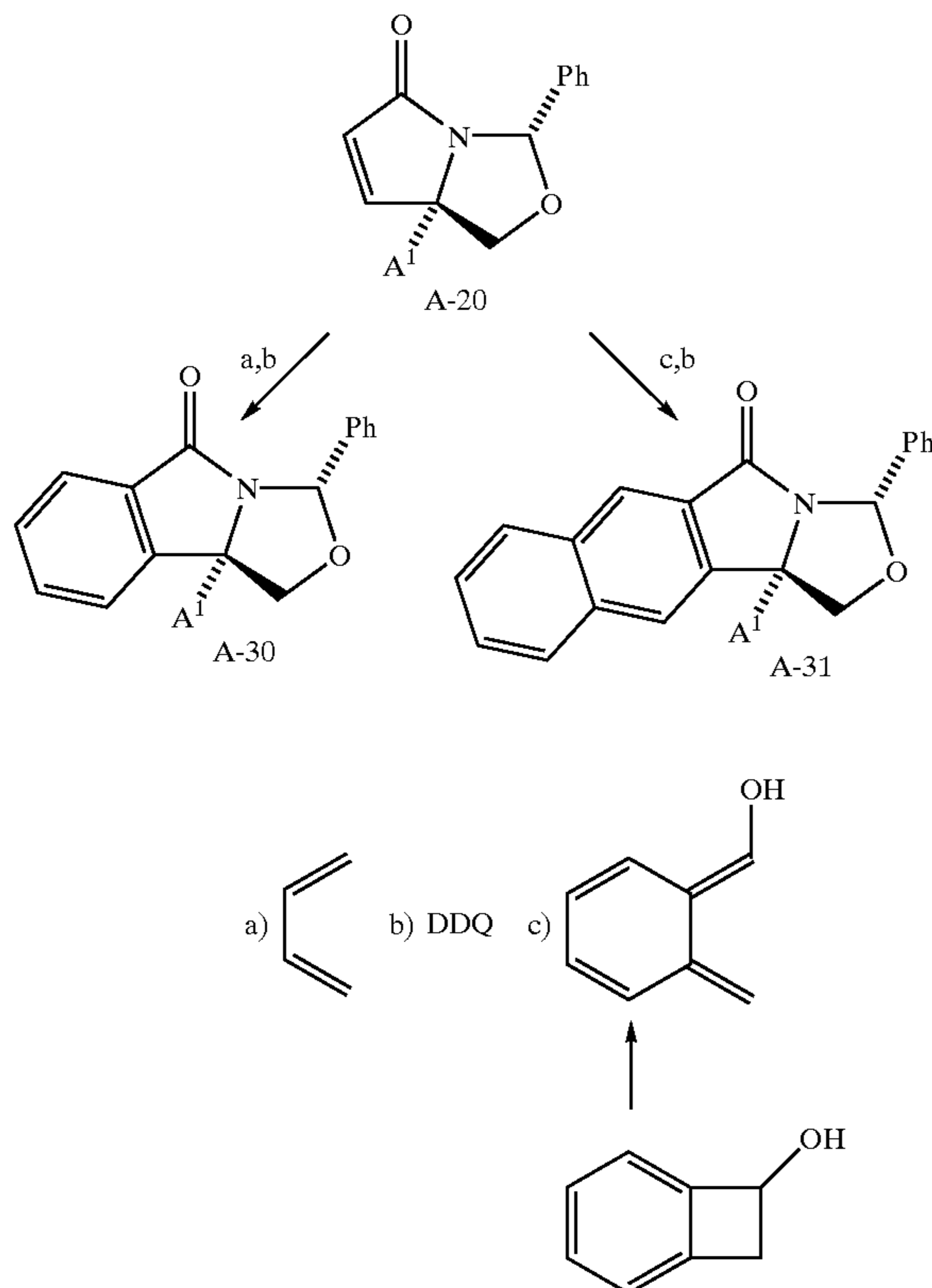
Scheme 4
