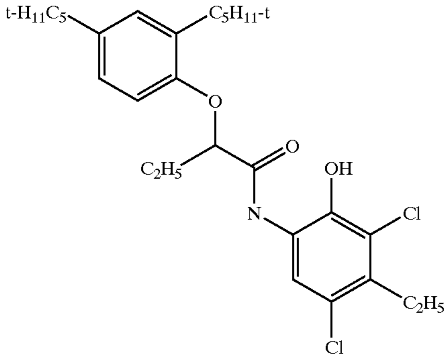
cyan coupler C-1
