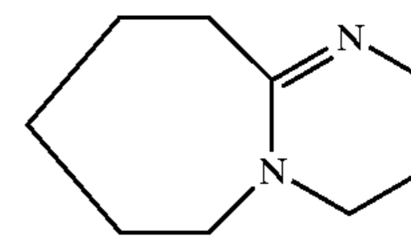
1,8-diazabicyclo[5.4.0]undec-7-ene ("DBU");
