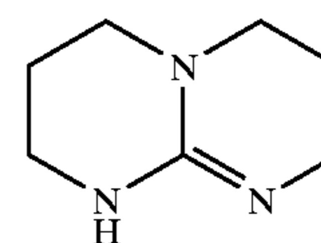
1,5,7-triazabicyclo[4.4.0]dec-5-ene; and
