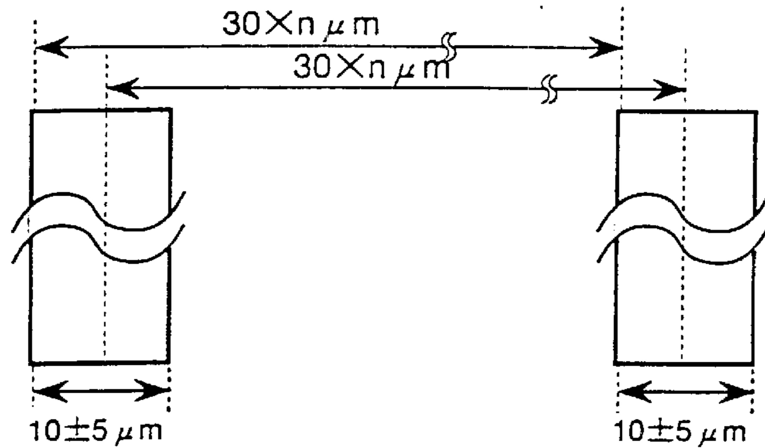
(b) DIMENSIONAL ACCURACY OF SLIT ( at r=22.2\text{mm} )
