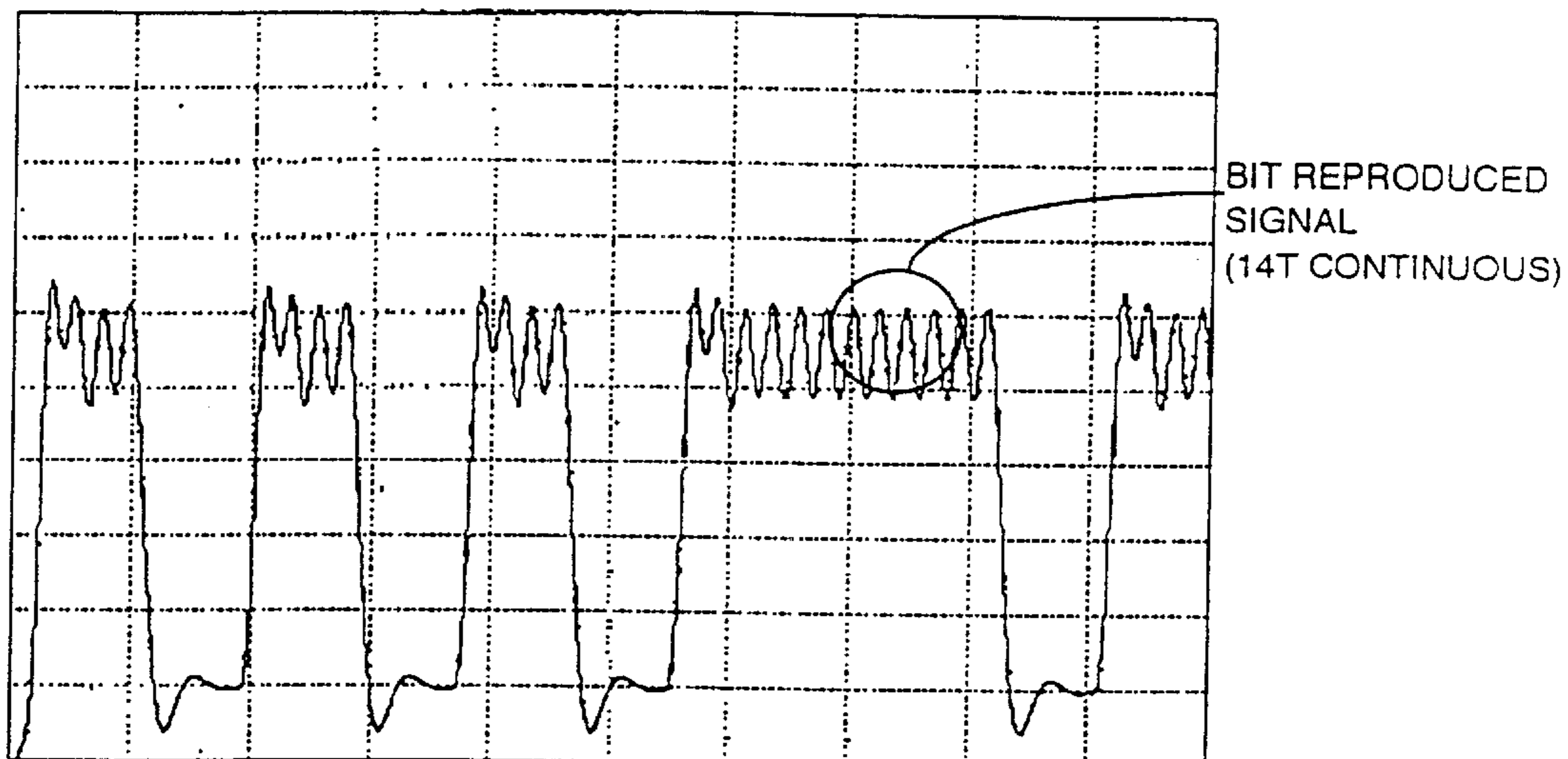
(b) SIMULATOR WAVEFORM AFTER LPF : I_{14L} = I_S = 0.1
