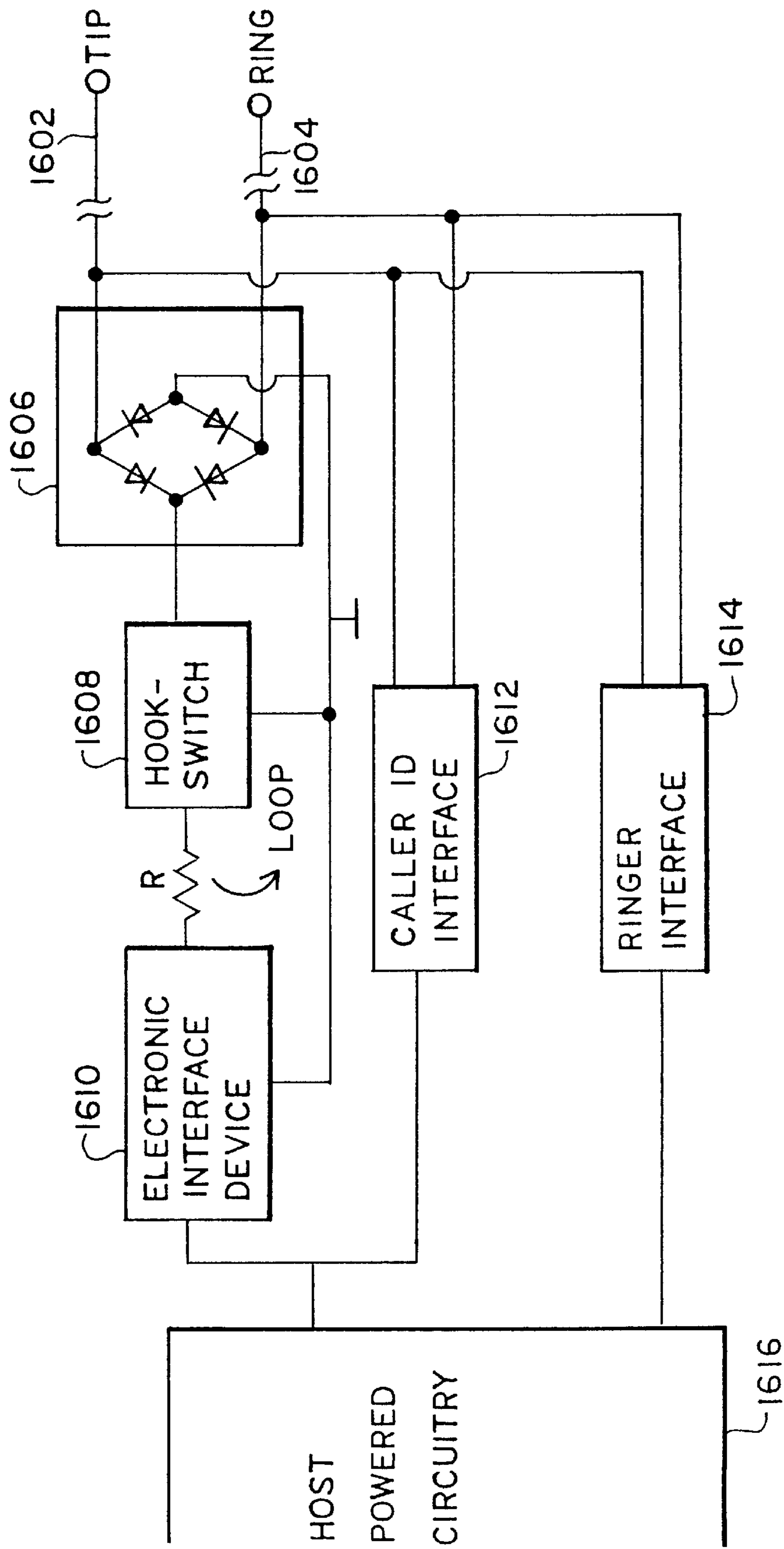
FIG. 16 (PRIOR ART)
