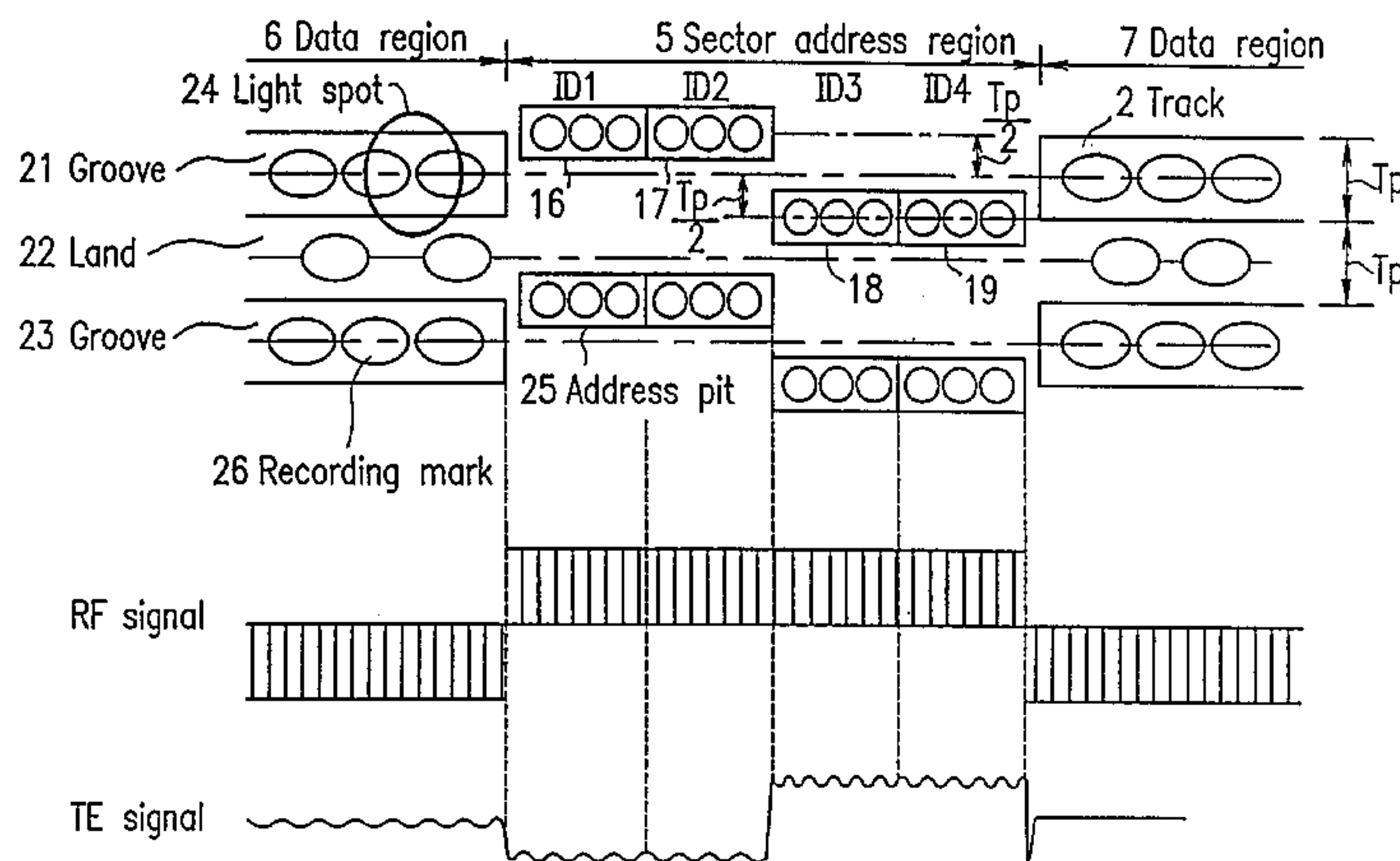
RF signal and TE signal in sector address region
