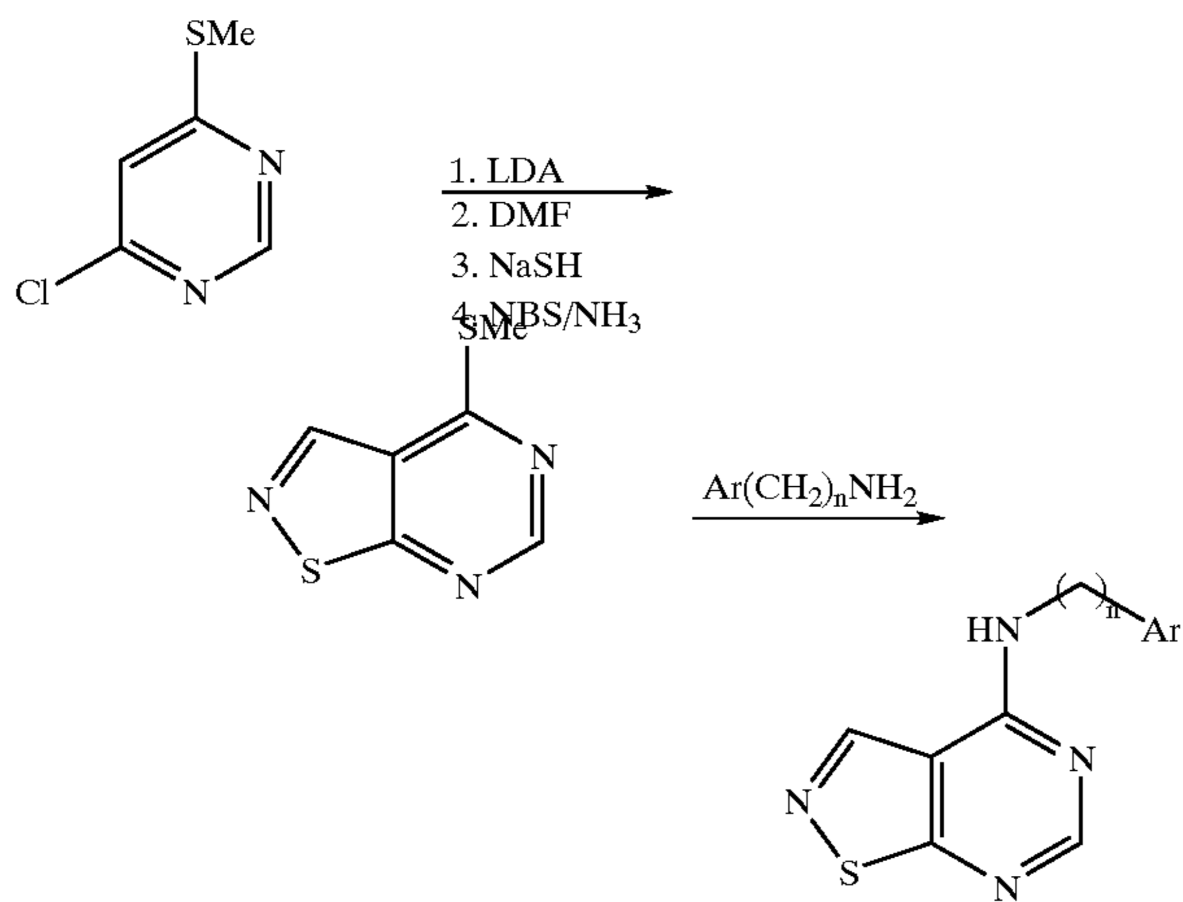
Scheme 30 Synthesis of Preferred Group 48: [5,4-d] ring fusion.
