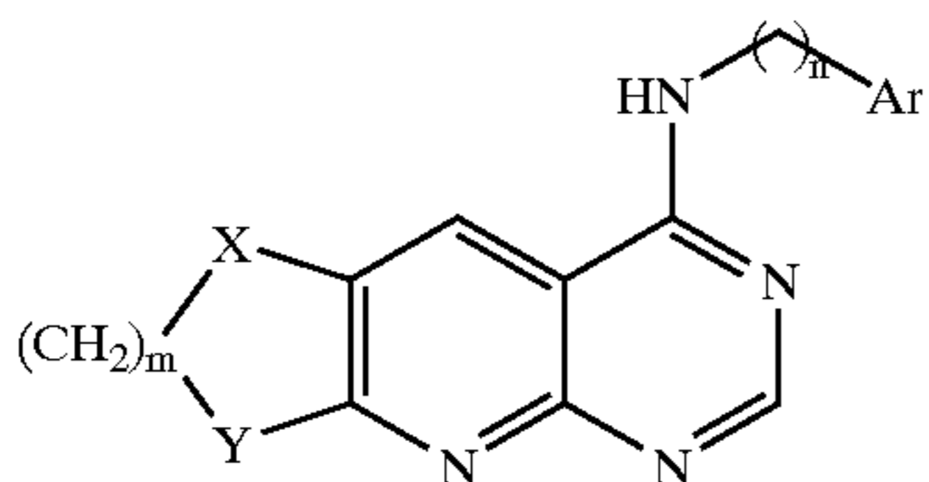
Scheme 14 Preferred Group 32.
