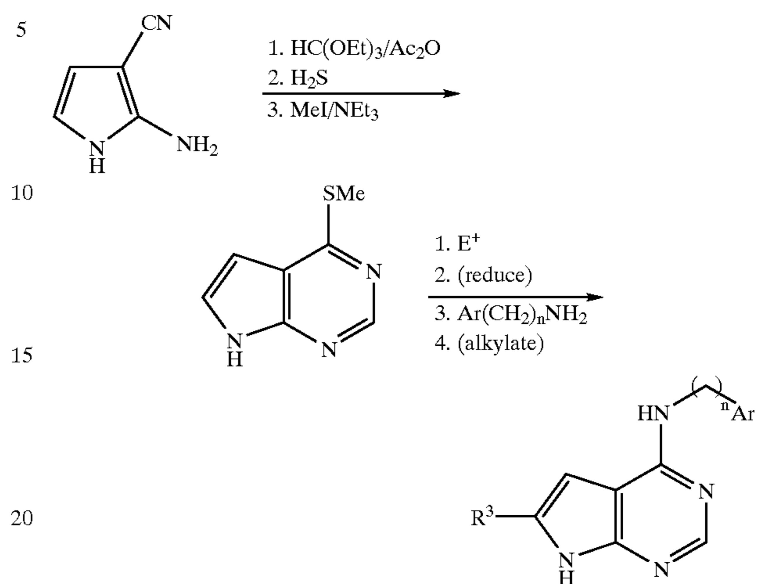
Scheme 21 Synthesis of Preferred Group 43: [2,3-d] ring fusion.
