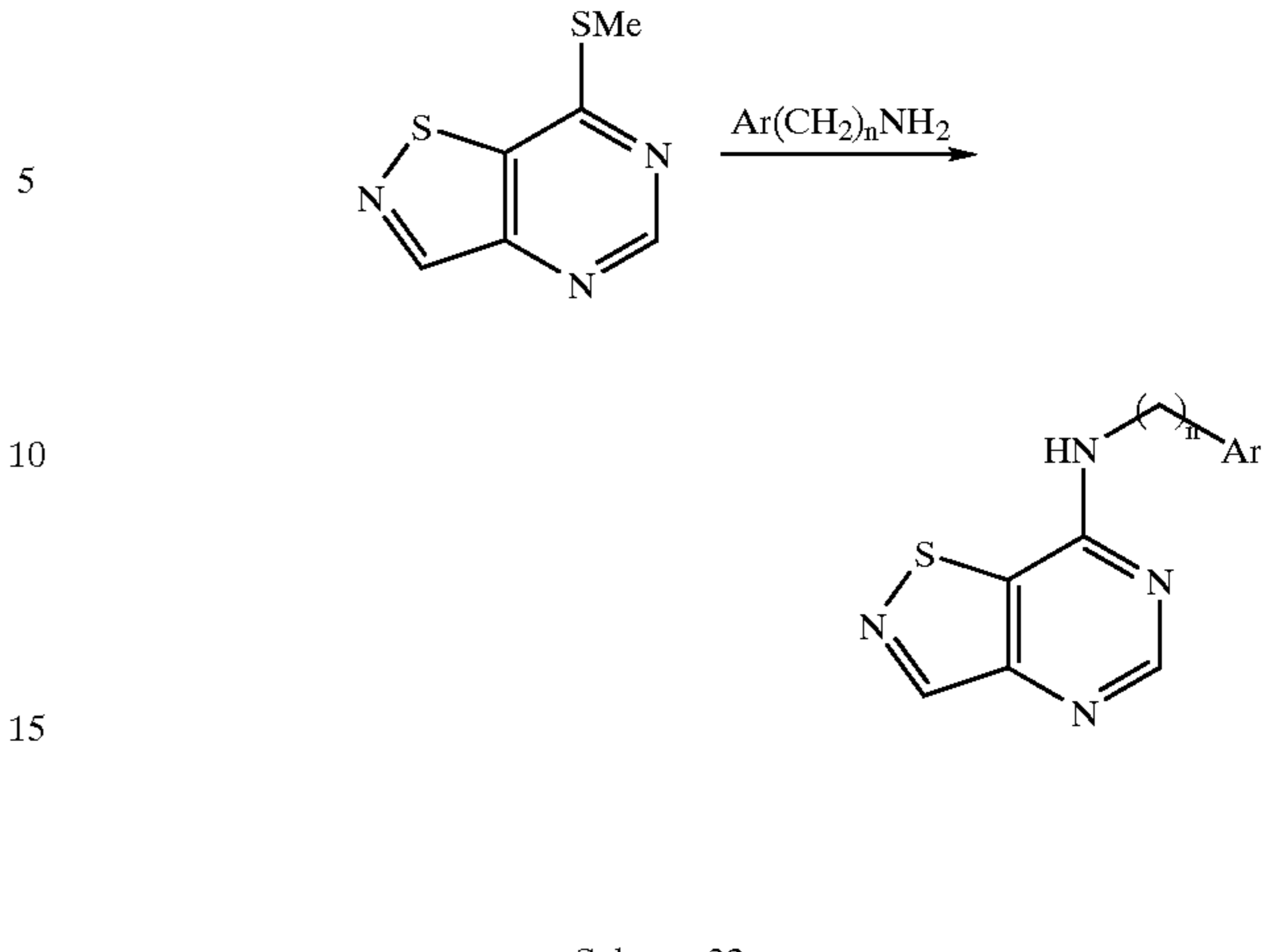
Scheme 32 Synthesis of Preferred Group 49: [3,4-d] ring fusion.
