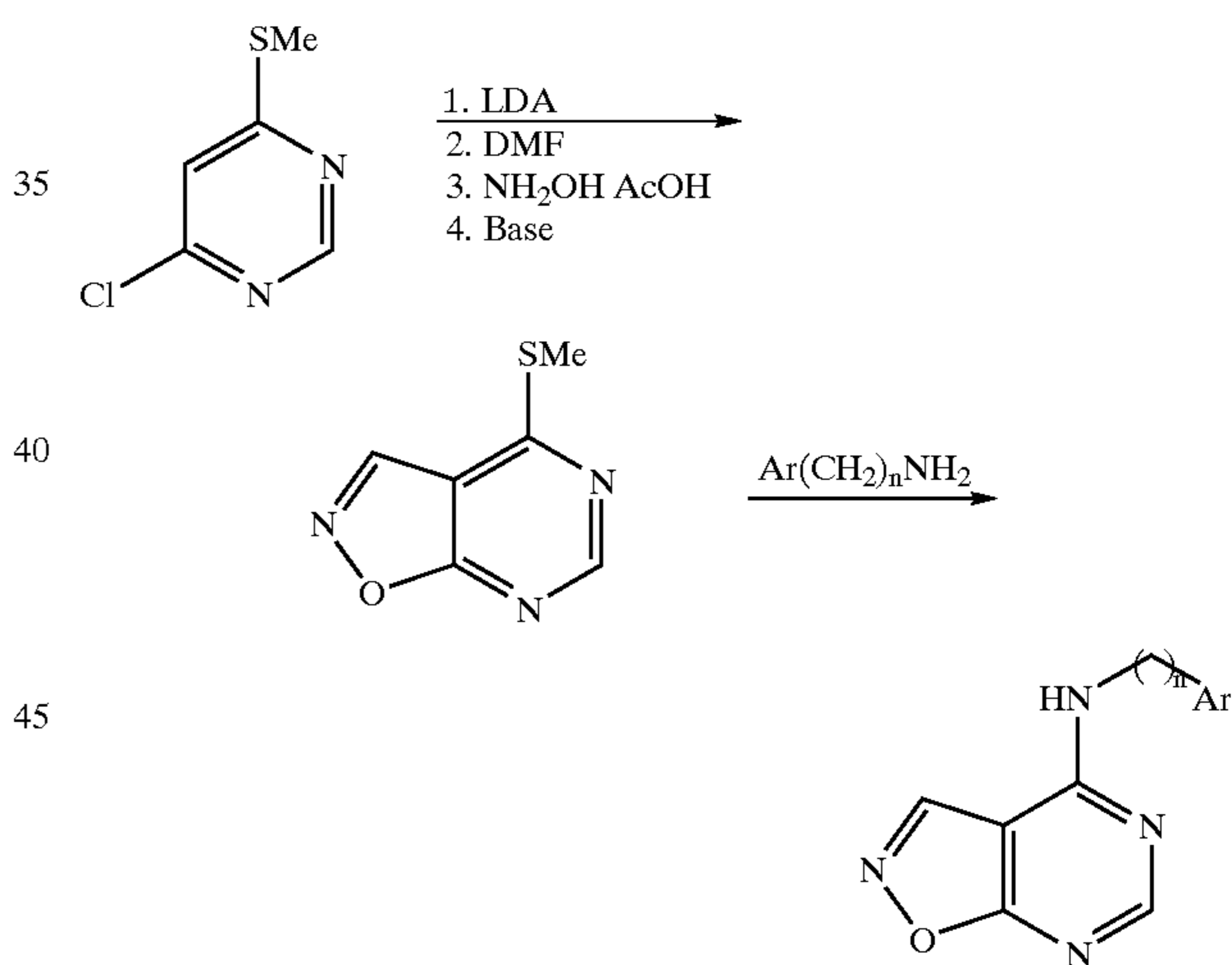
Scheme 28 Synthesis of Preferred Group 47: [5,4-d] ring fusion.
