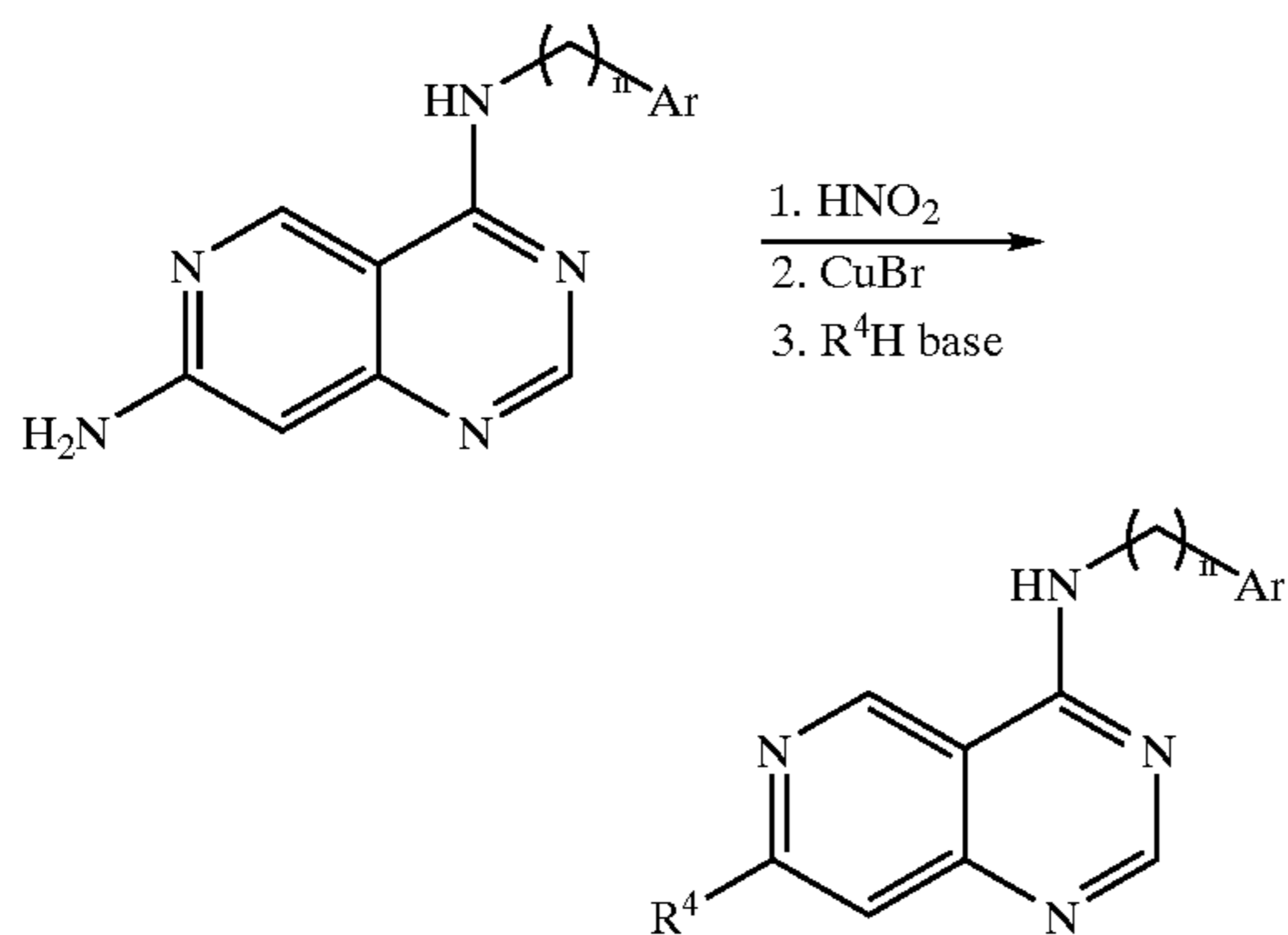
Scheme 8 Synthesis of Preferred Groups 17-21.
