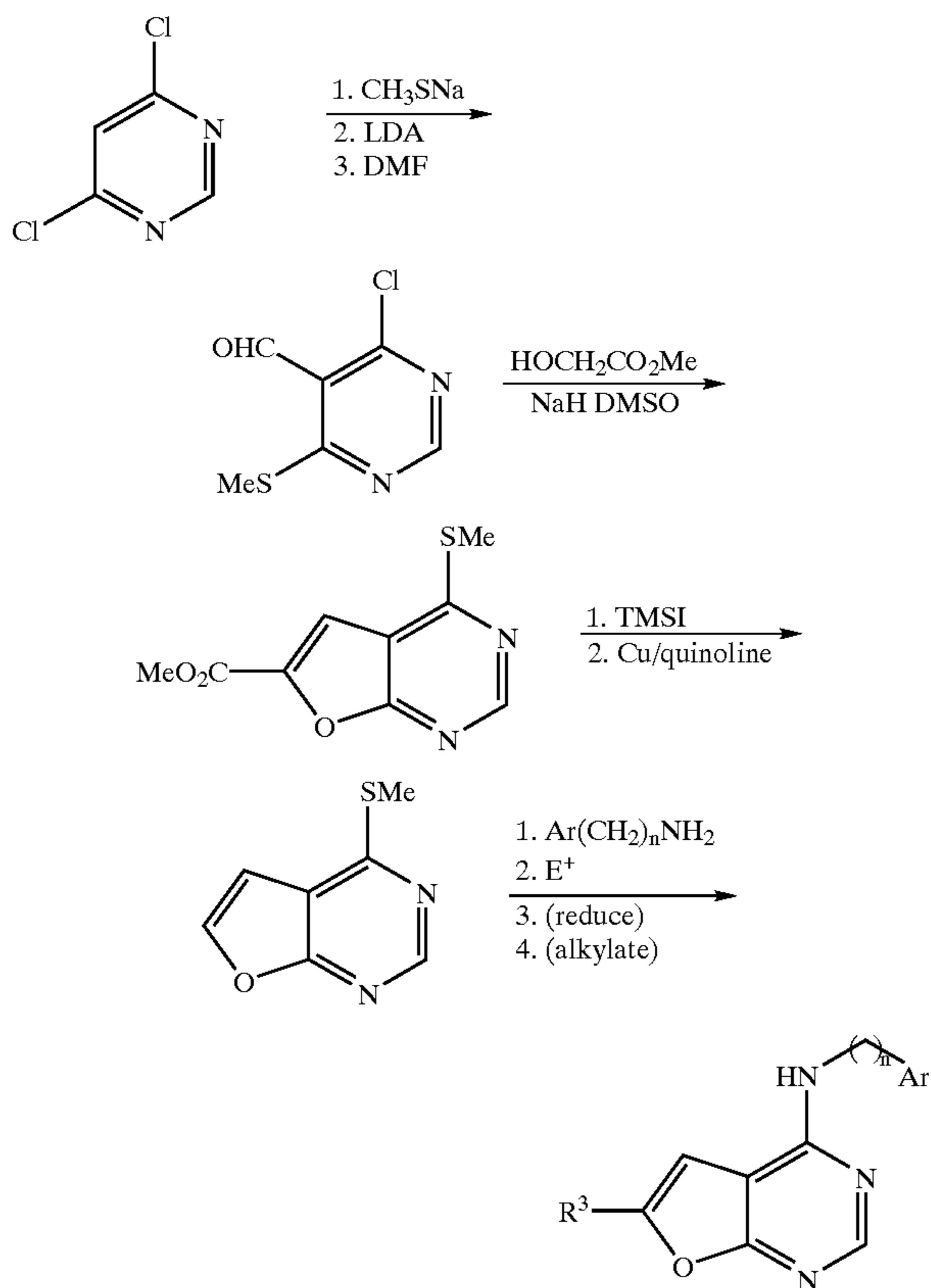
Scheme 20 Synthesis of Preferred Group 42: [2,3-d] ring fusion
