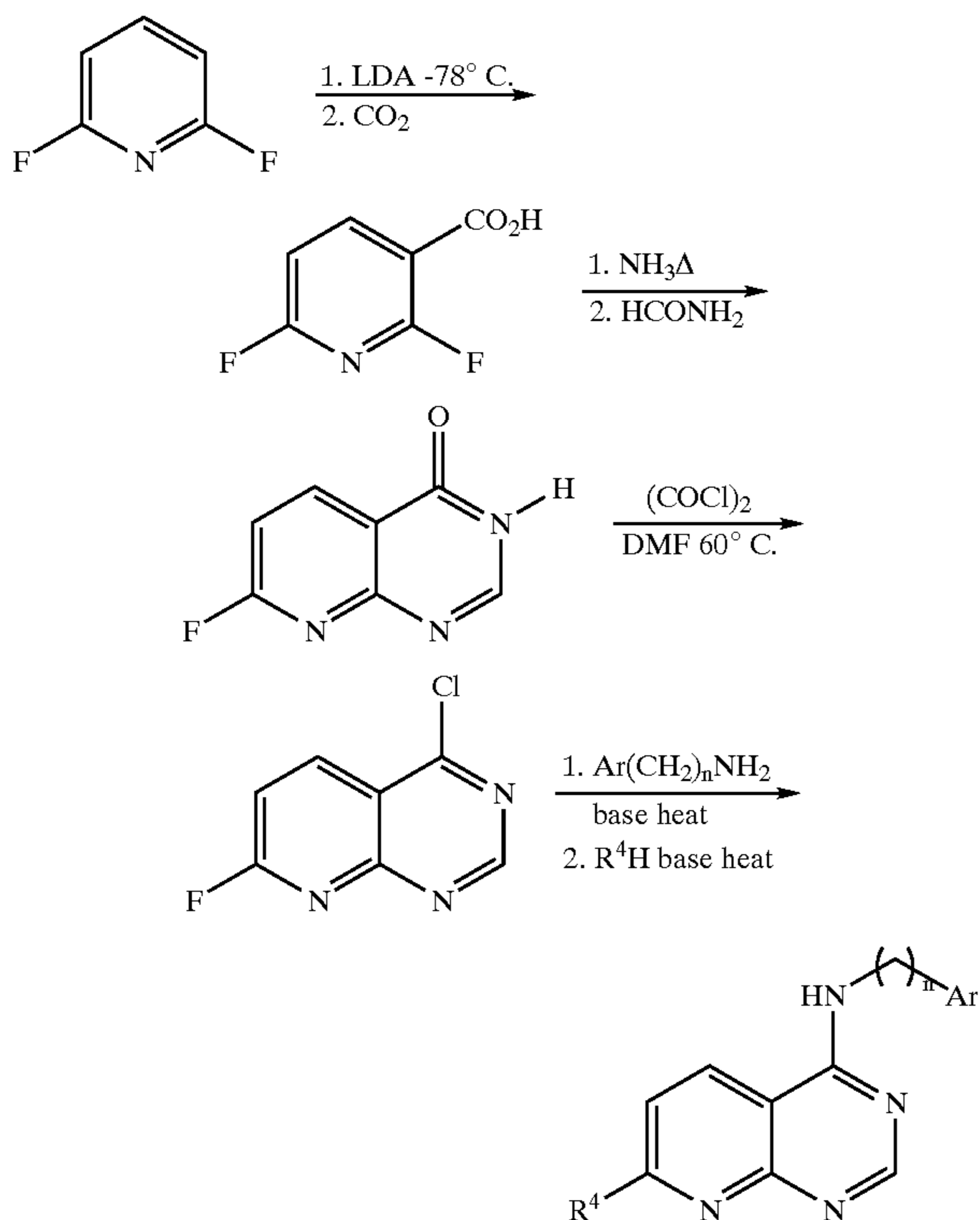
Scheme 10 Synthesis of Preferred Groups 22–26: R 3 = H.
