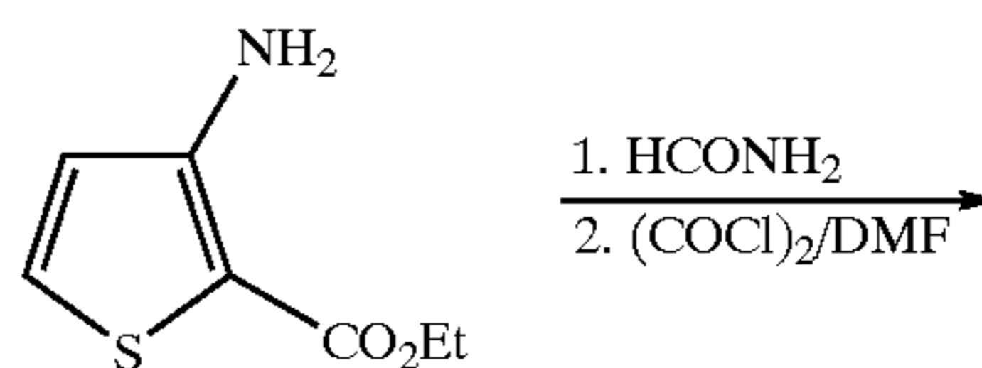
Scheme 17 Synthesis of Preferred Group 41: [3,2-d] ring fusion
