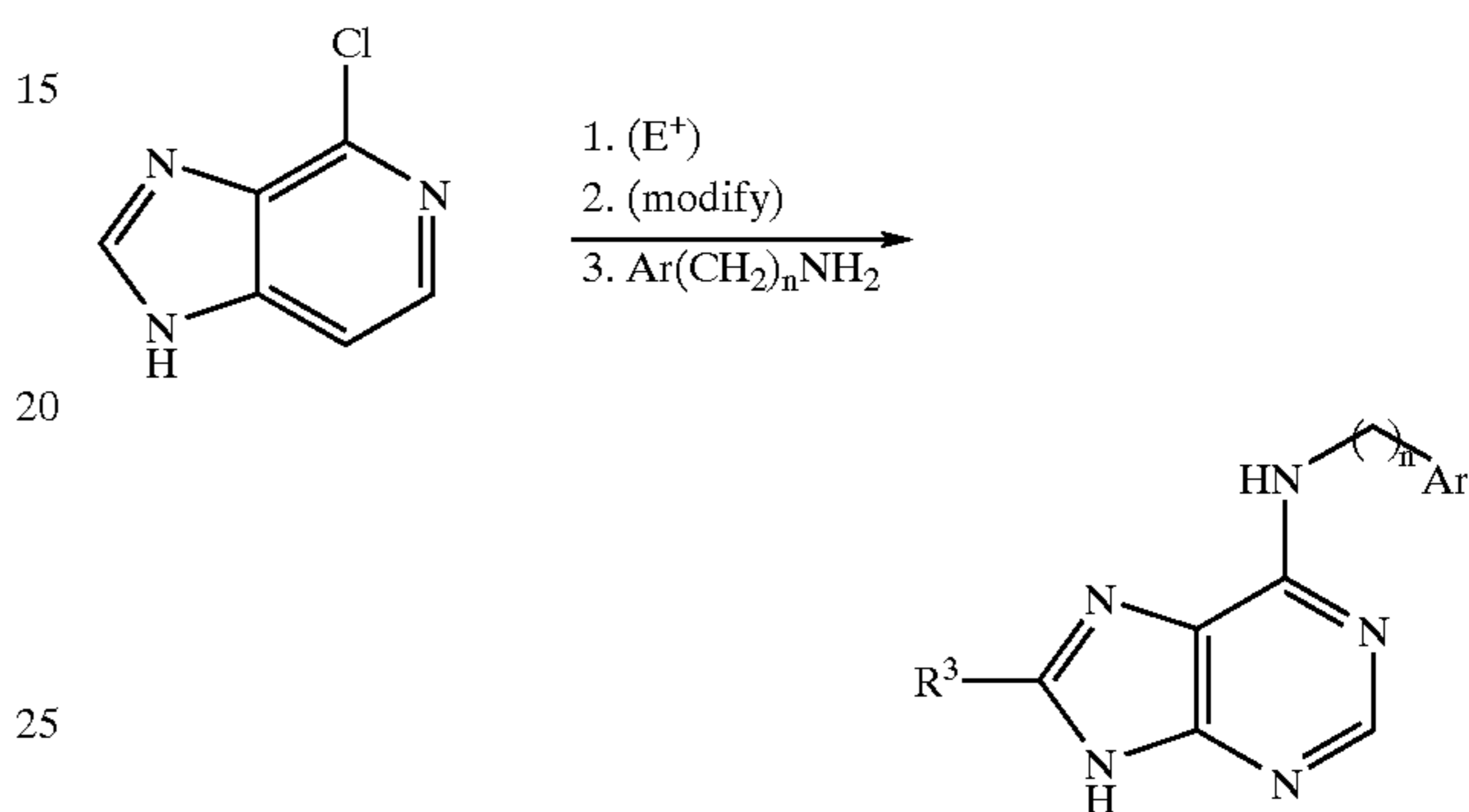
Scheme 27 Synthesis of Preferred Group 46.
