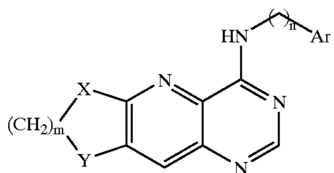
Scheme 6 Preferred Group 11.
