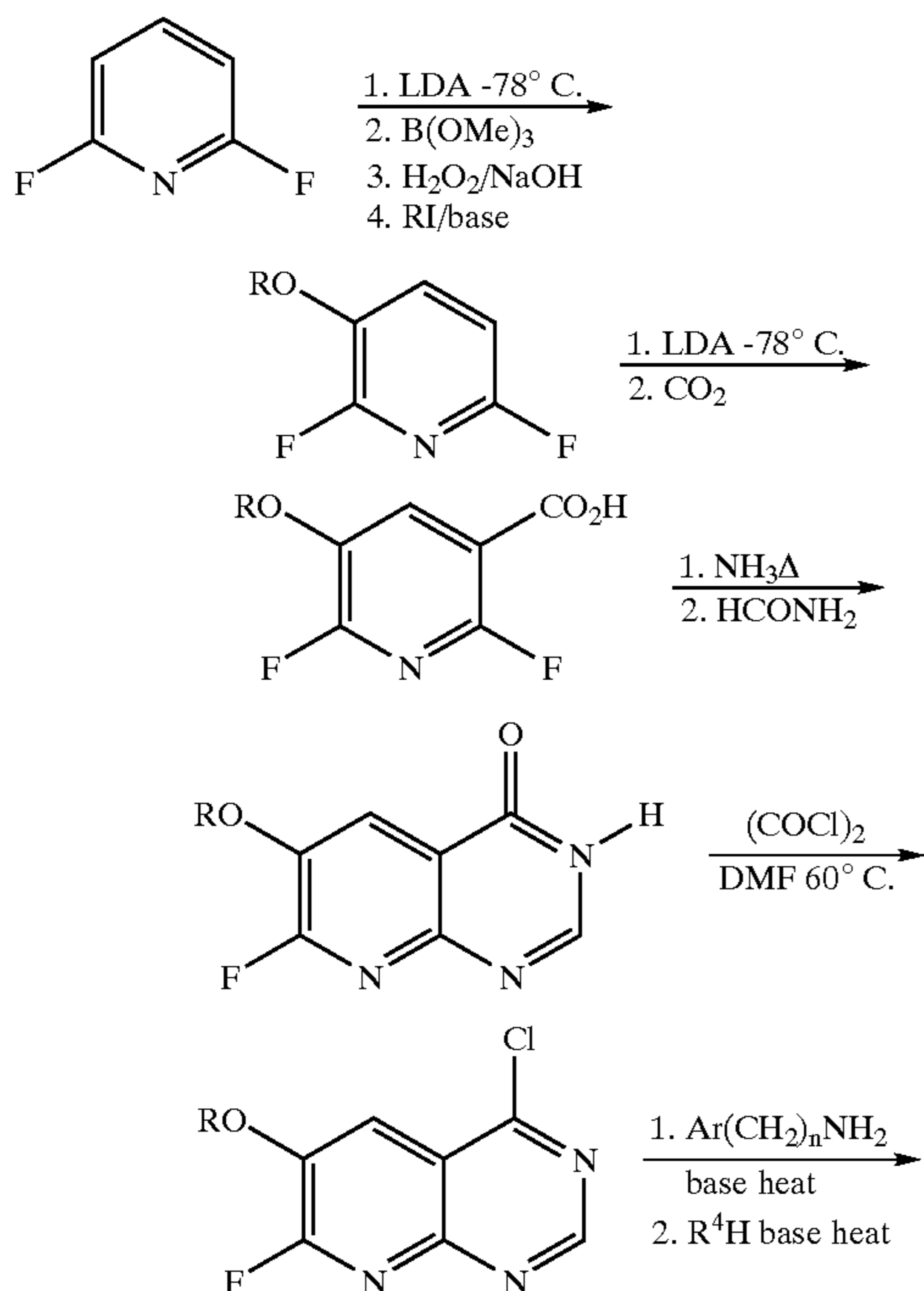
Scheme 11 Synthesis of Preferred Groups 27 & 29–31: R 3 = RO
