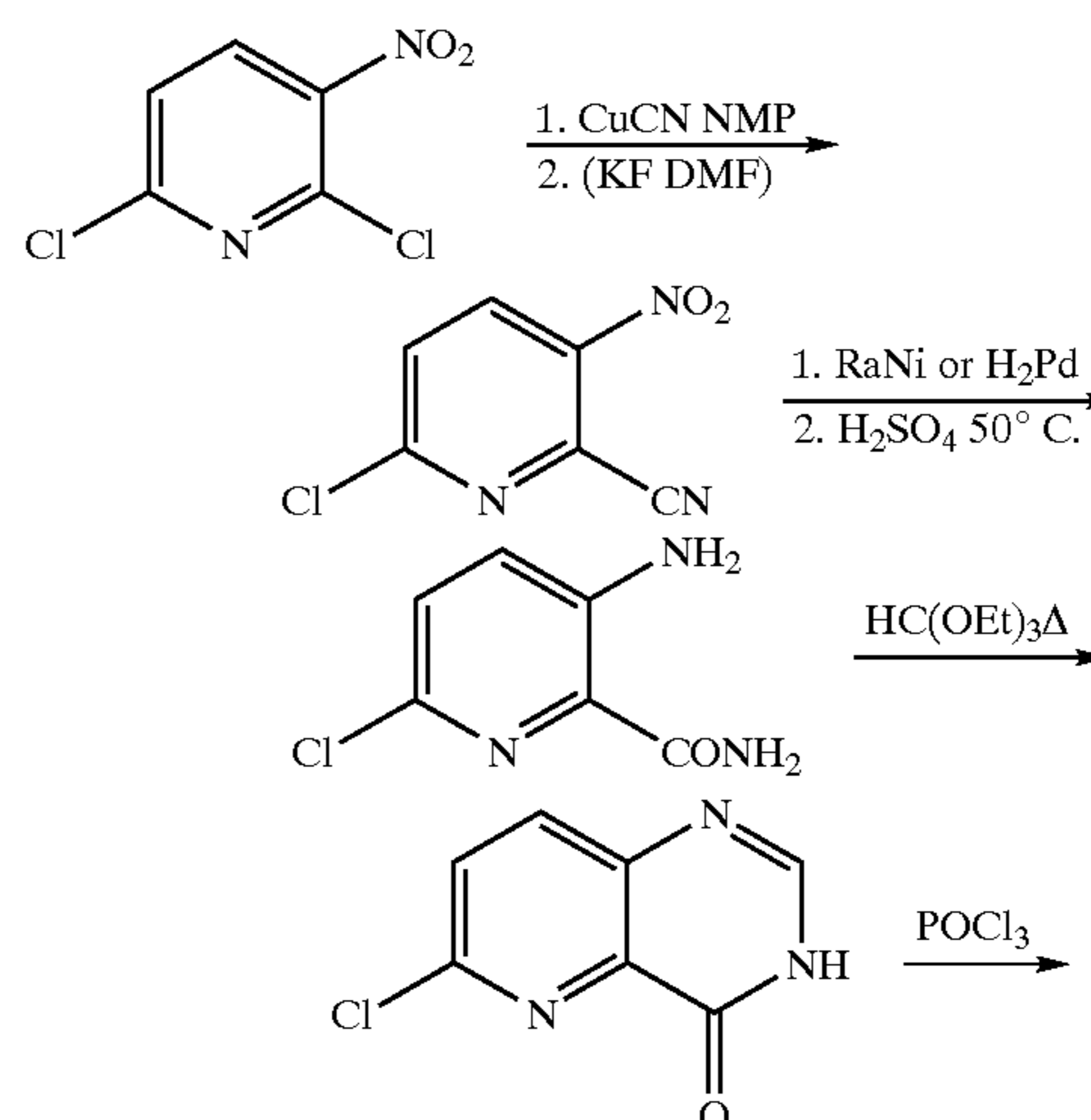
Scheme 1 Synthesis of Preferred Groups 1-5: R 4 = H
