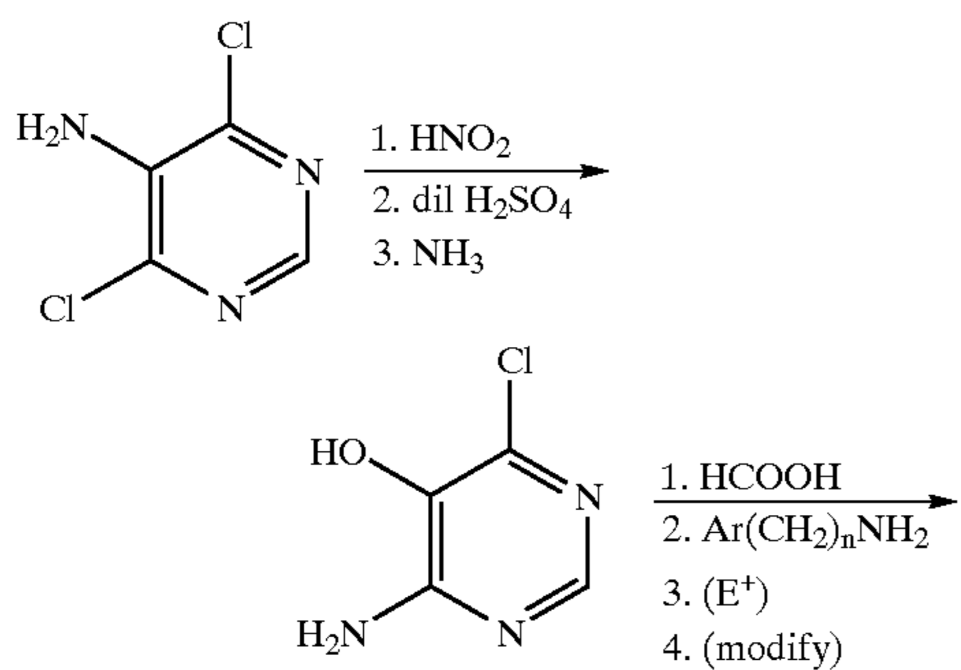
Scheme 26 Synthesis of Preferred Group 45: [4,5-d] ring fusion.
