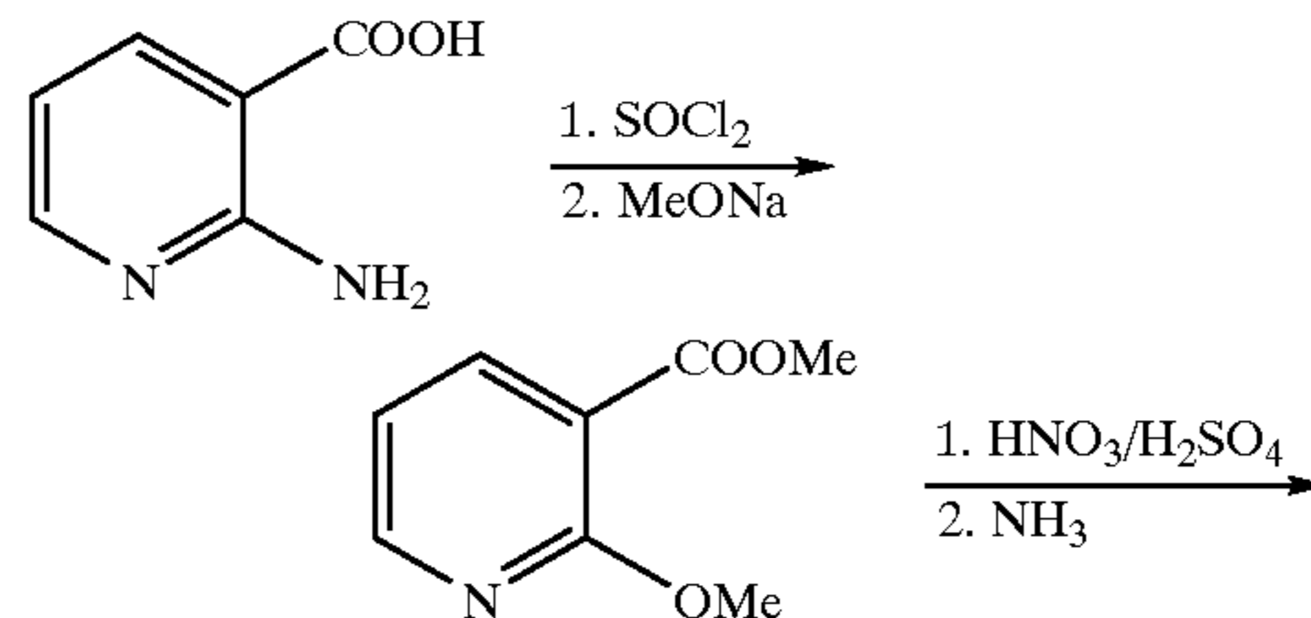
Scheme 9 Synthesis of Preferred Groups 22-26: \text{R}^4 = \text{H} .
