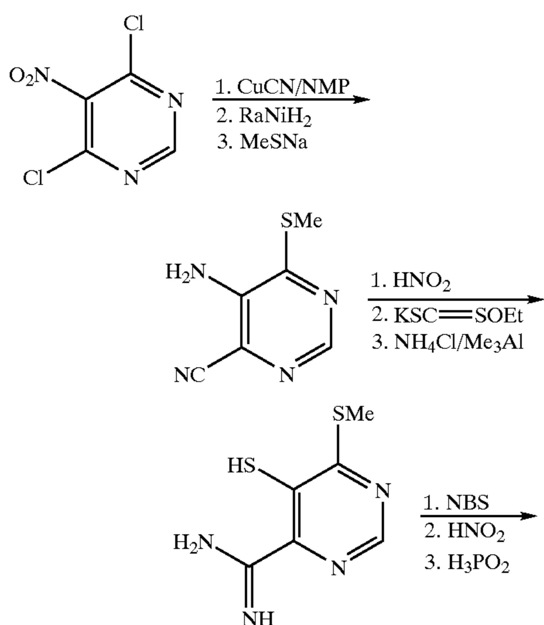
Scheme 31 Synthesis of Preferred Group 48: [4,5-d] ring fusion.
