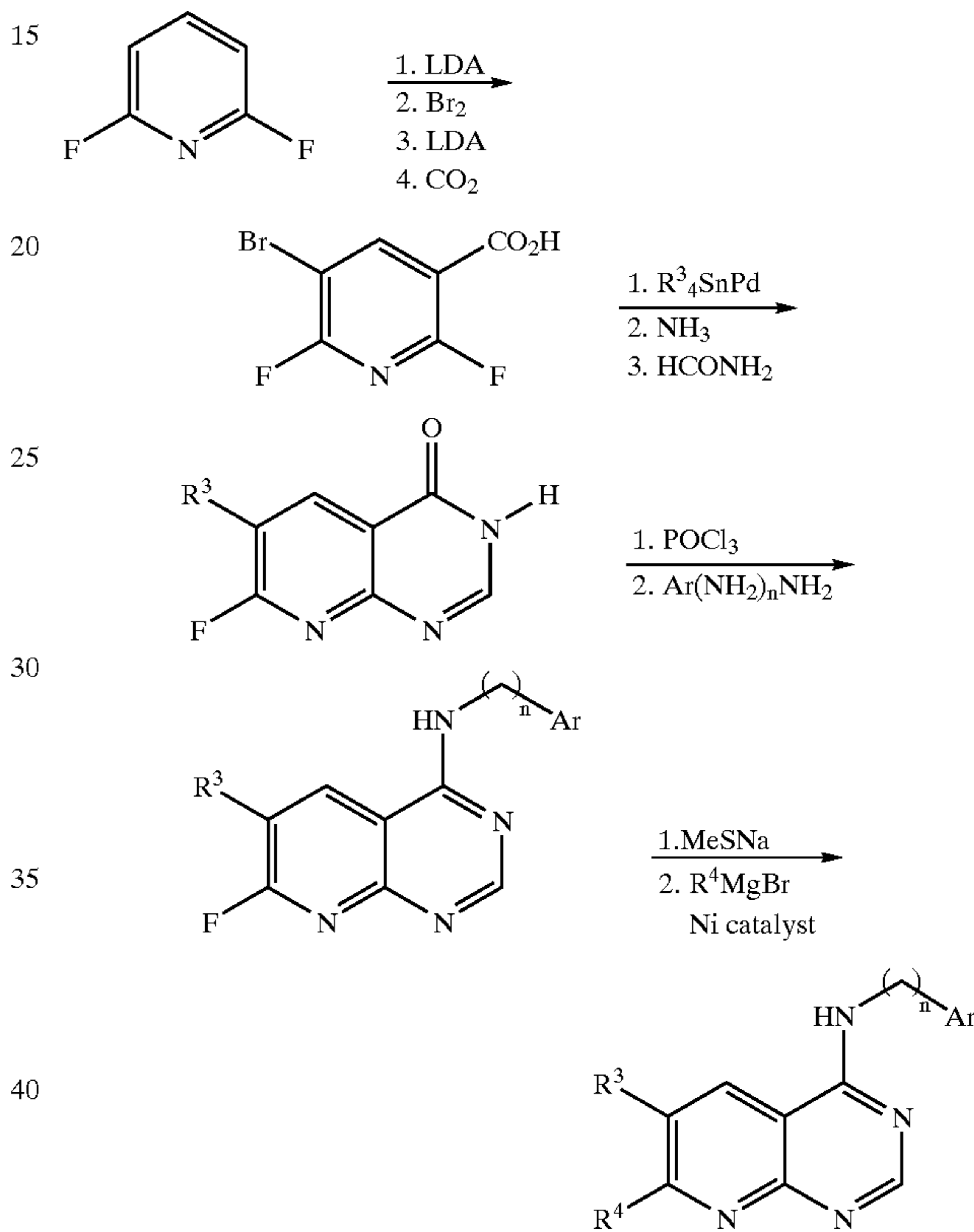
Scheme 12 Synthesis of Preferred Groups 28
