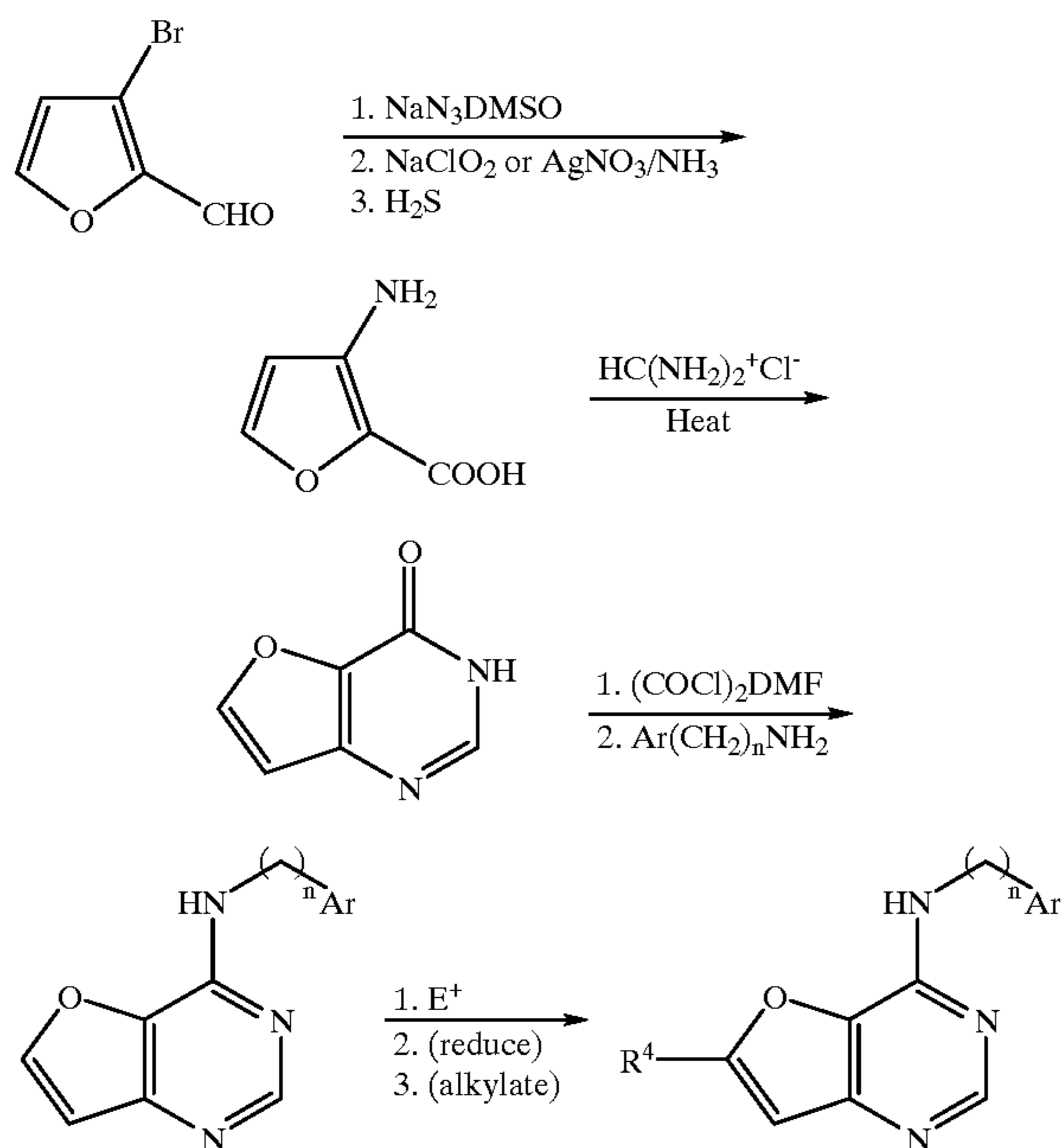
Scheme 19 Synthesis of Preferred Group 42: [3,2-d] ring fusion
