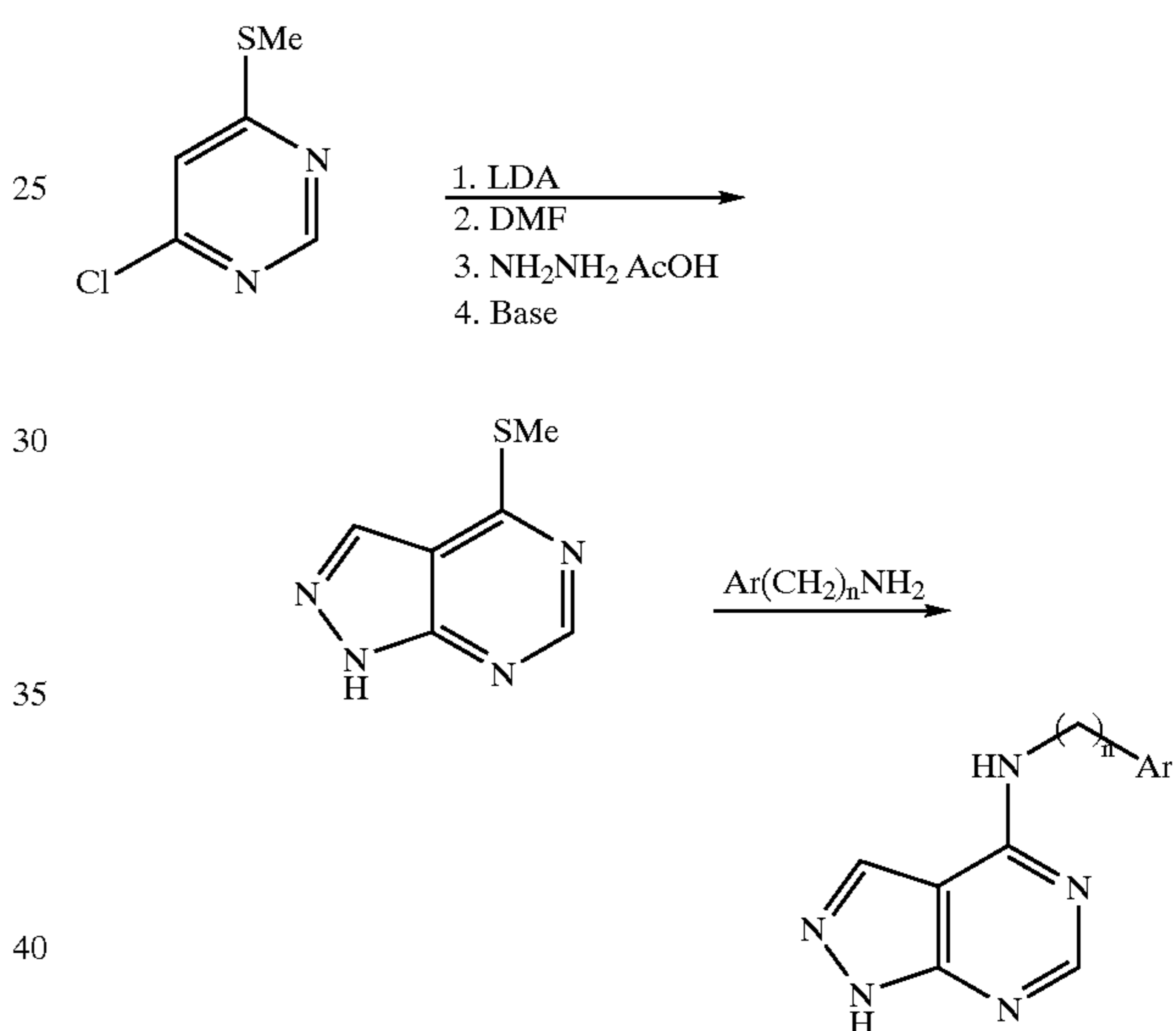
Scheme 32 Synthesis of Preferred Group 49: [3,4-d] ring fusion.
