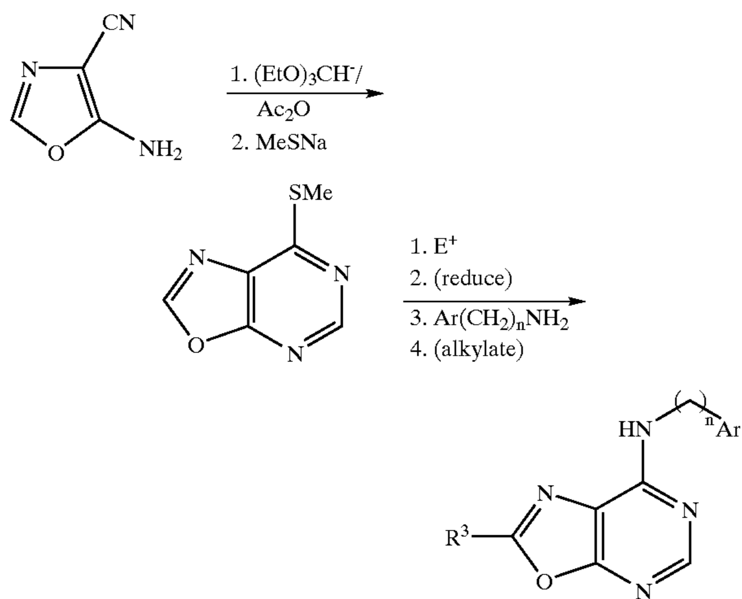
Scheme 25 Synthesis of Preferred Group 45: [5,4-d] ring fusion.
