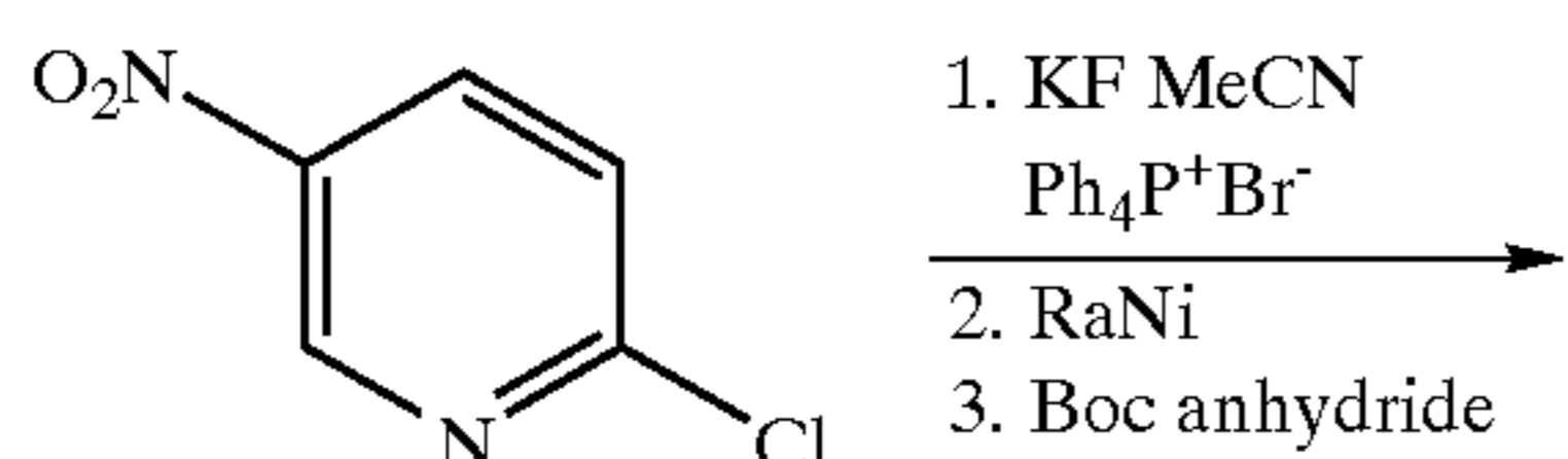
Scheme 8 Synthesis of Preferred Groups 17-21.
