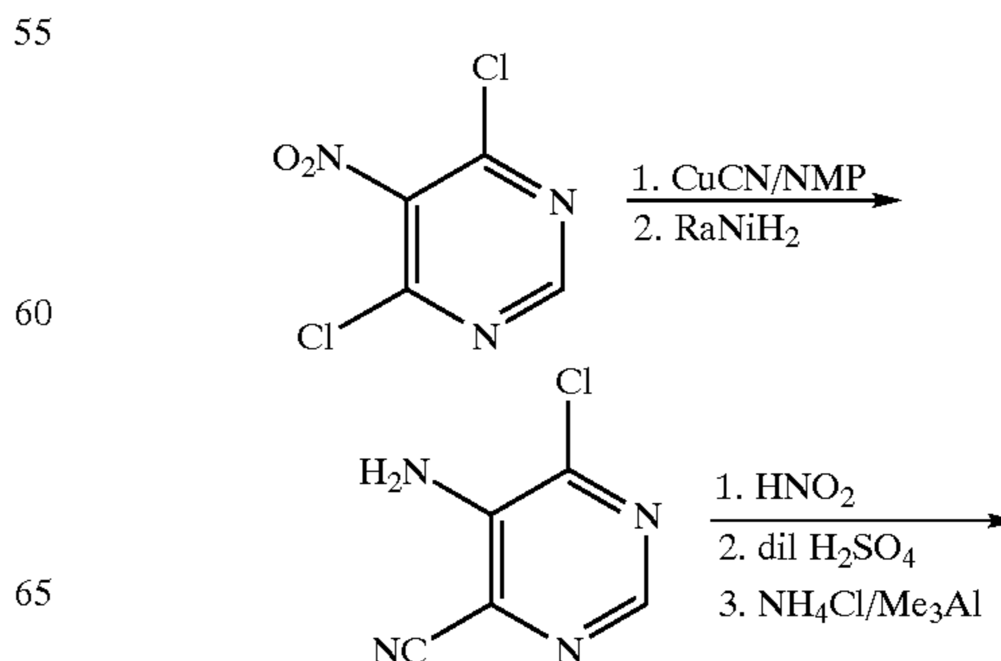
Scheme 29 Synthesis of Preferred Group 47: [4,5-d] ring fusion.
