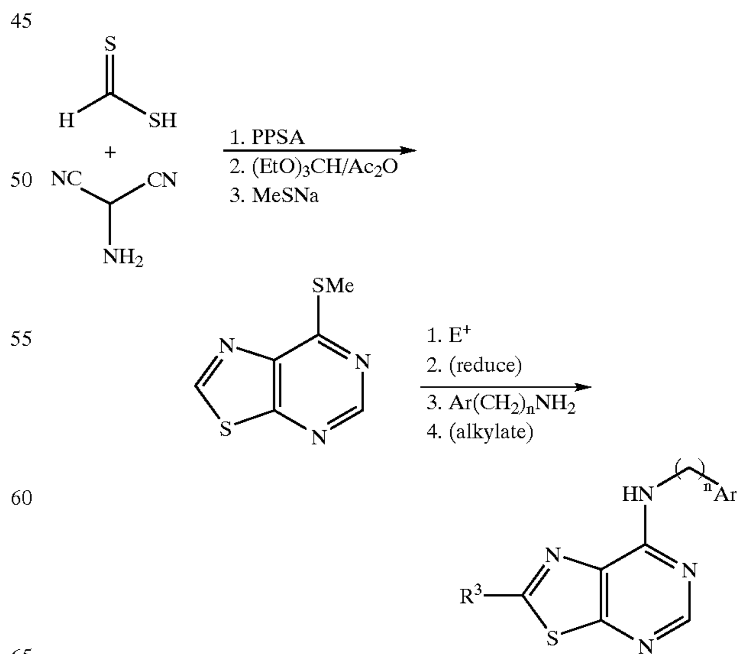
Scheme 23 Synthesis of Preferred Group 44: [5,4-d] ring fusion.
