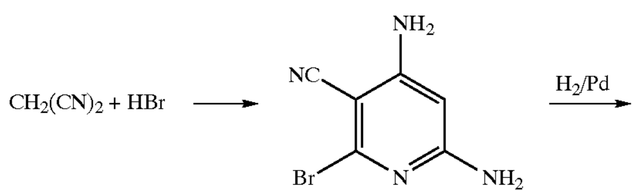
Scheme 7 Synthesis of Preferred Groups 12-16.
