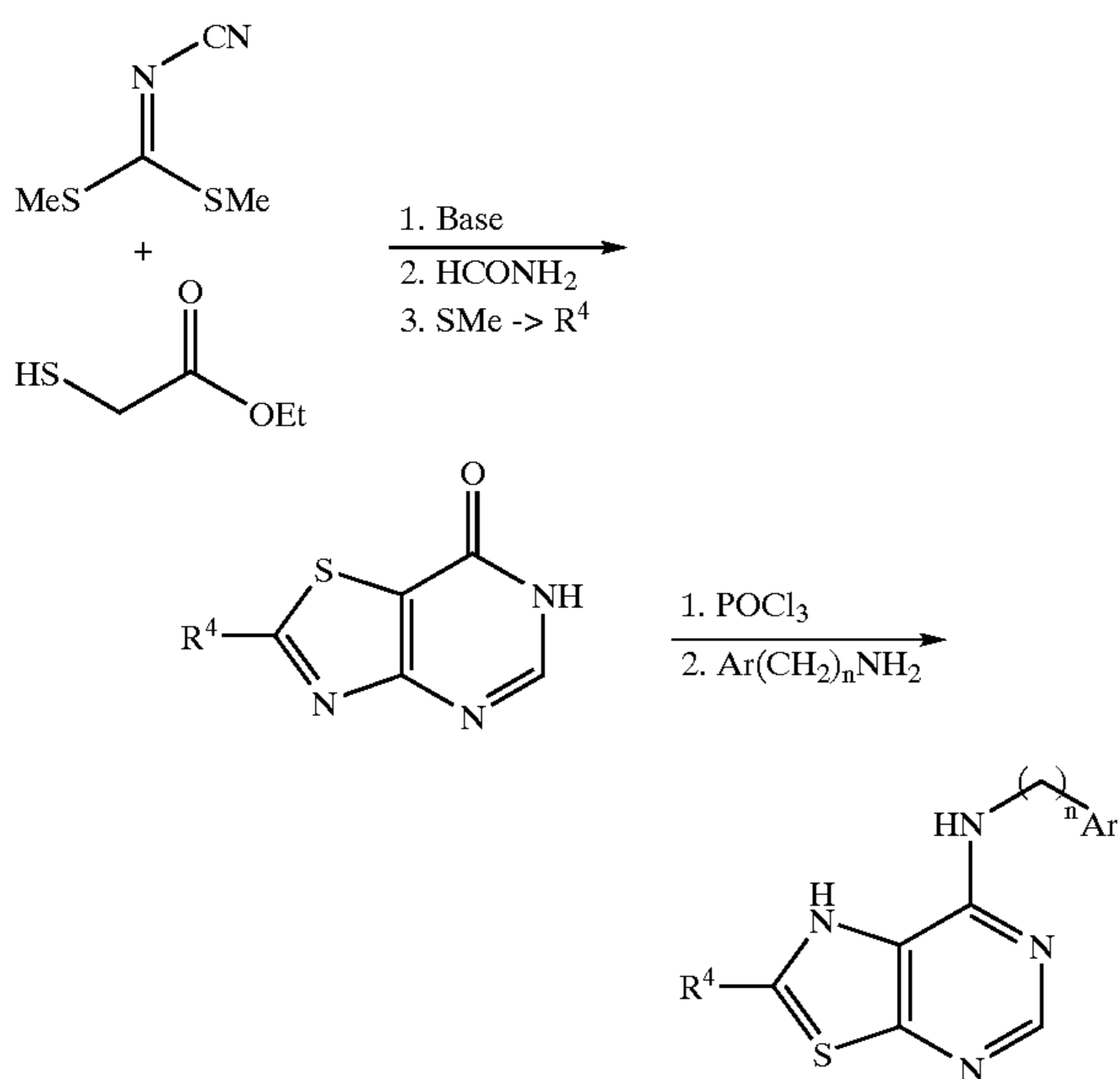
Scheme 24 Synthesis of Preferred Group 44: [4,5-d] ring fusion.
