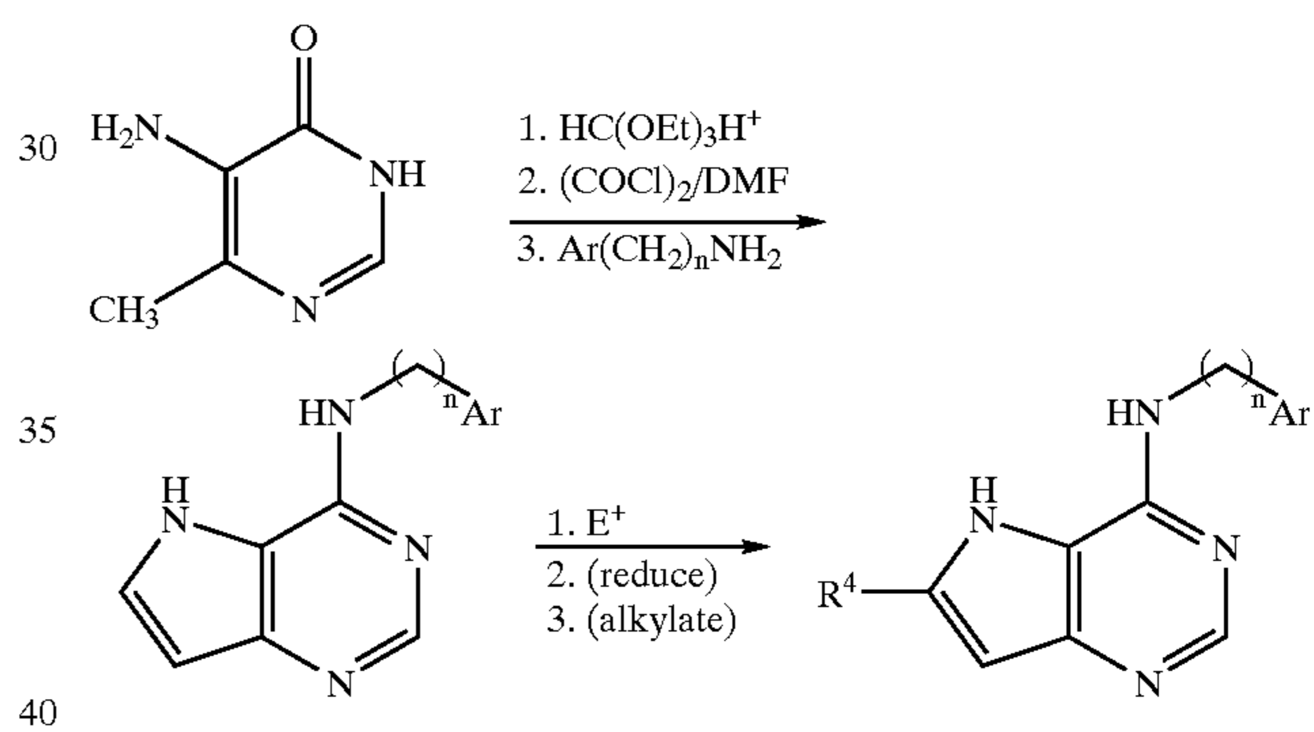
Scheme 22 Synthesis of Preferred Group 43: [3,2-d] ring fusion.
