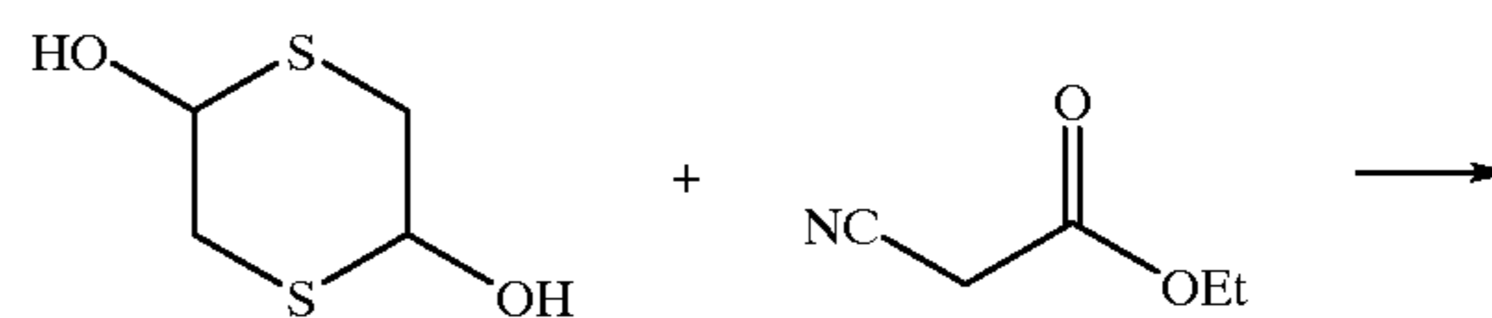
Scheme 18 Synthesis of Preferred Group 41: [2,3-d] ring fusion
