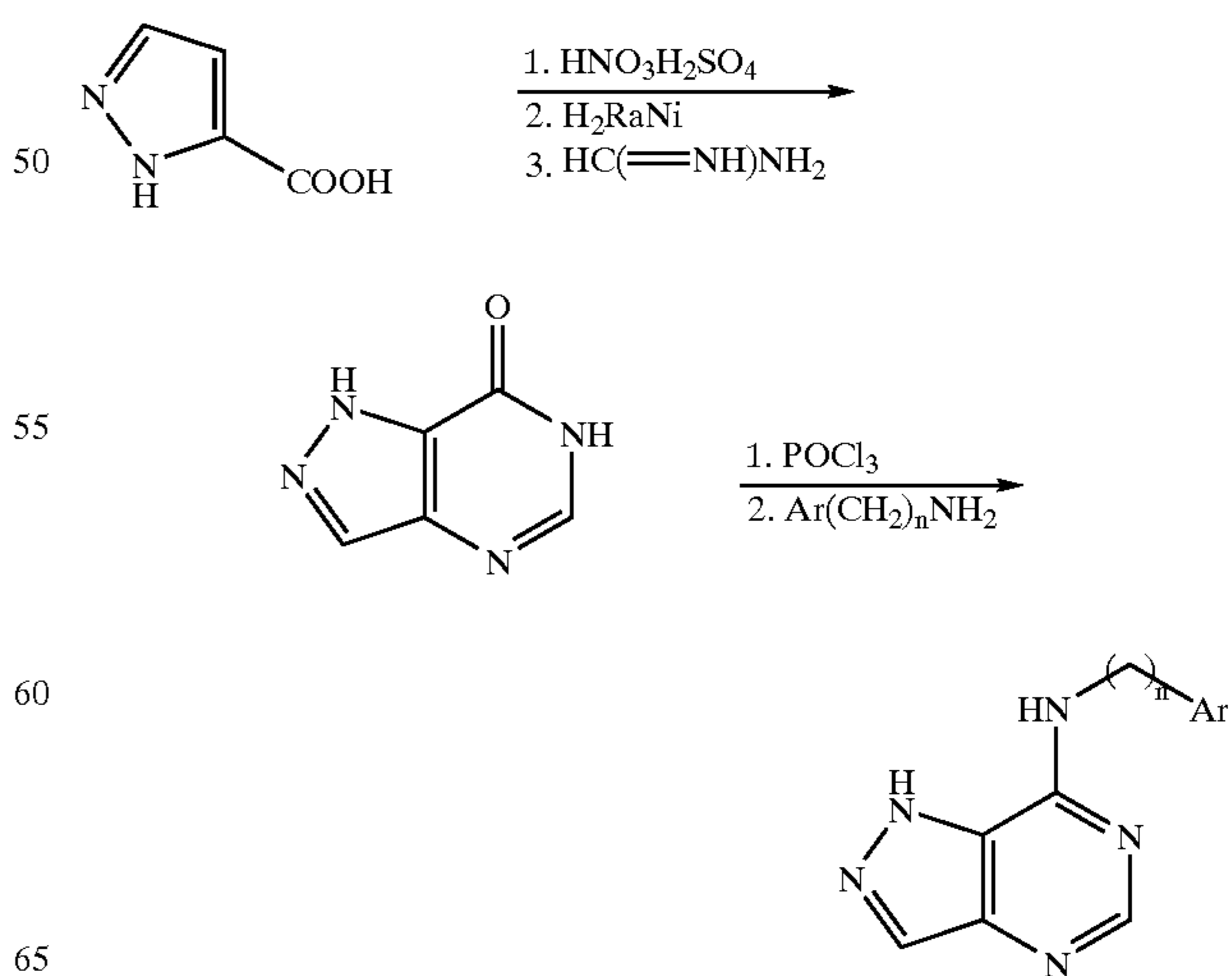
Scheme 33 Synthesis of Preferred Group 49: [4,3-d] ring fusion.
