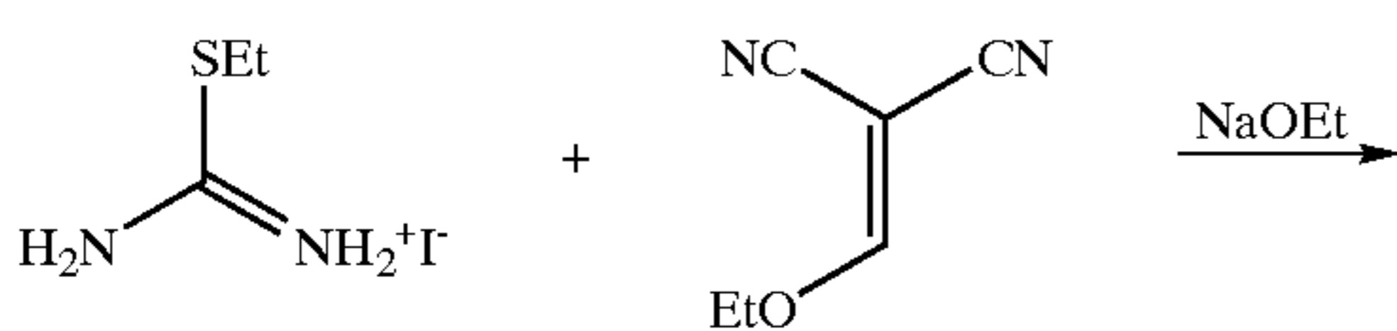
Scheme 15 Synthesis of Preferred Groups 33-36.
