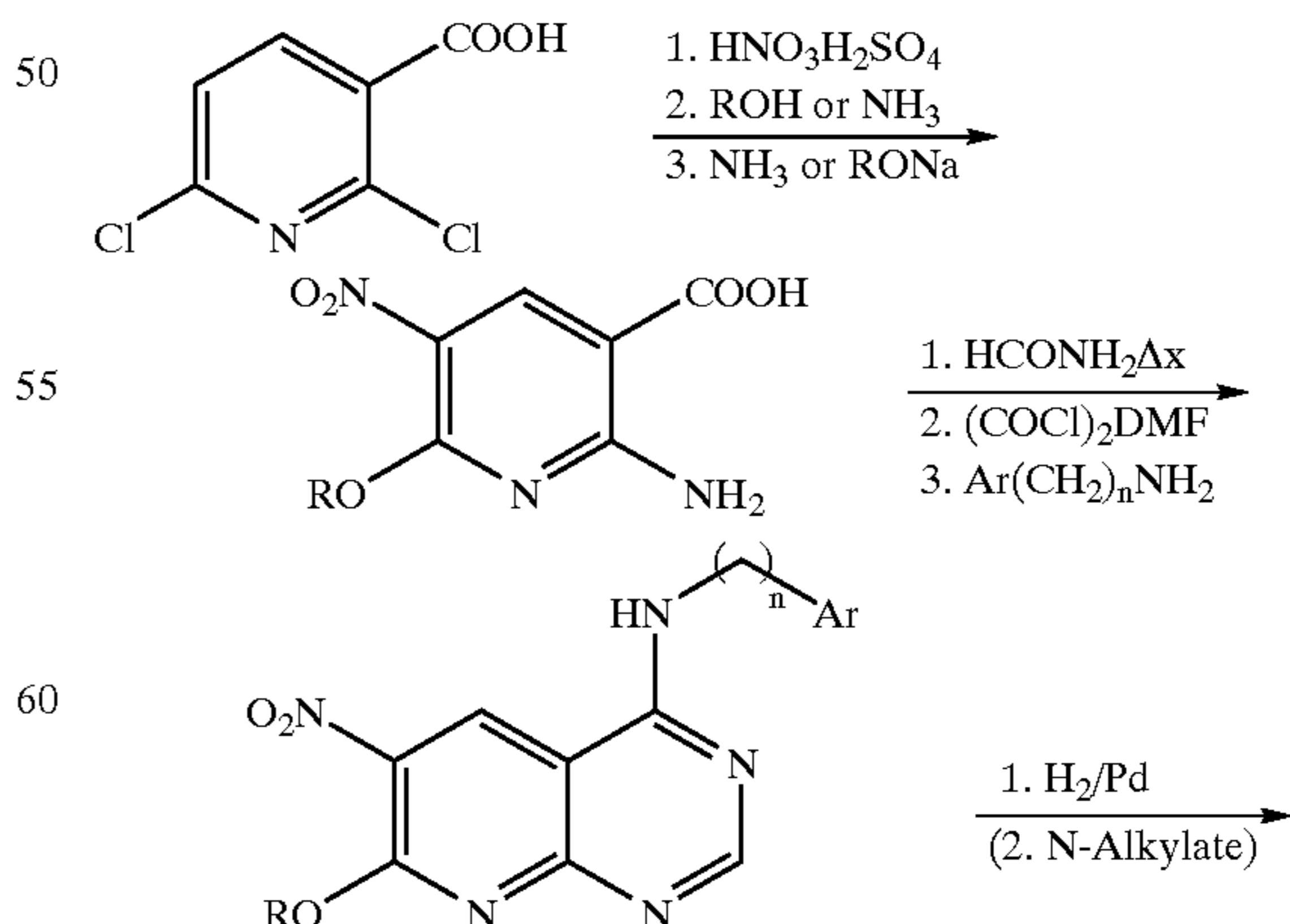
Scheme 13 Synthesis of Preferred Groups 29 & 30: R 4 = OR
