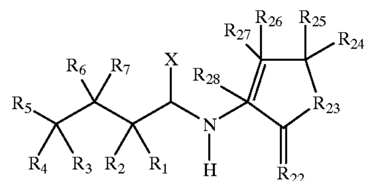
N(3-oxododecanoyl)-L-homoserine Lactone blockers:
