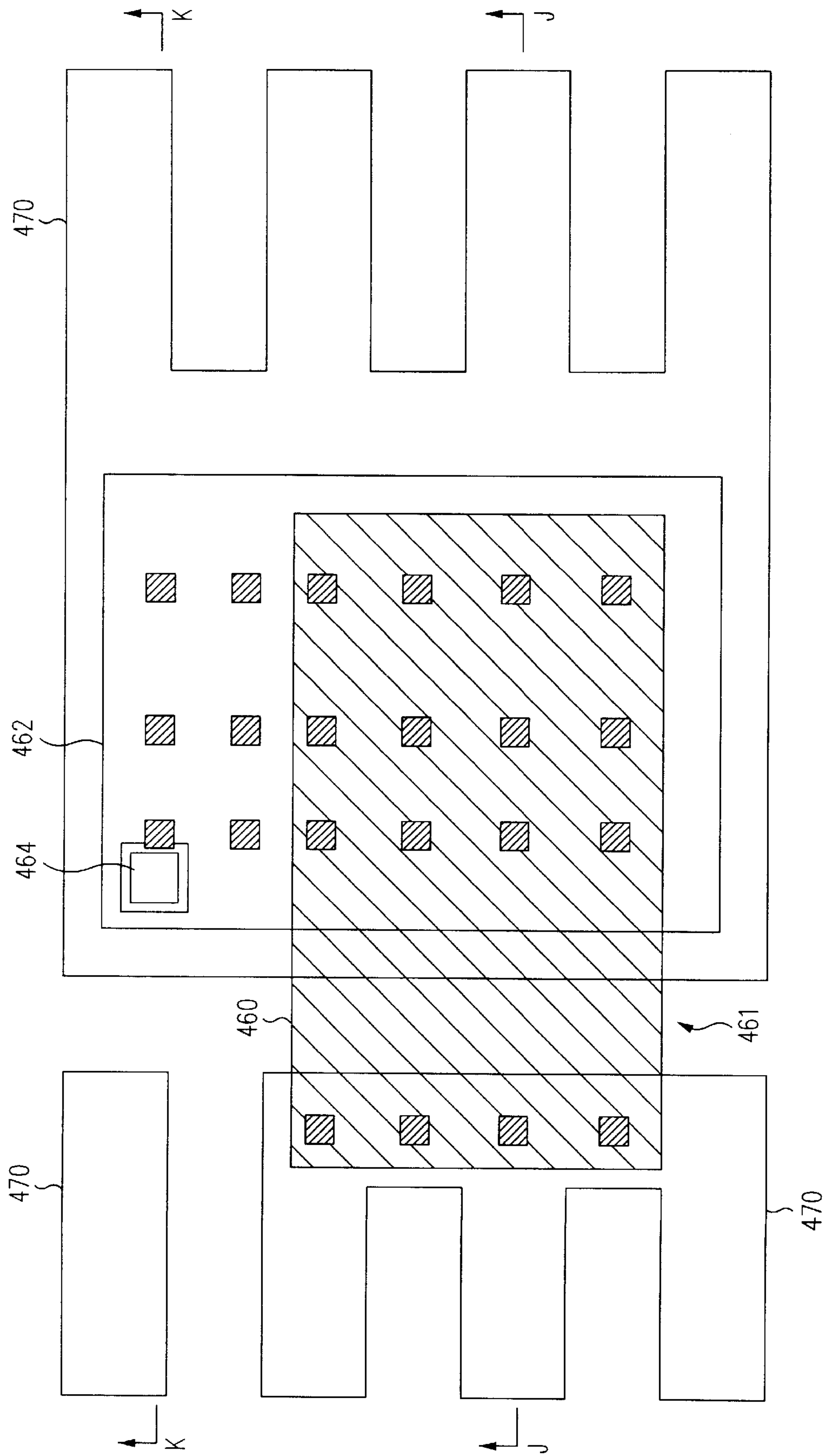
FIG. 2I (PRIOR ART)
