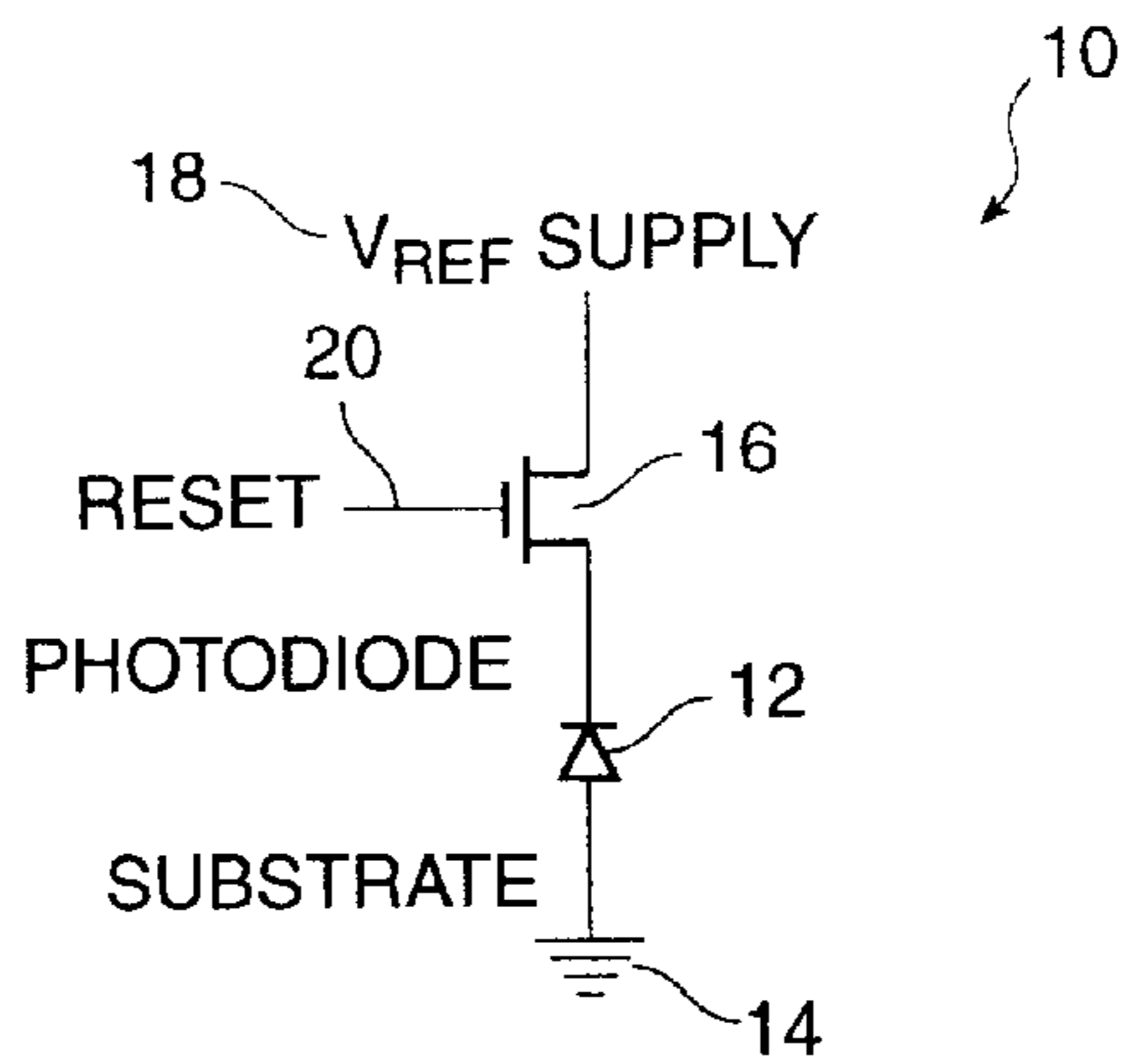
FIG. 1 (PRIOR ART)
