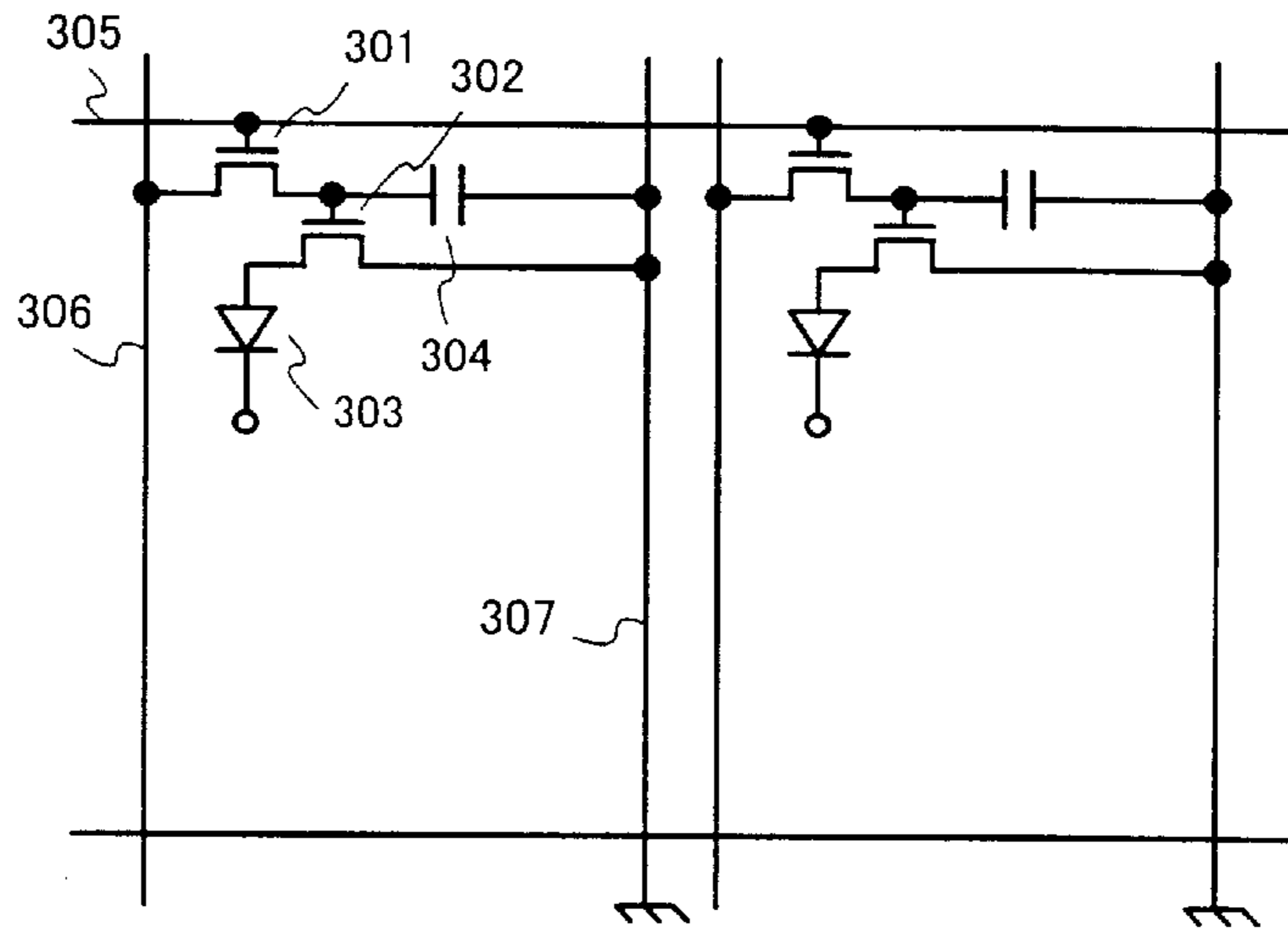
Fig. 3 (Prior Art)
