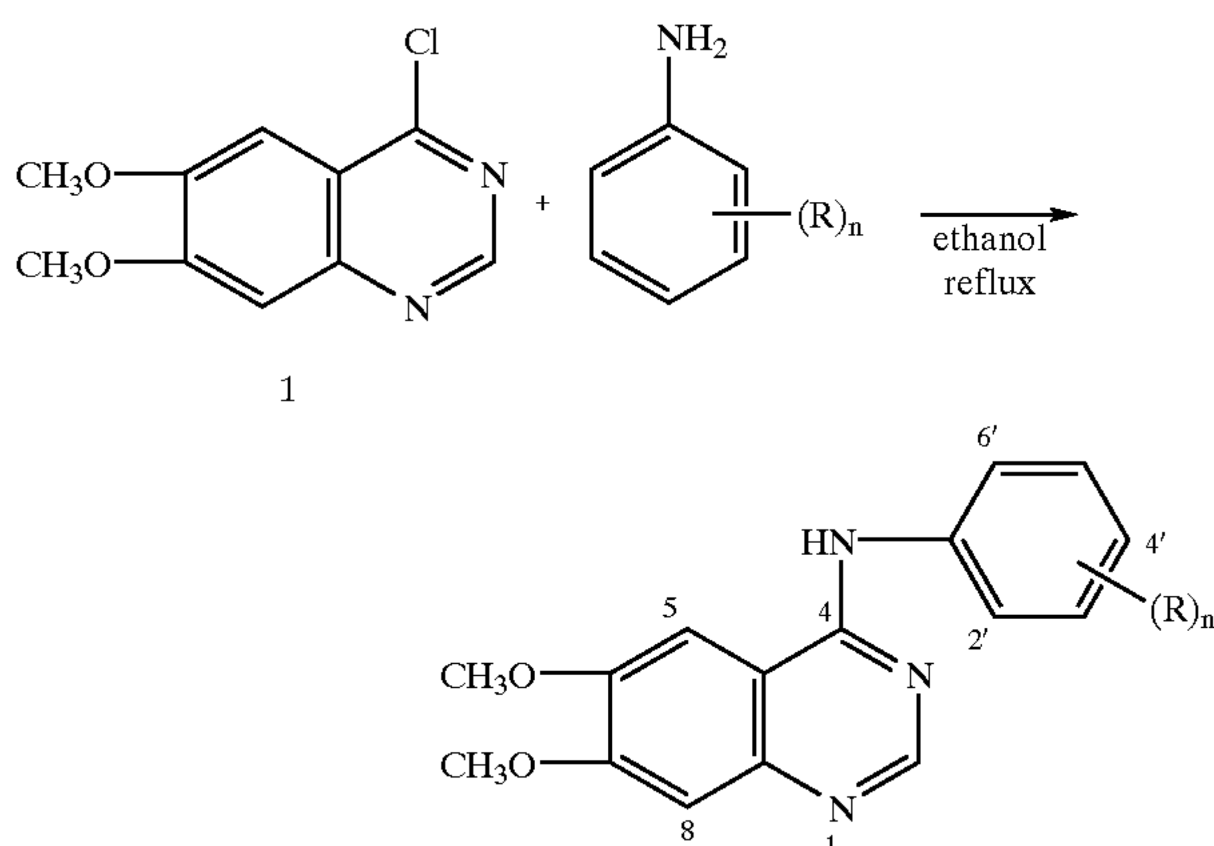
Scheme 2. Synthesis of JAK3 inhibitors.
