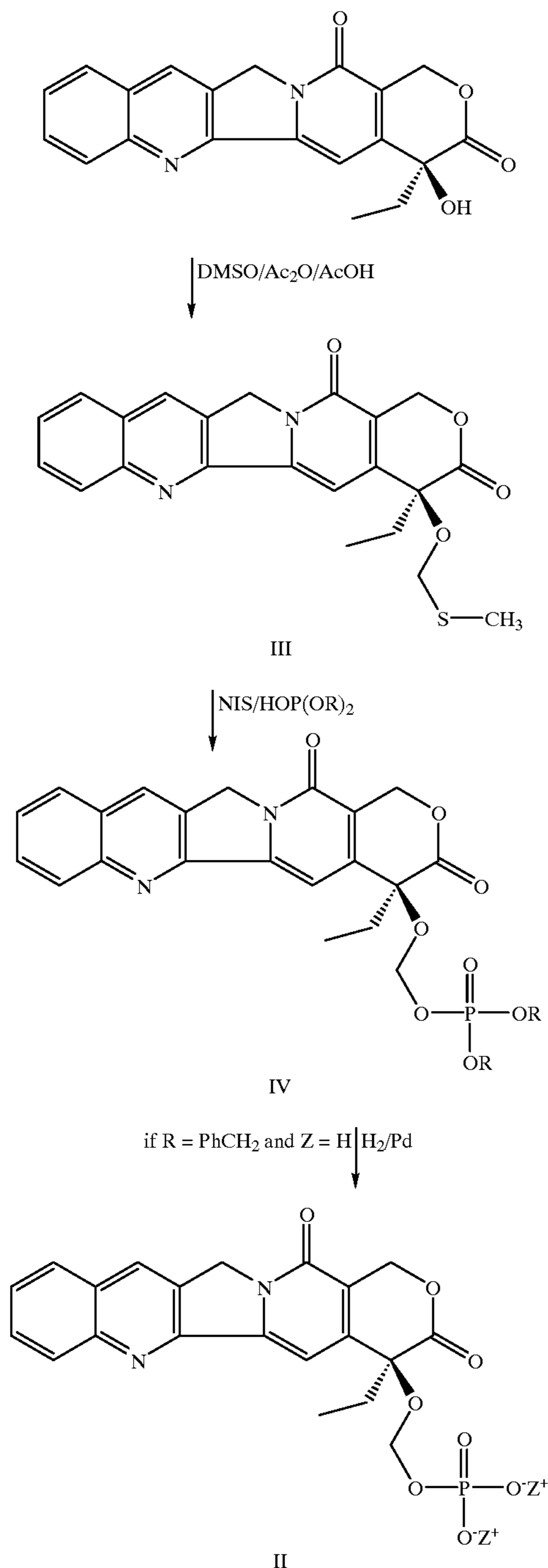
Scheme 3
