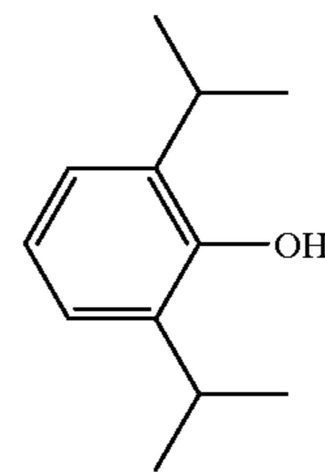
Propofol (2,6-diisopropylphenol)
