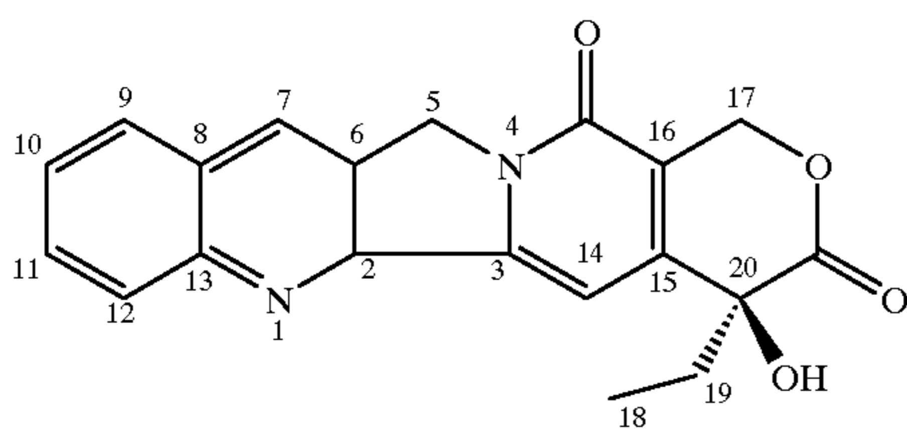
Figure 1-Camptothecin
