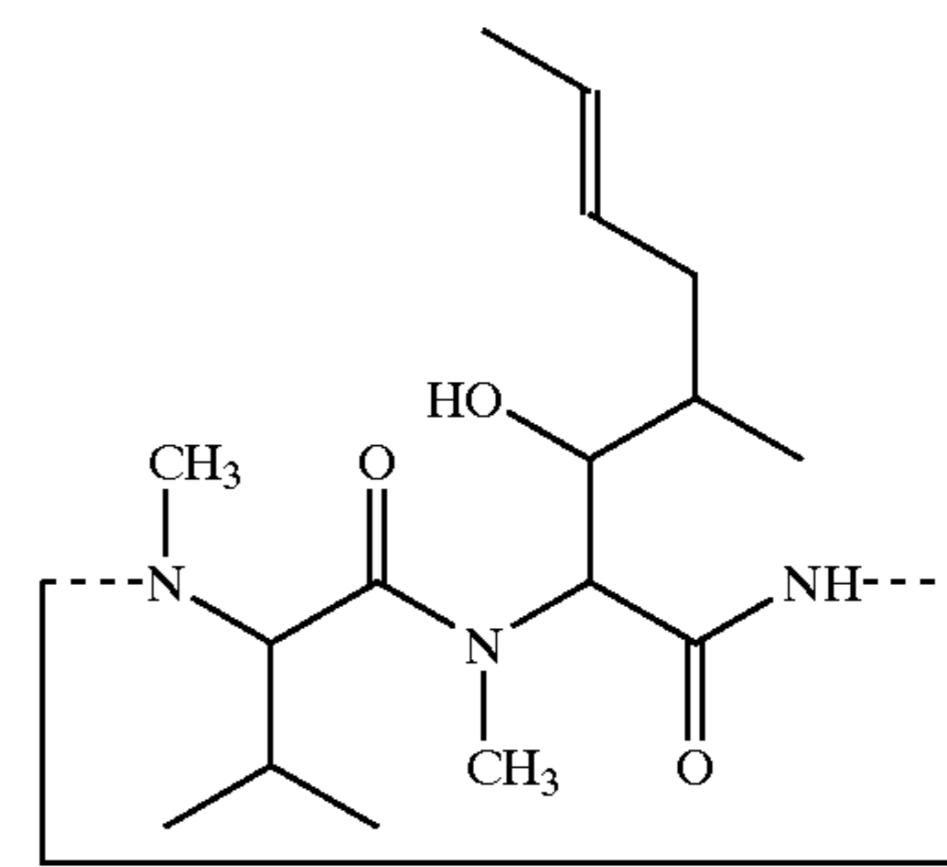
Cyclosporin A
