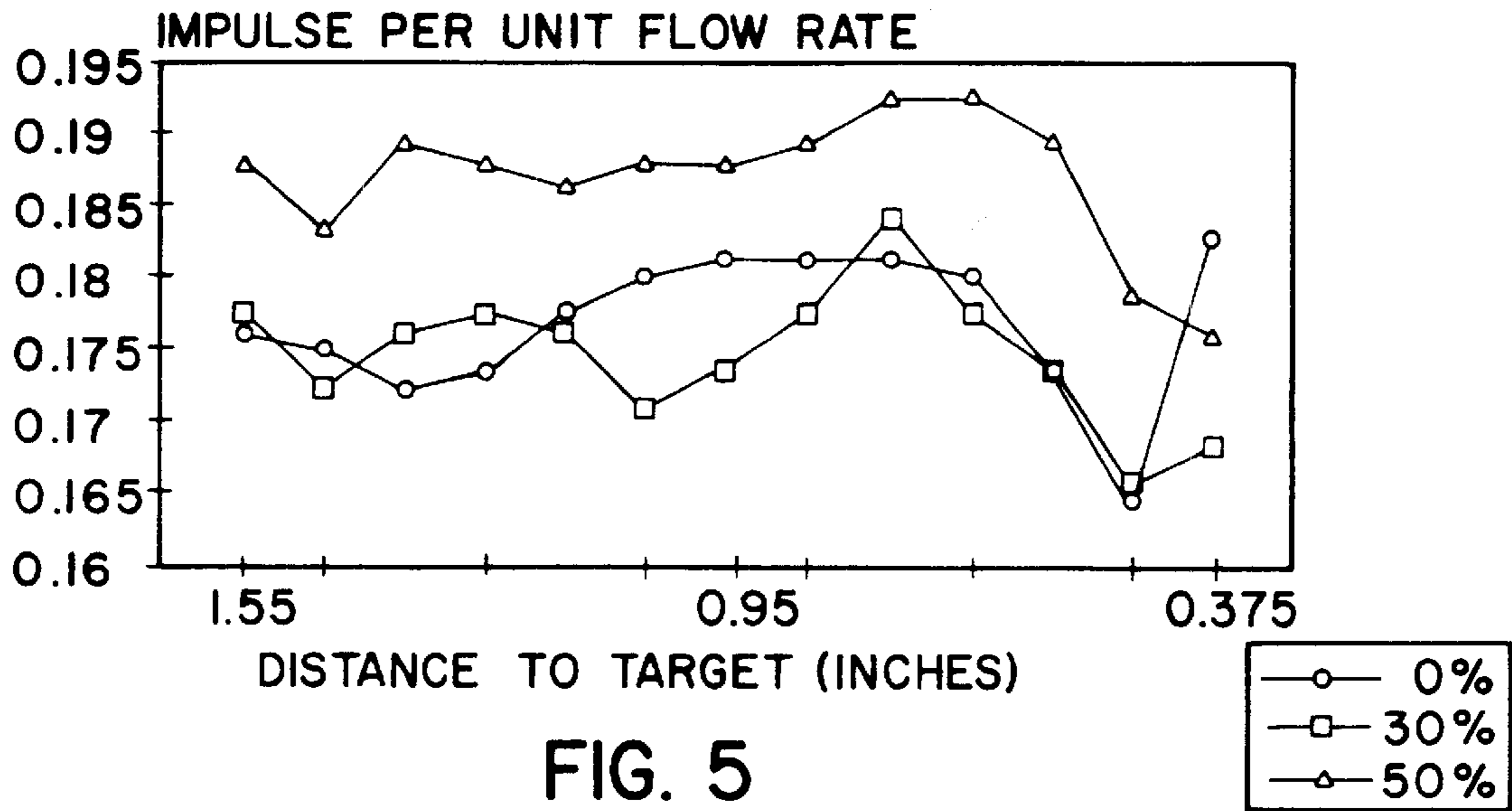
GRAPH OF IMPULSE PER UNIT FLOW RATE (800 psi)
