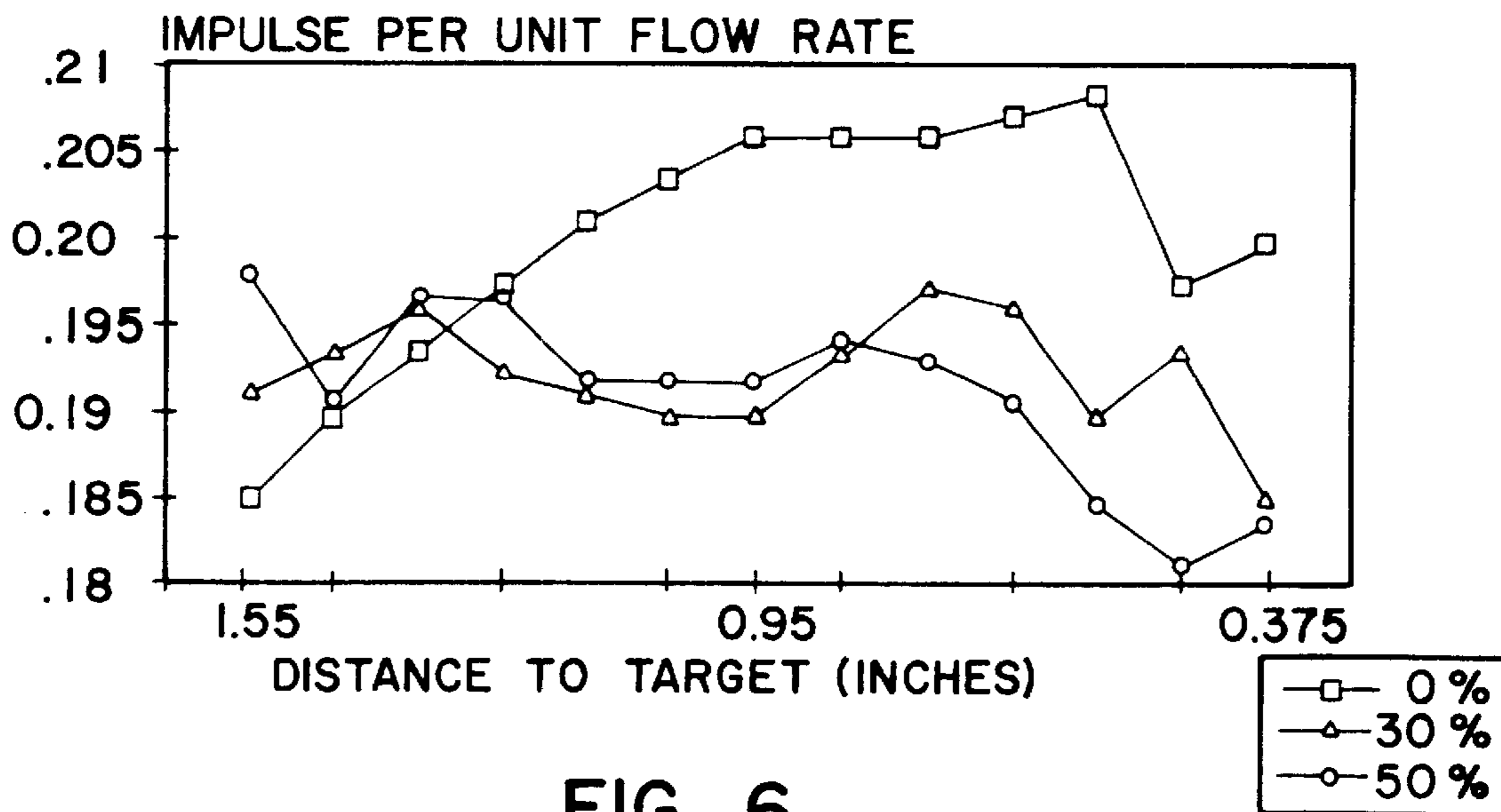
GRAPH OF IMPULSE PER UNIT FLOW RATE (1000 psi)
