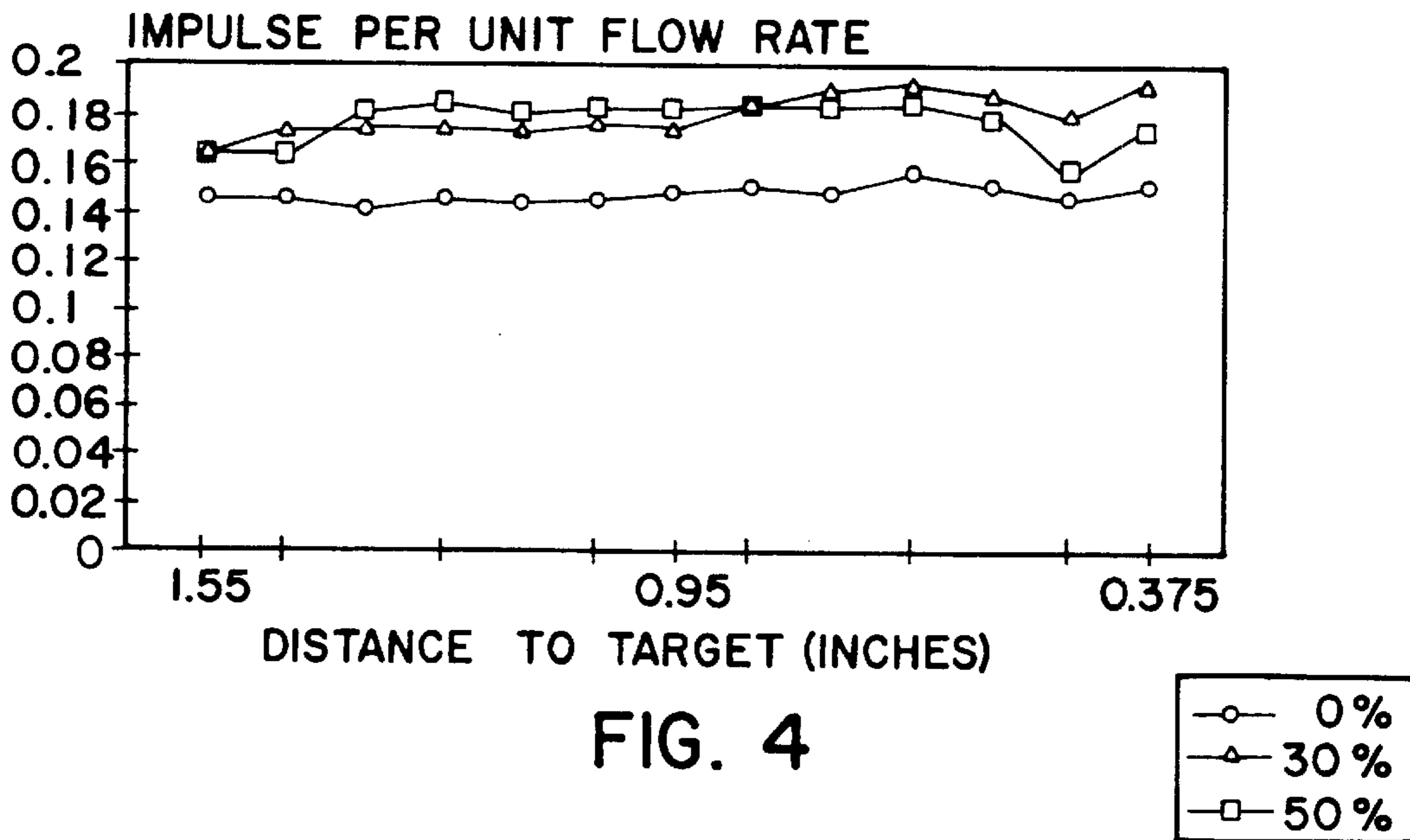
GRAPH OF IMPULSE PER UNIT FLOW RATE (600 psi)
