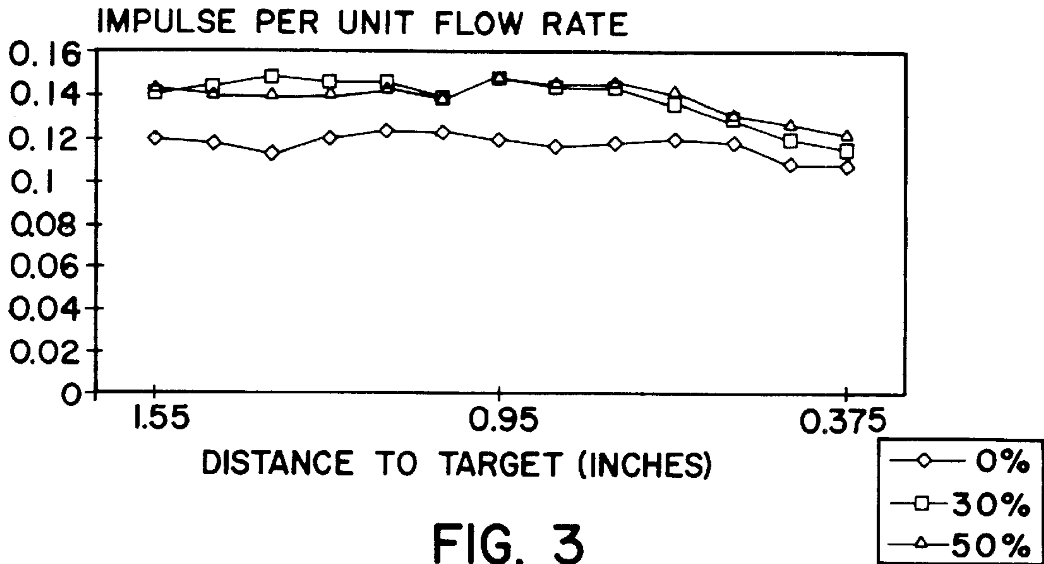
GRAPH OF IMPULSE PER UNIT FLOW RATE (400 psi)
