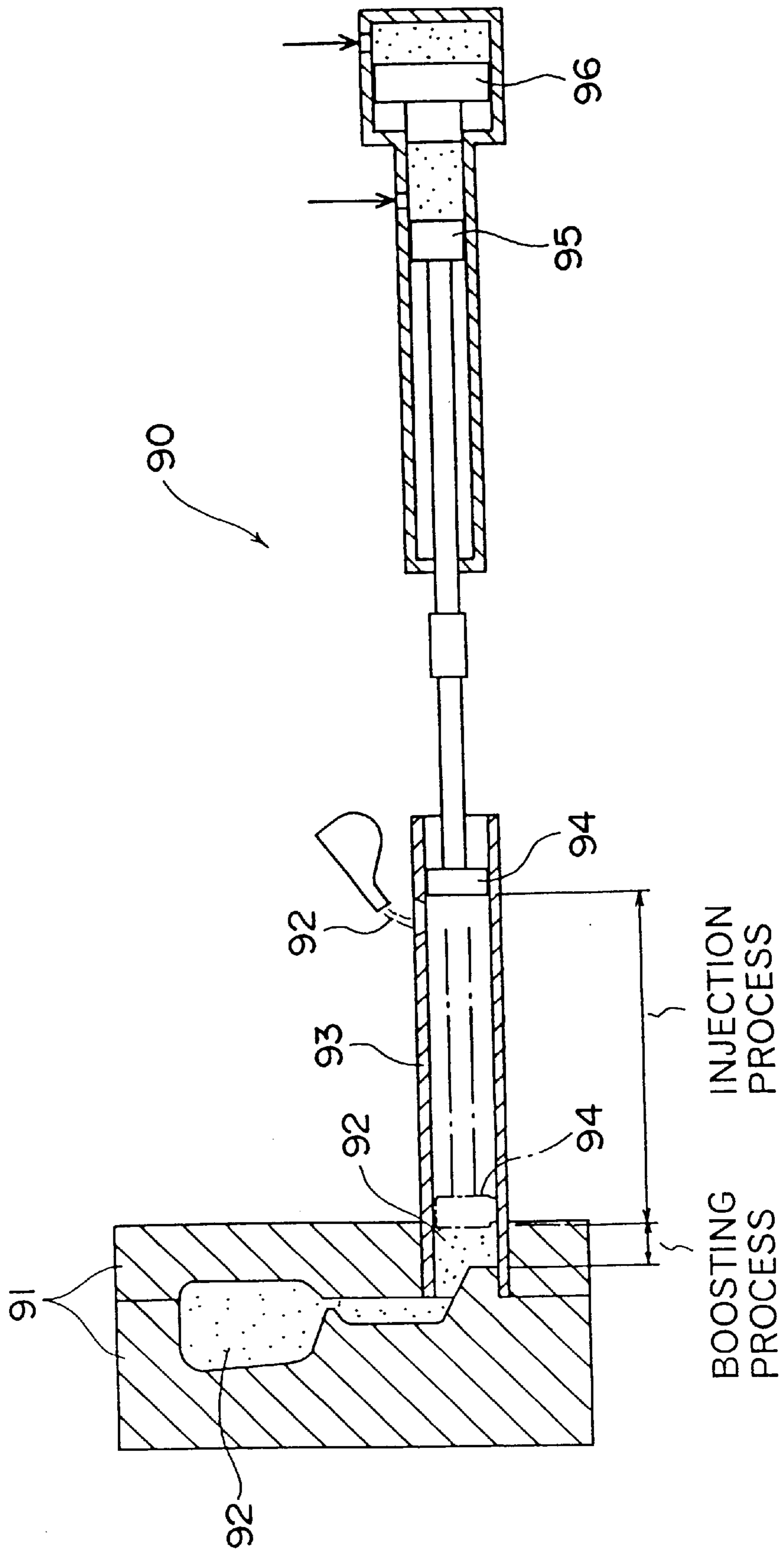
FIG. 6 PRIOR ART
