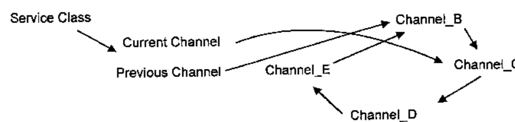
Receive Channel Ring after Channel_B is Served But it is Not Run-Limited
