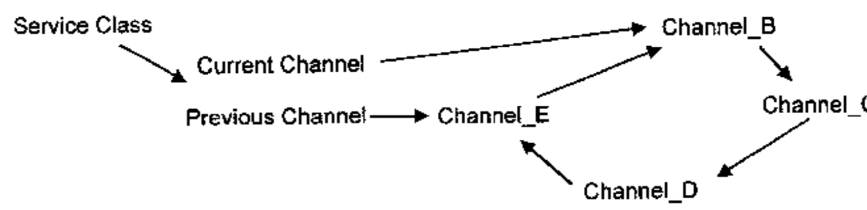
Receive Channel Ring after Channel_A Becomes Run-Limited
