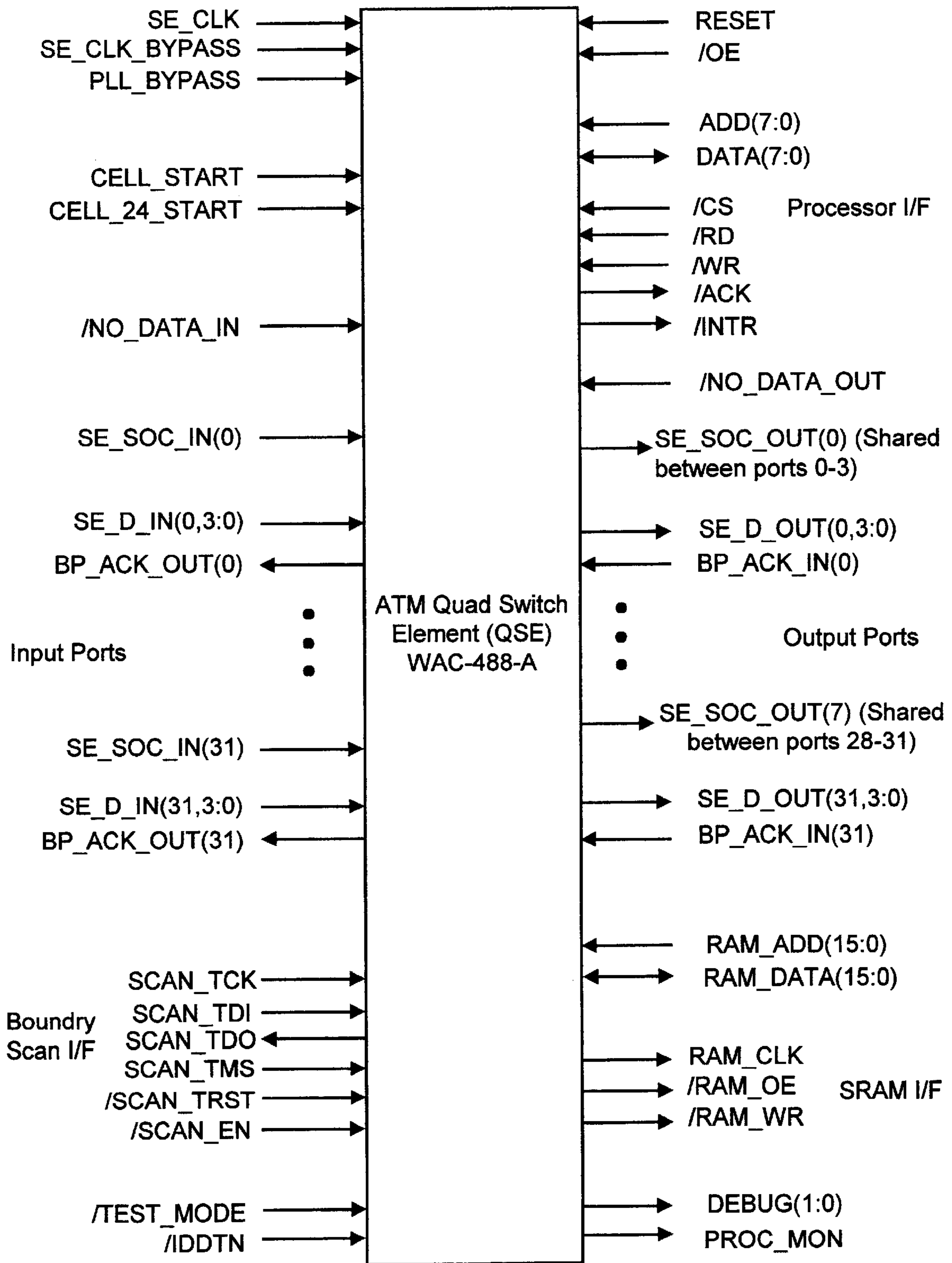
QSE Pinout Block Diagram
