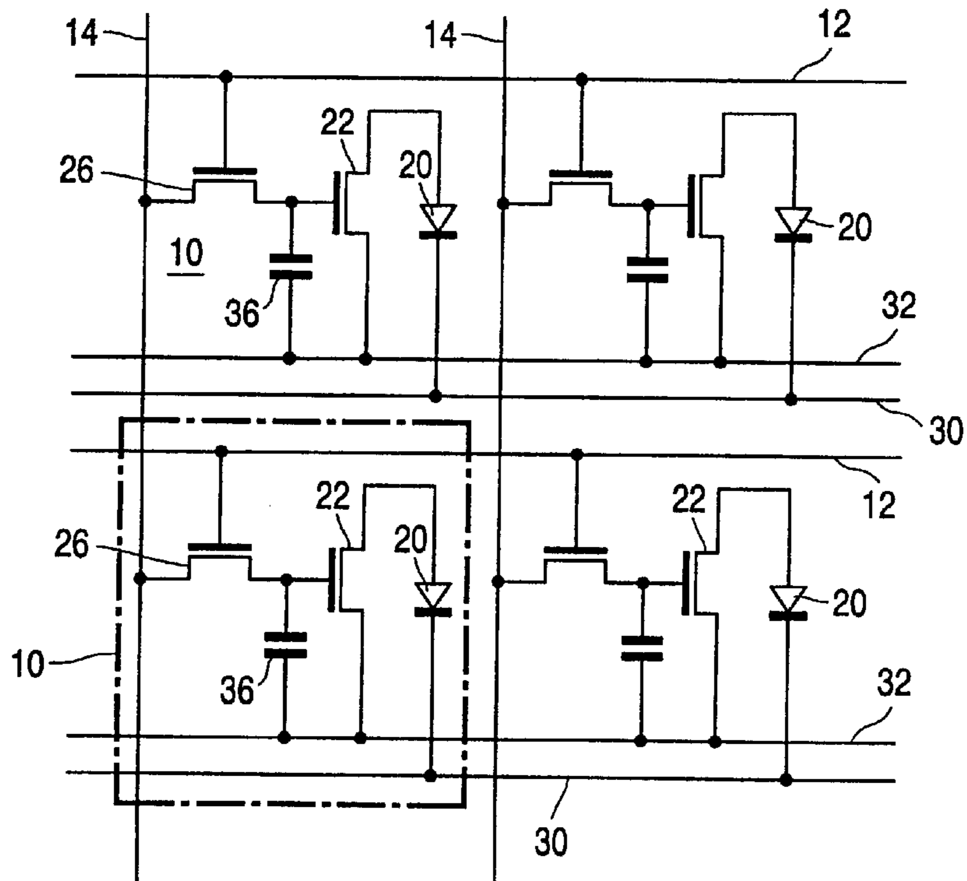
FIG. 2 PRIOR ART
