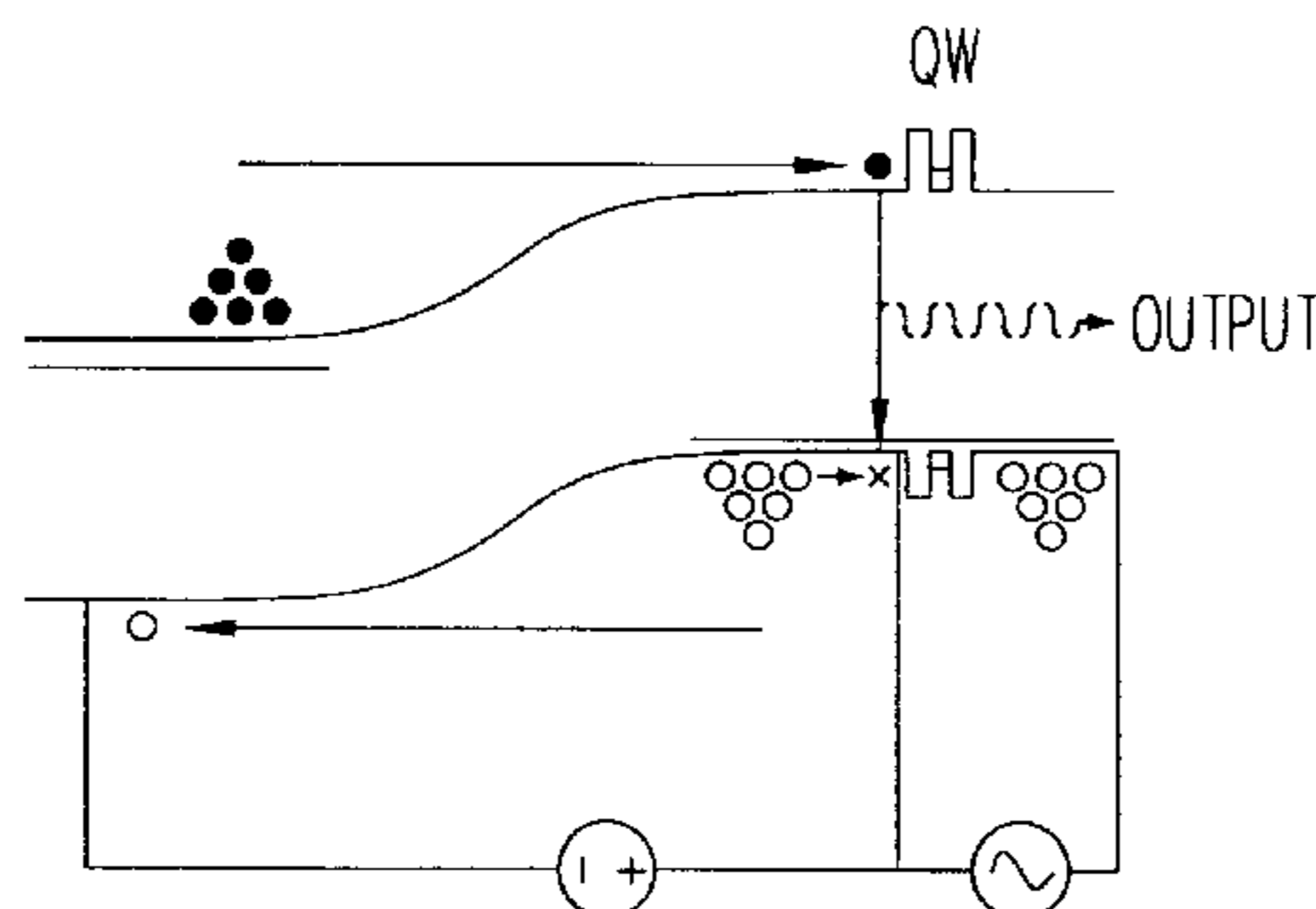
ELECTRICALLY MODULATED RESONANT TUNNELING BARRIER- LIGHT ON LED FORWARD BIASED, BARRIER UNBIASED
