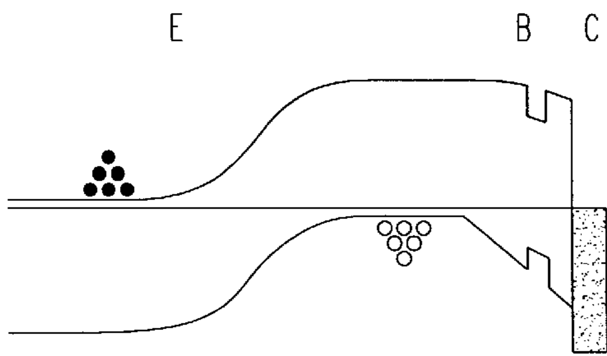
OPTICALLY MODULATED TRIANGULAR BARRIER (NON-INVERTING) LED UNBIASED, NO INCIDENT LIGHT
