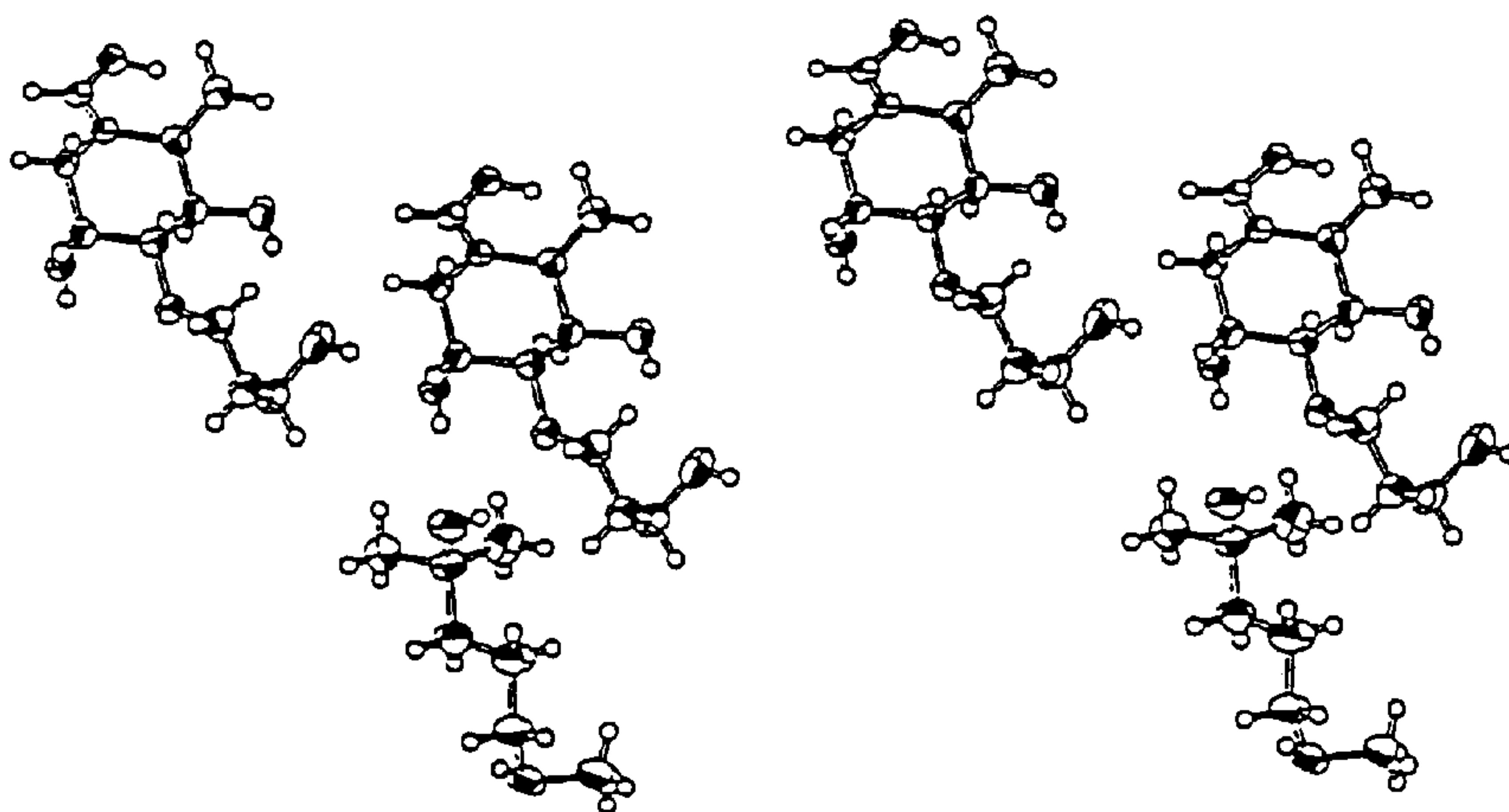
Structure of ED-71 where hydrogen bonds are focused (2); Stereographic view
