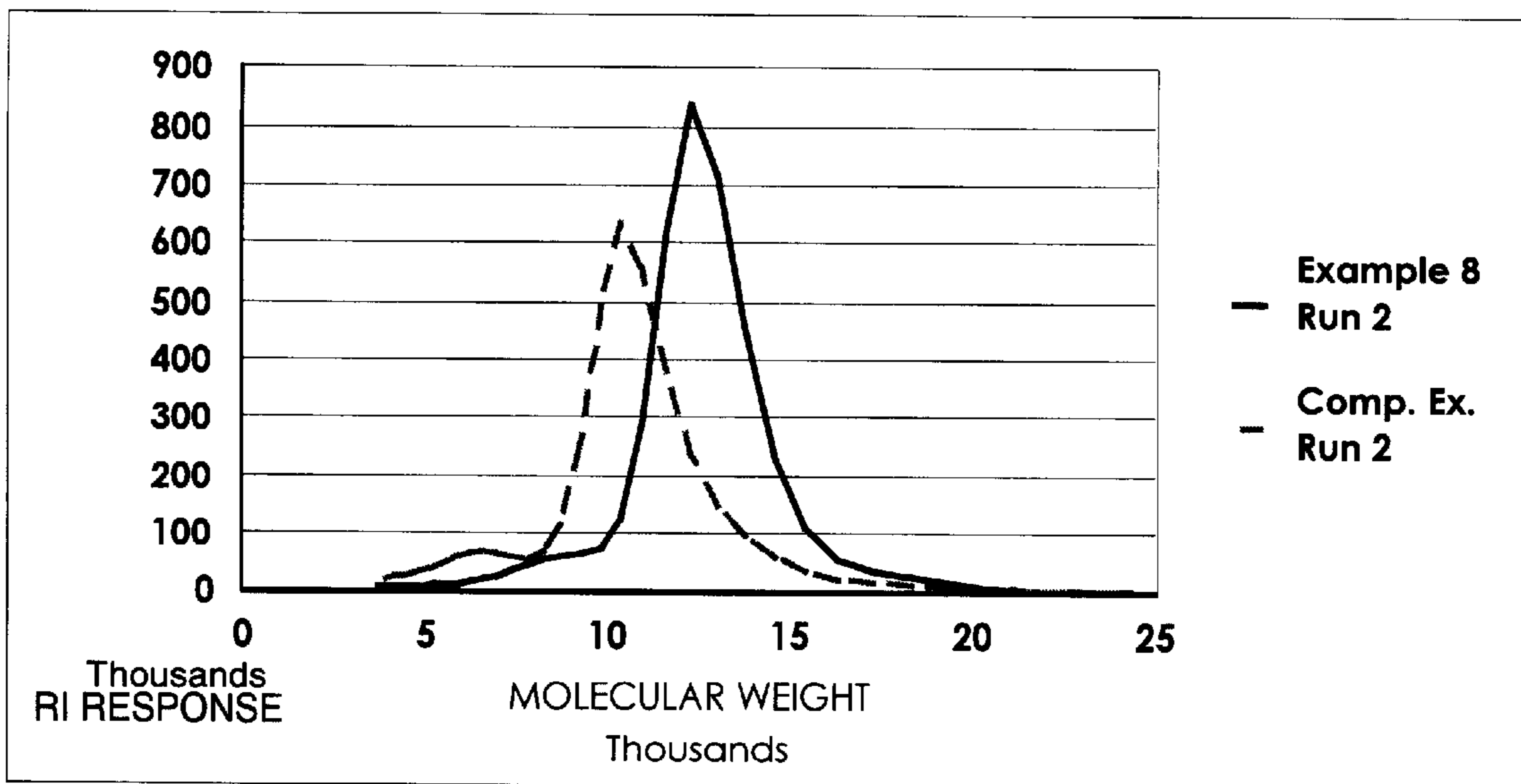
FIGURE 1. SIZE EXCLUSION CHROMATOGRAM OF POLYETHER POLYOLS MADE WITH DIFFERENT CATALYSTS
