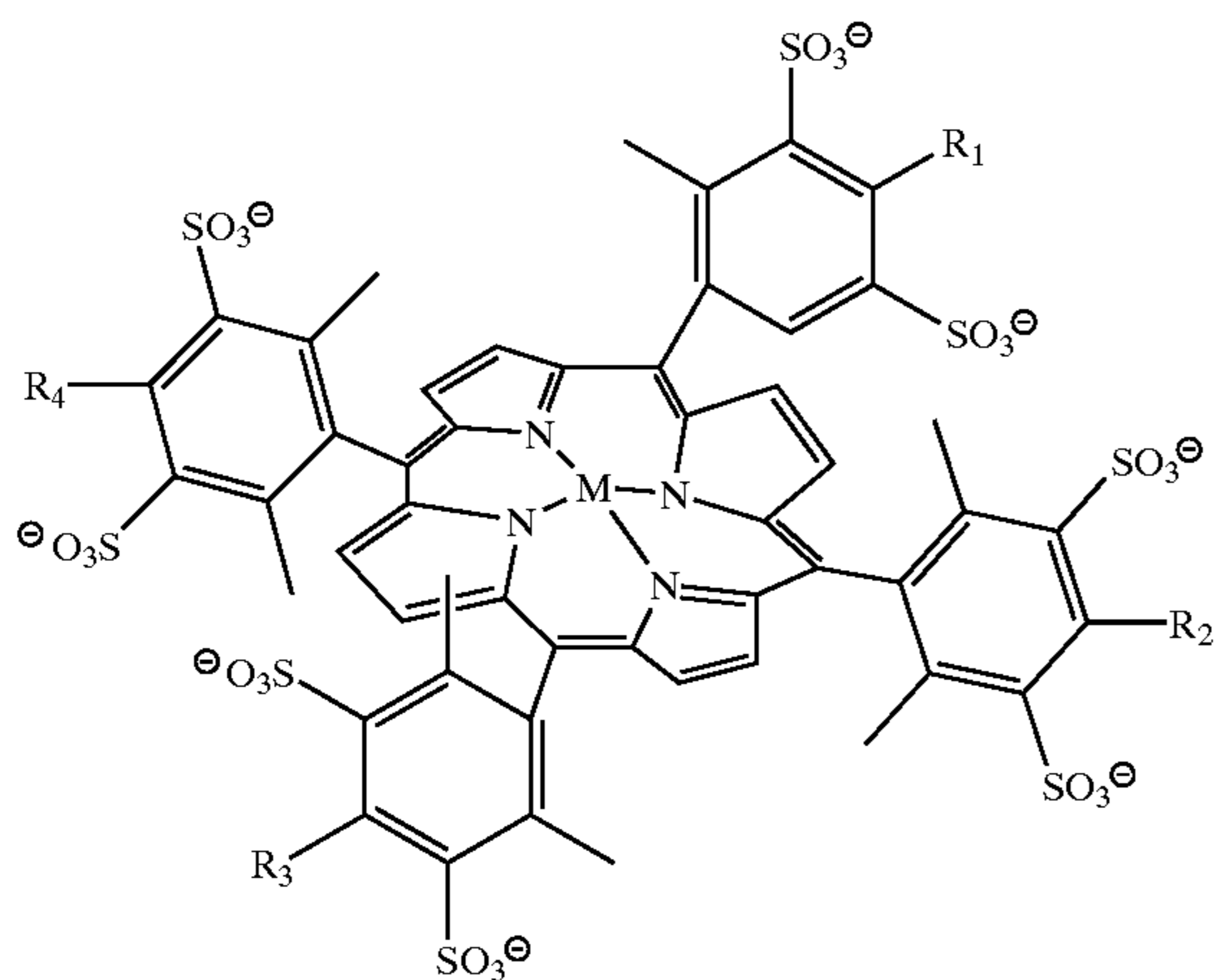
TMPS (R)-Metal complex
