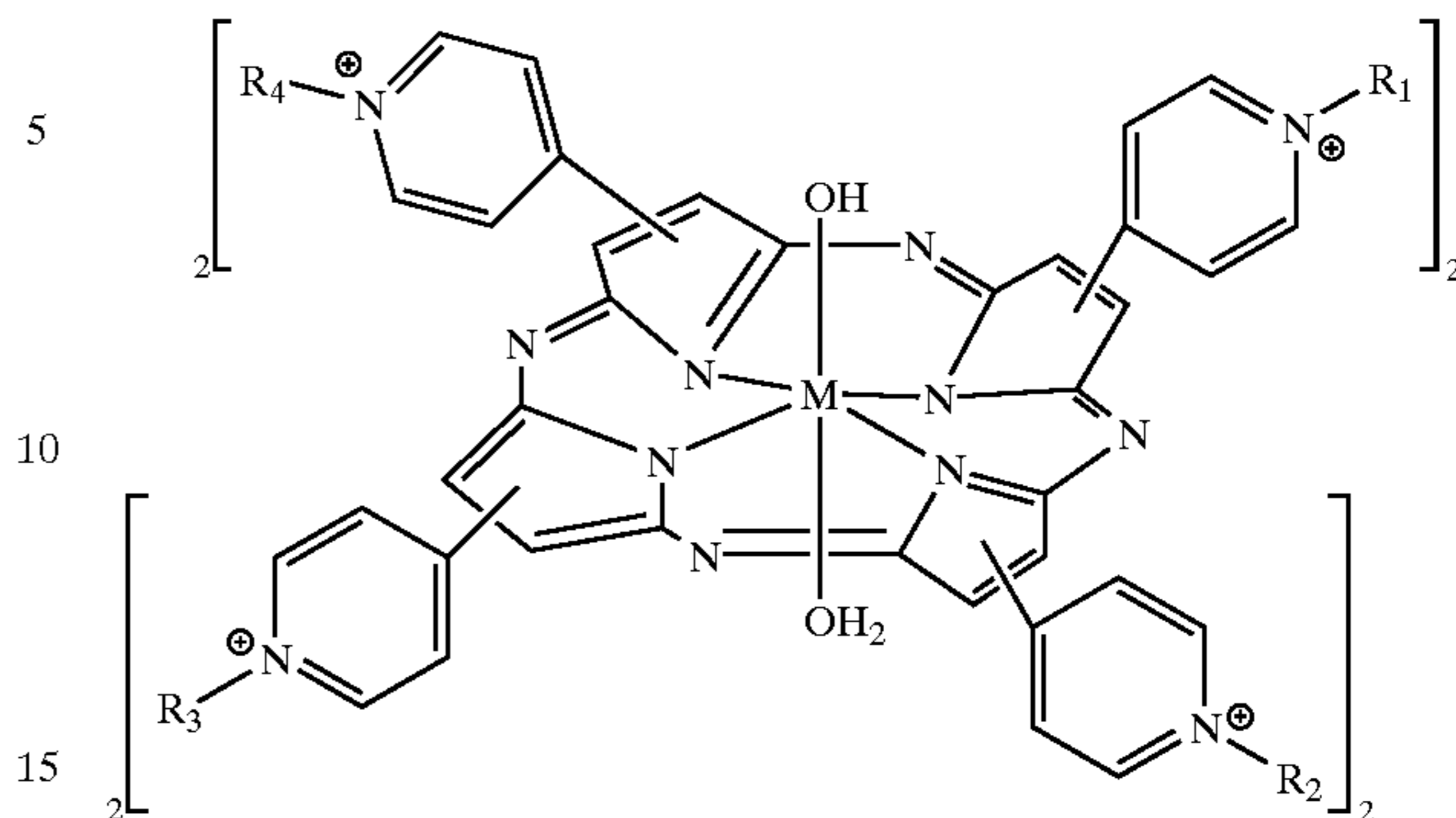
2-, 3-, and 4-R-pyridyl porphyrazine-Metal complexes
