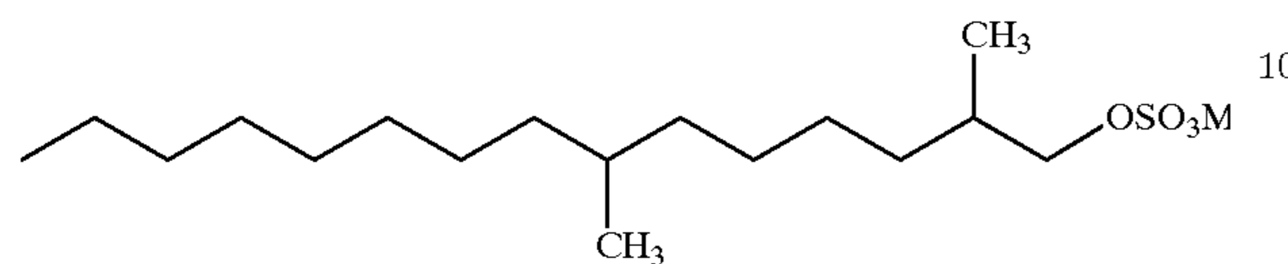
2,7-dimethylpentadecylsulfate having the formula
