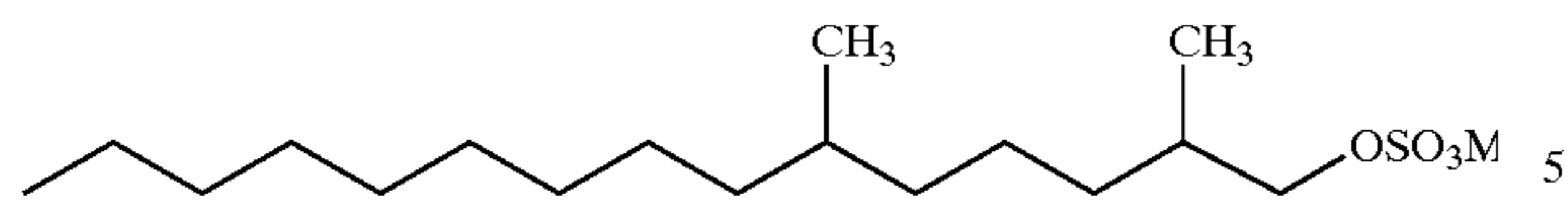
2,6-dimethylpentadecylsulfate having the formula
