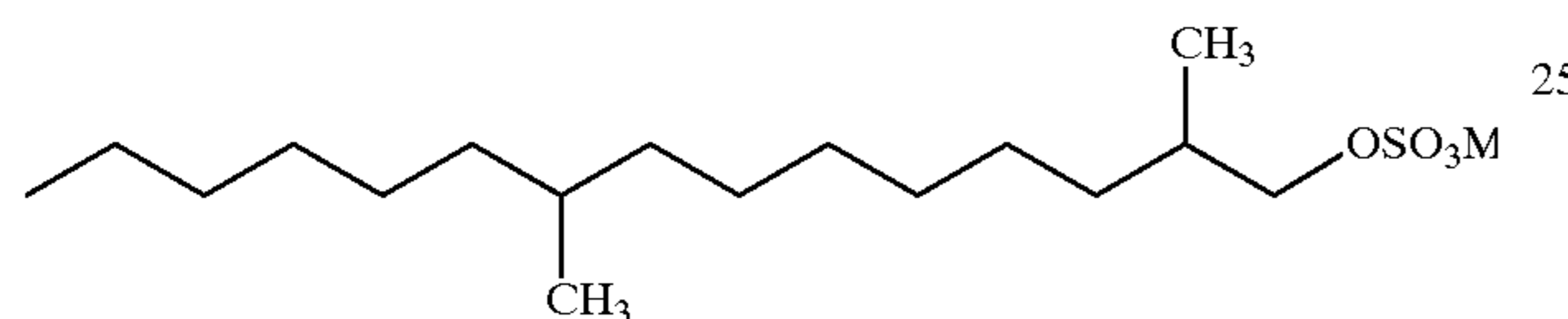
2,9-dimethylpentadecylsulfate having the formula
