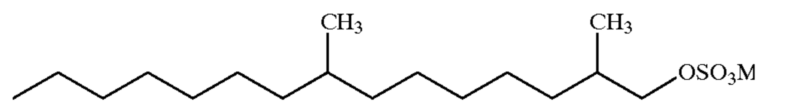
2,7-dimethylpentadecylsulfate having the formula
