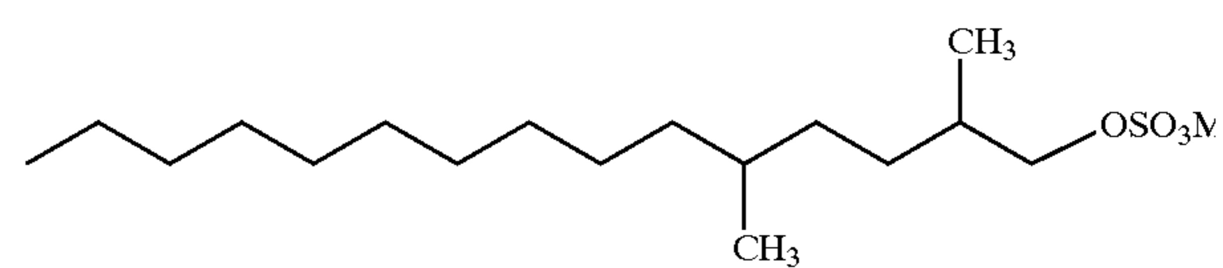
2,5-dimethylpentadecylsulfate having the formula:
