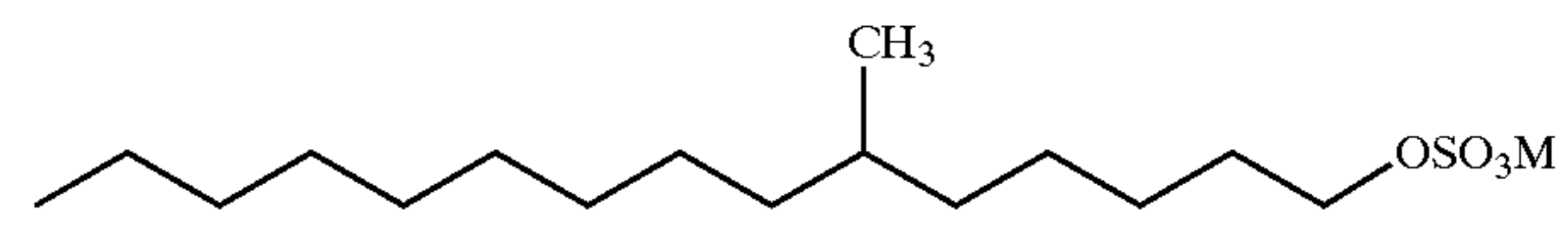
5-methylpentadecylsulfate having the formula:
