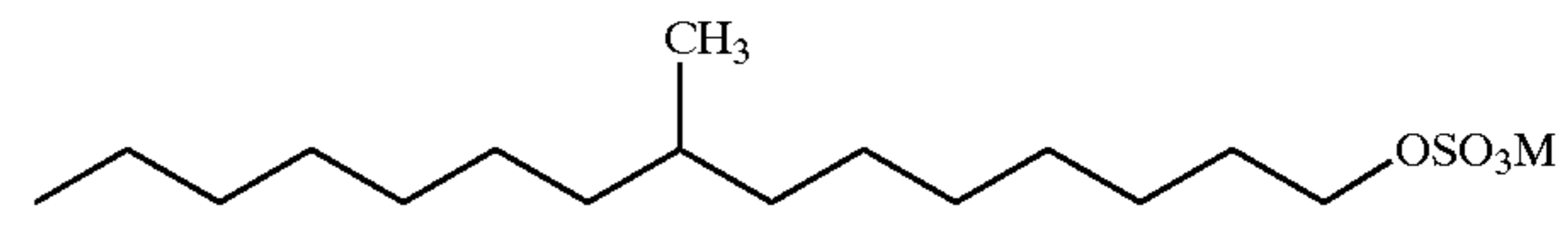
8-methylpentadecylsulfate having the formula
