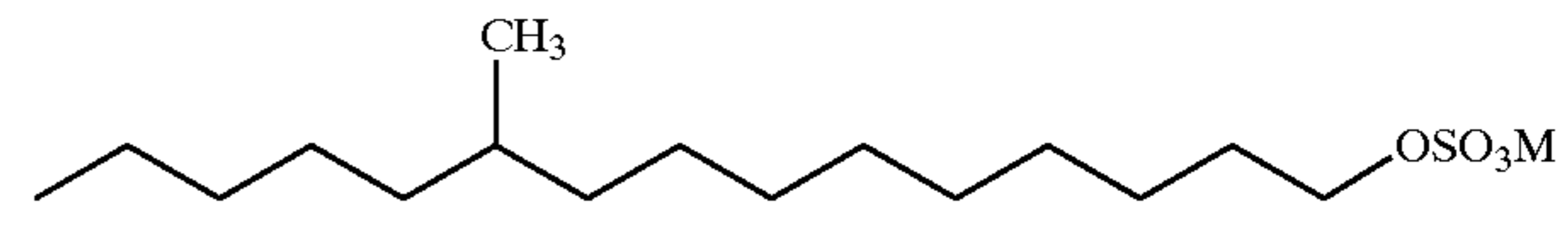
10-methylpentadecylsulfate having the formula
