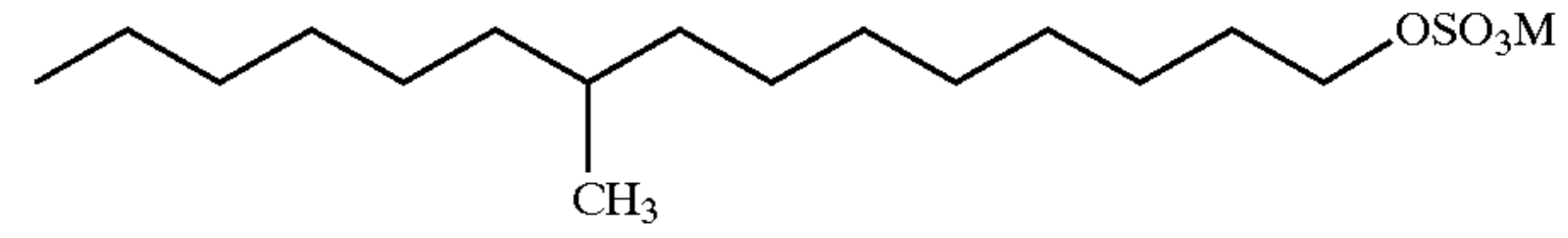
9-methylpentadecylsulfate having the formula
