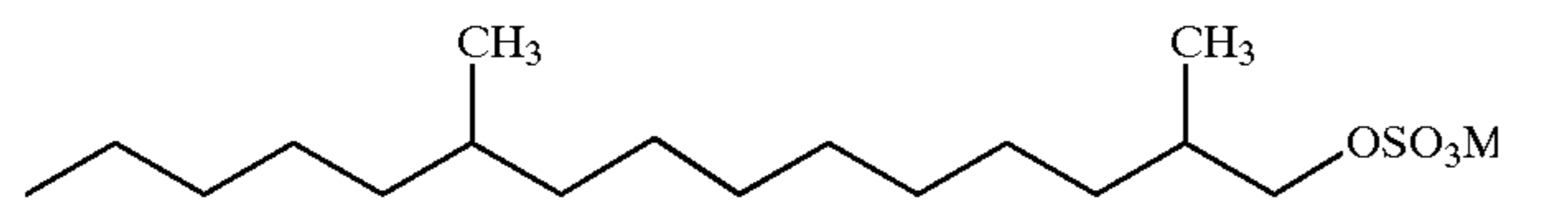
2,10-dimethylpentadecylsulfate having the formula
