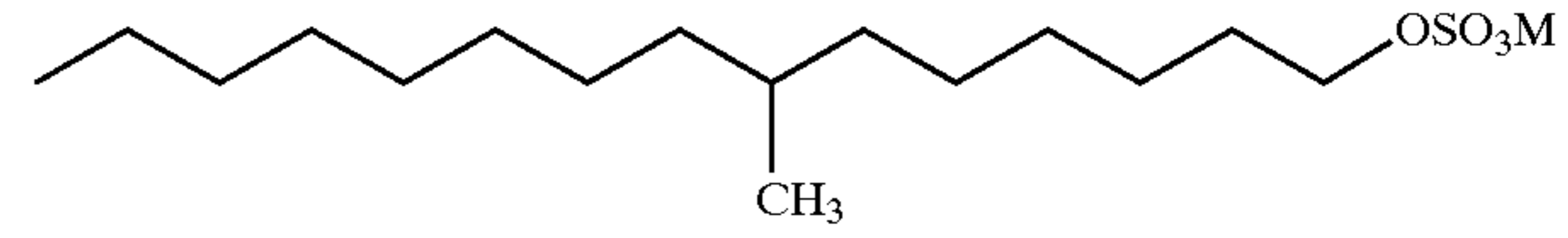
7-methylpentadecylsulfate having the formula
