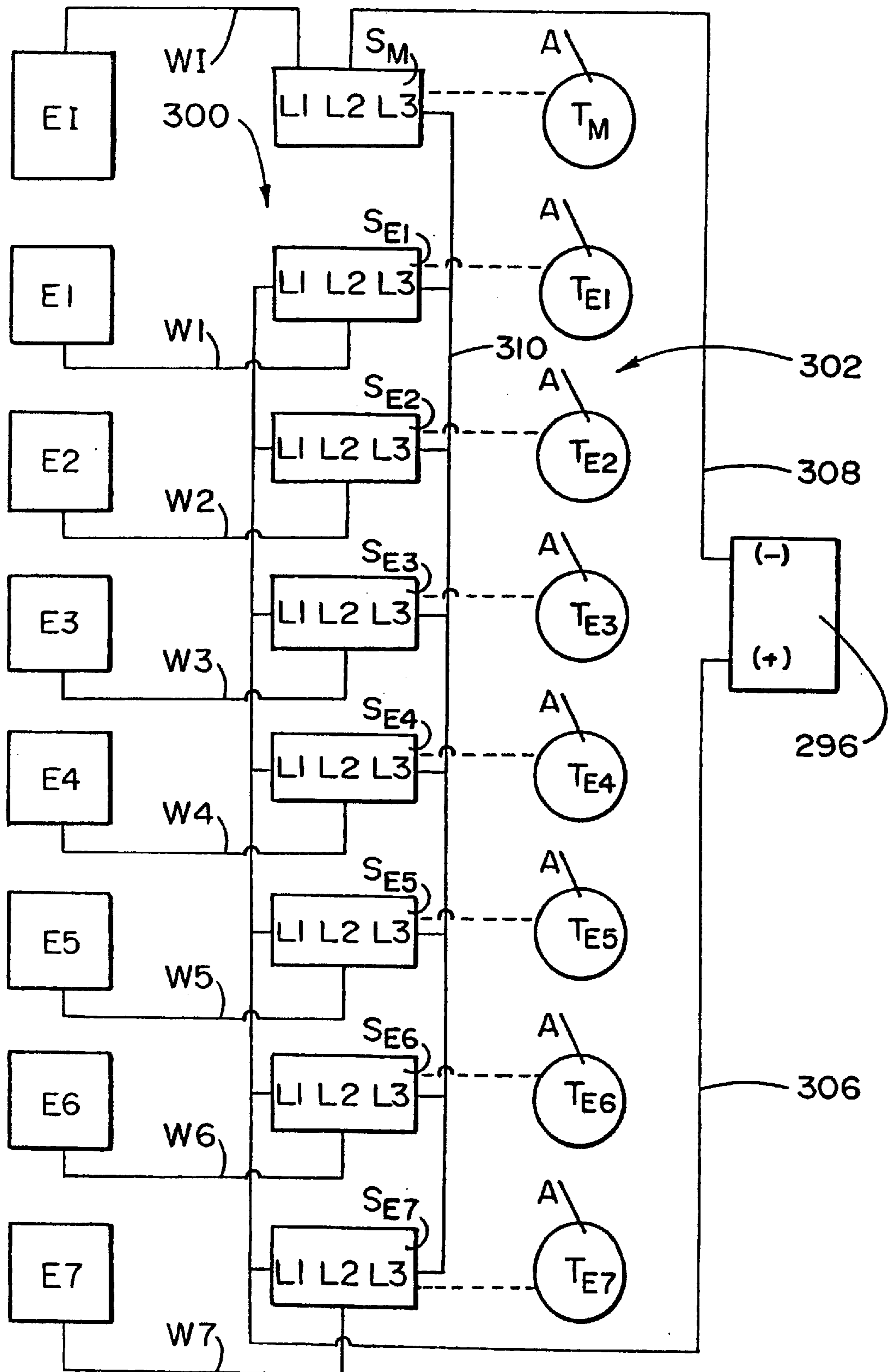
FIG. 63 UNIPOLAR CONTINUOUS
