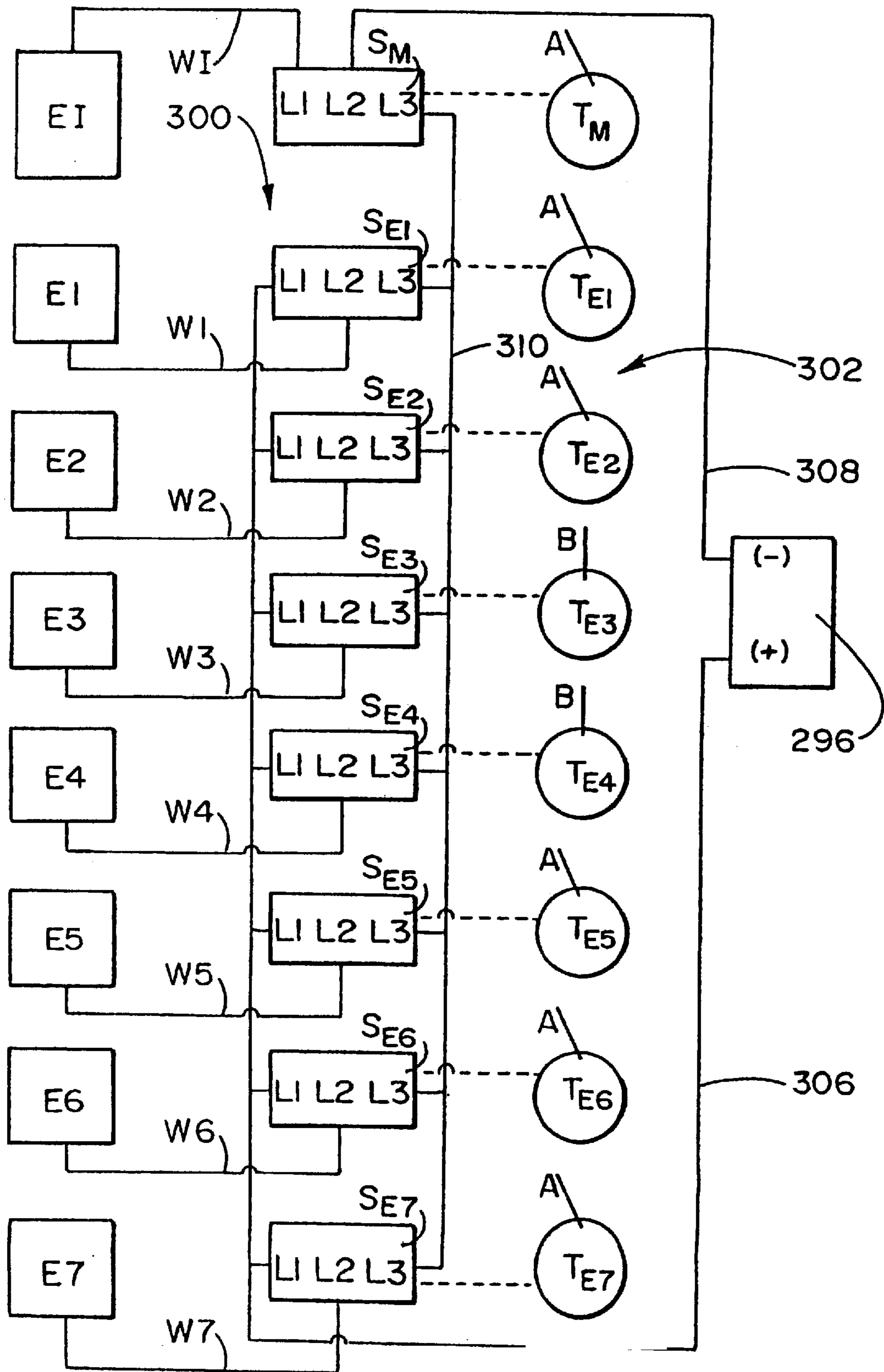
FIG. 64 UNIPOLAR INTERRUPTED
