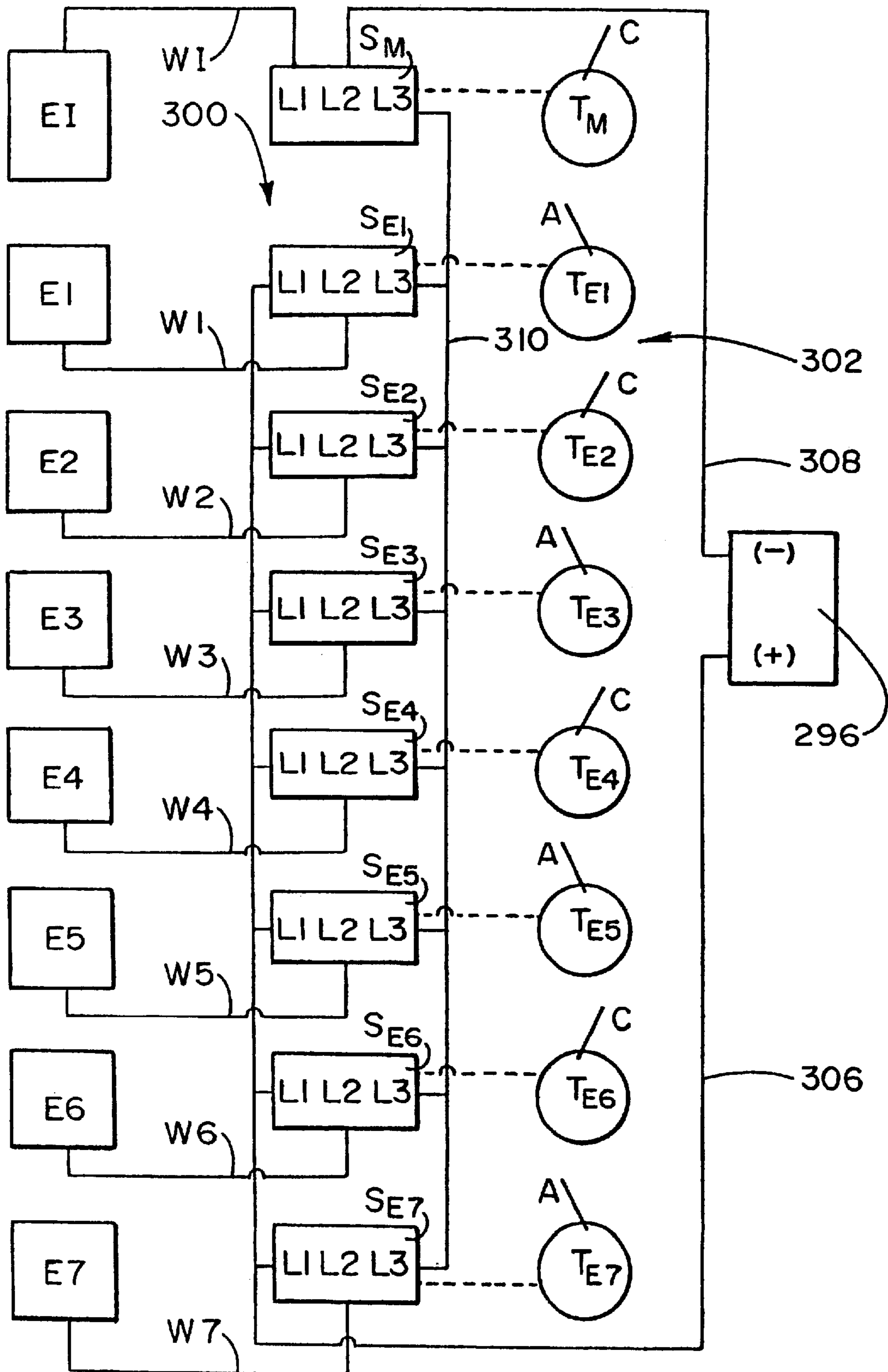
FIG. 65 BIPOLAR CONTINUOUS
