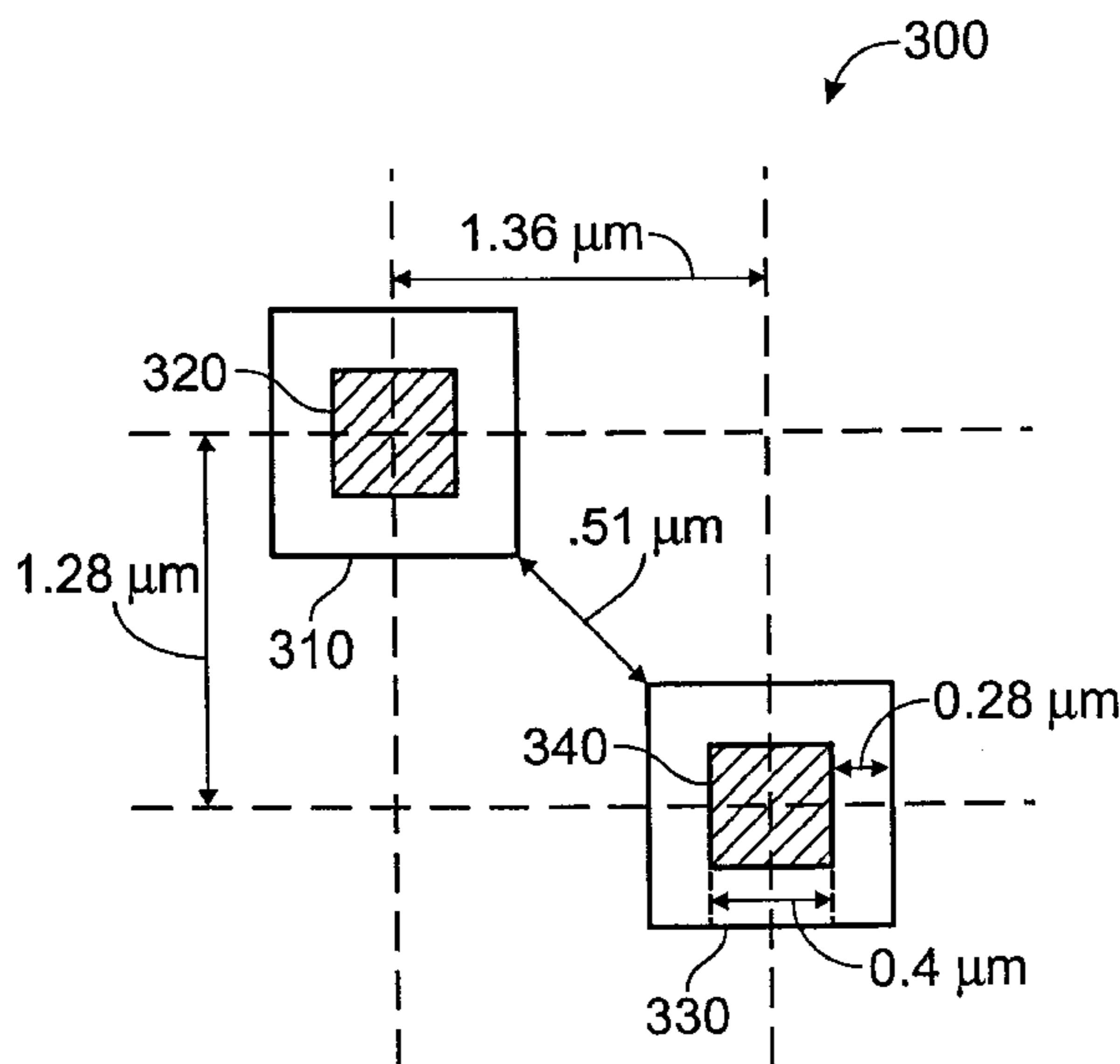
METAL-TO-METAL DESIGN RULES = 0.52 μm
