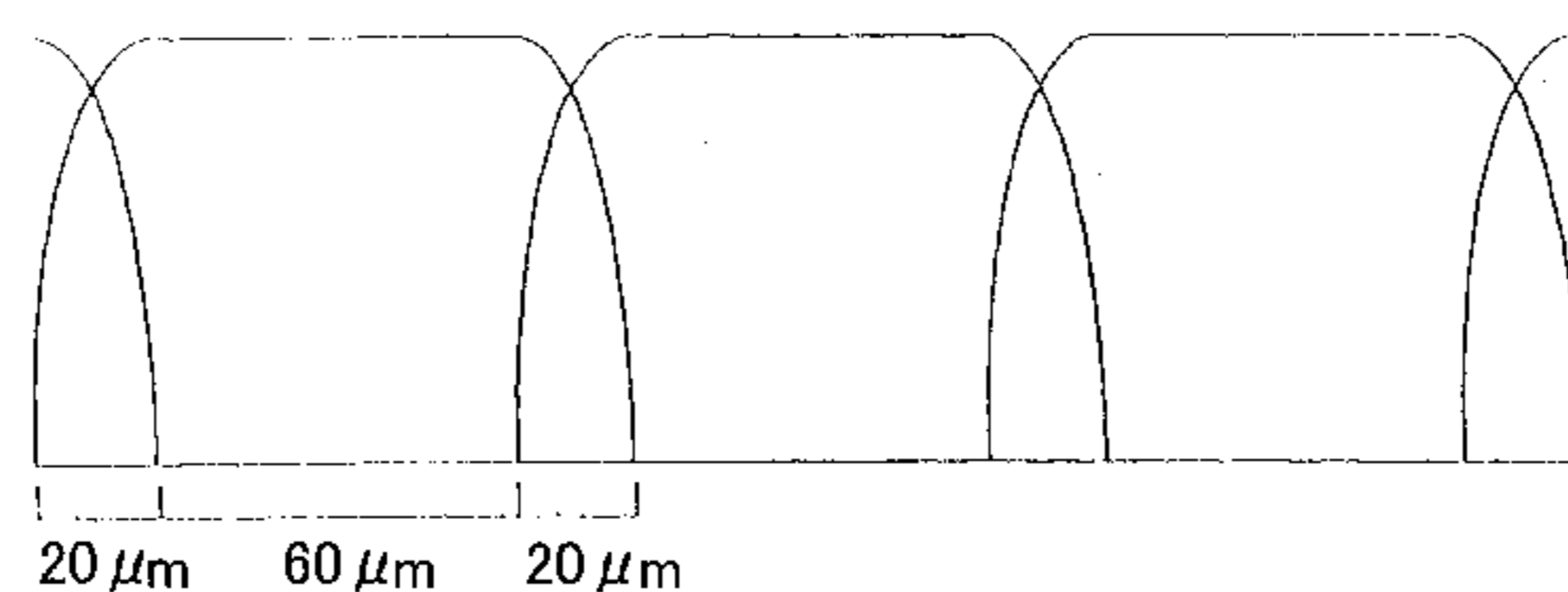
LASER BEAM INTENSITY DISTRIBUTION ON OPTICAL DISK
