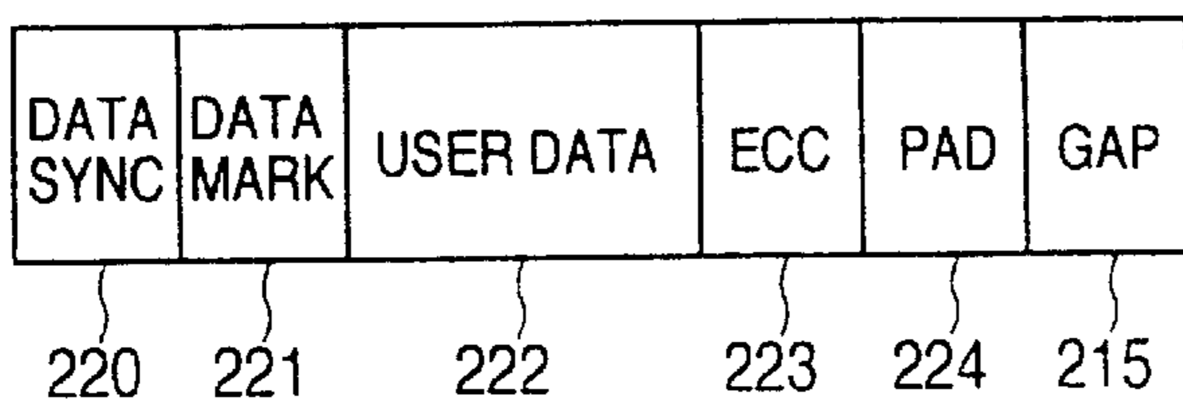
DATA SECTOR FORMAT
