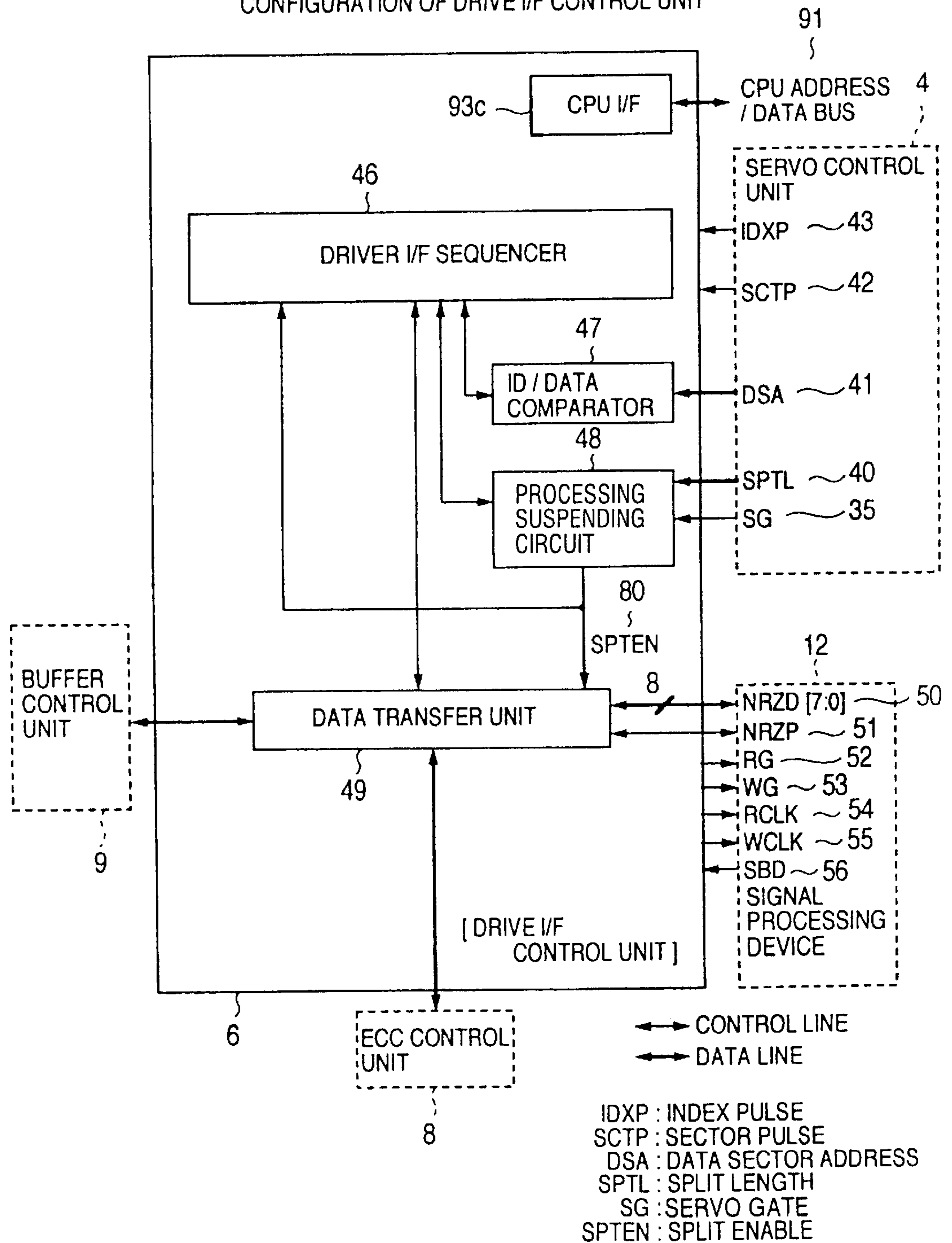
CONFIGURATION OF DRIVE I/F CONTROL UNIT
