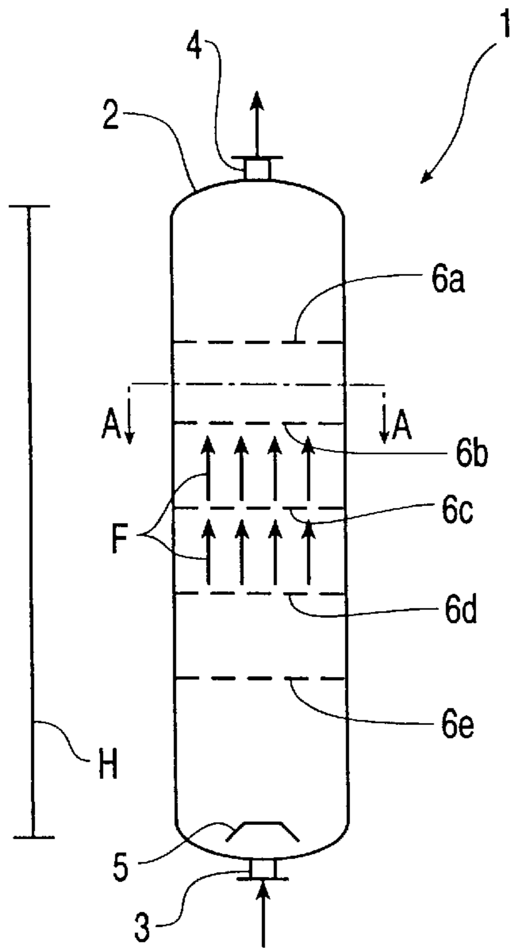
Fig. 1 Prior Art
