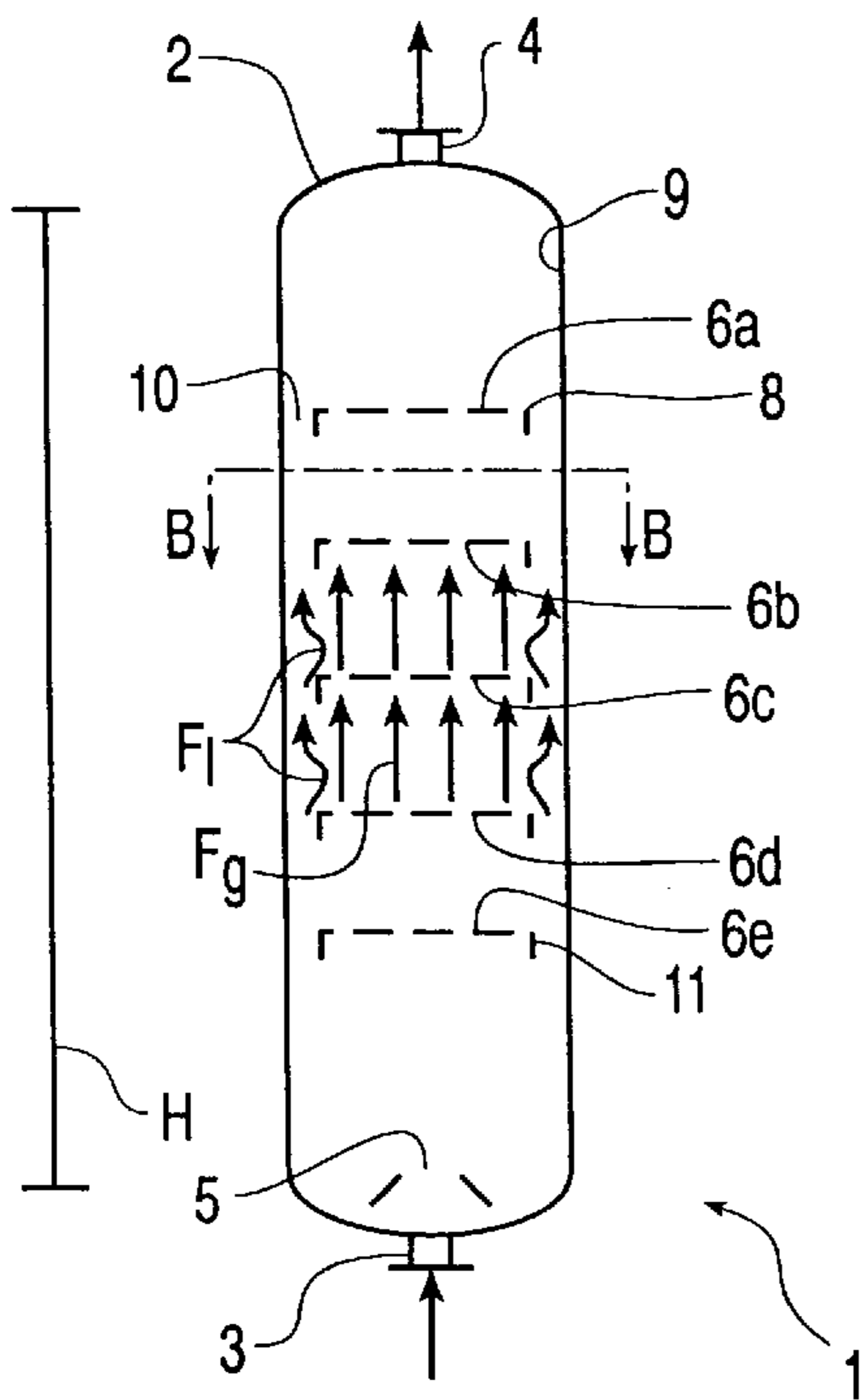
Fig. 3 Prior Art
