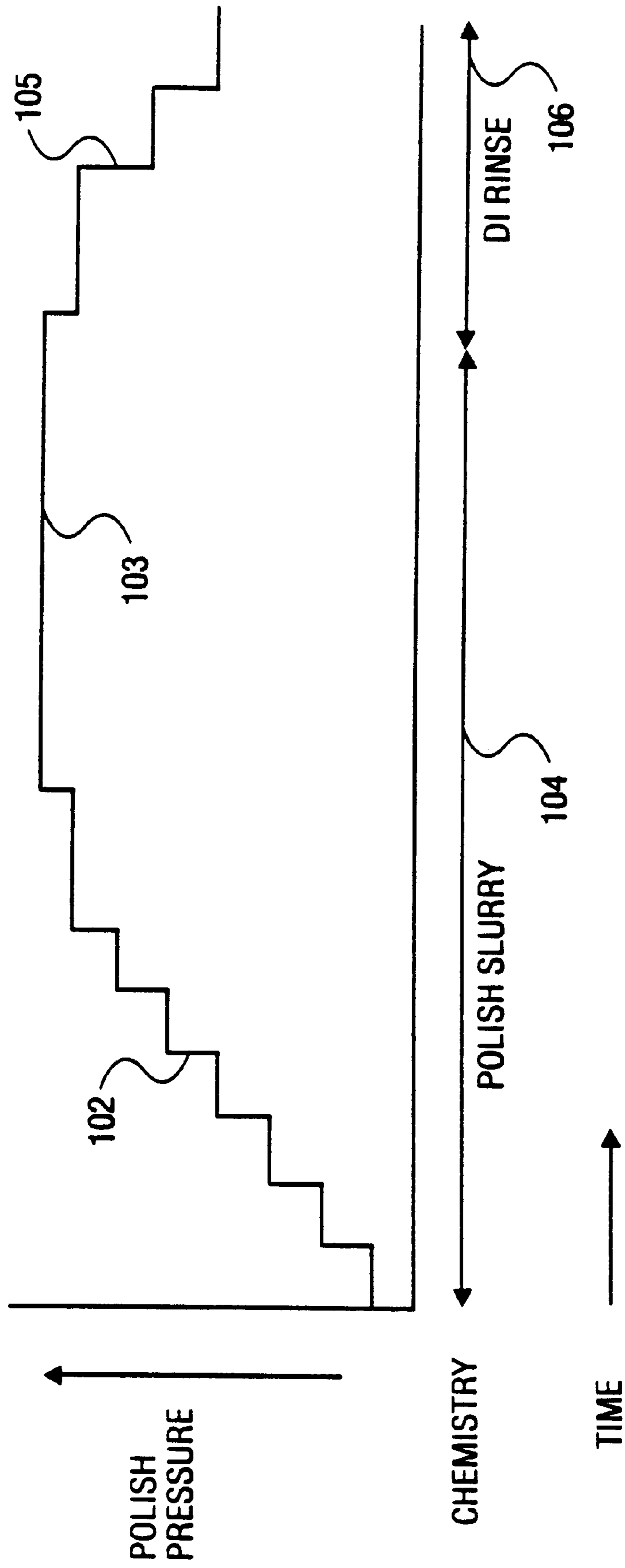
FIG. 1 (PRIOR ART)
