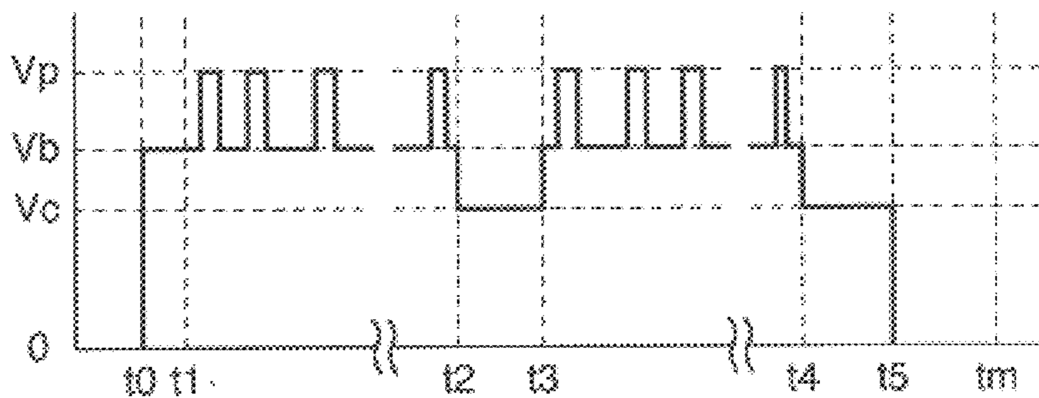
(a) RECORDING ELECTRODE
