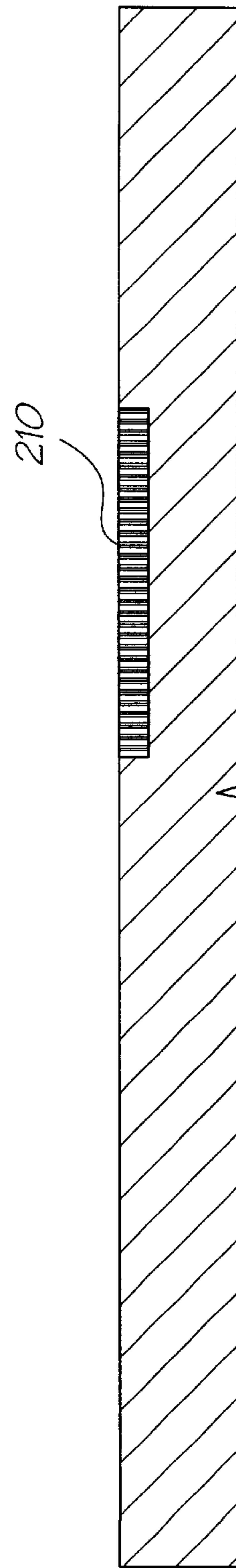
Implant N-Well
