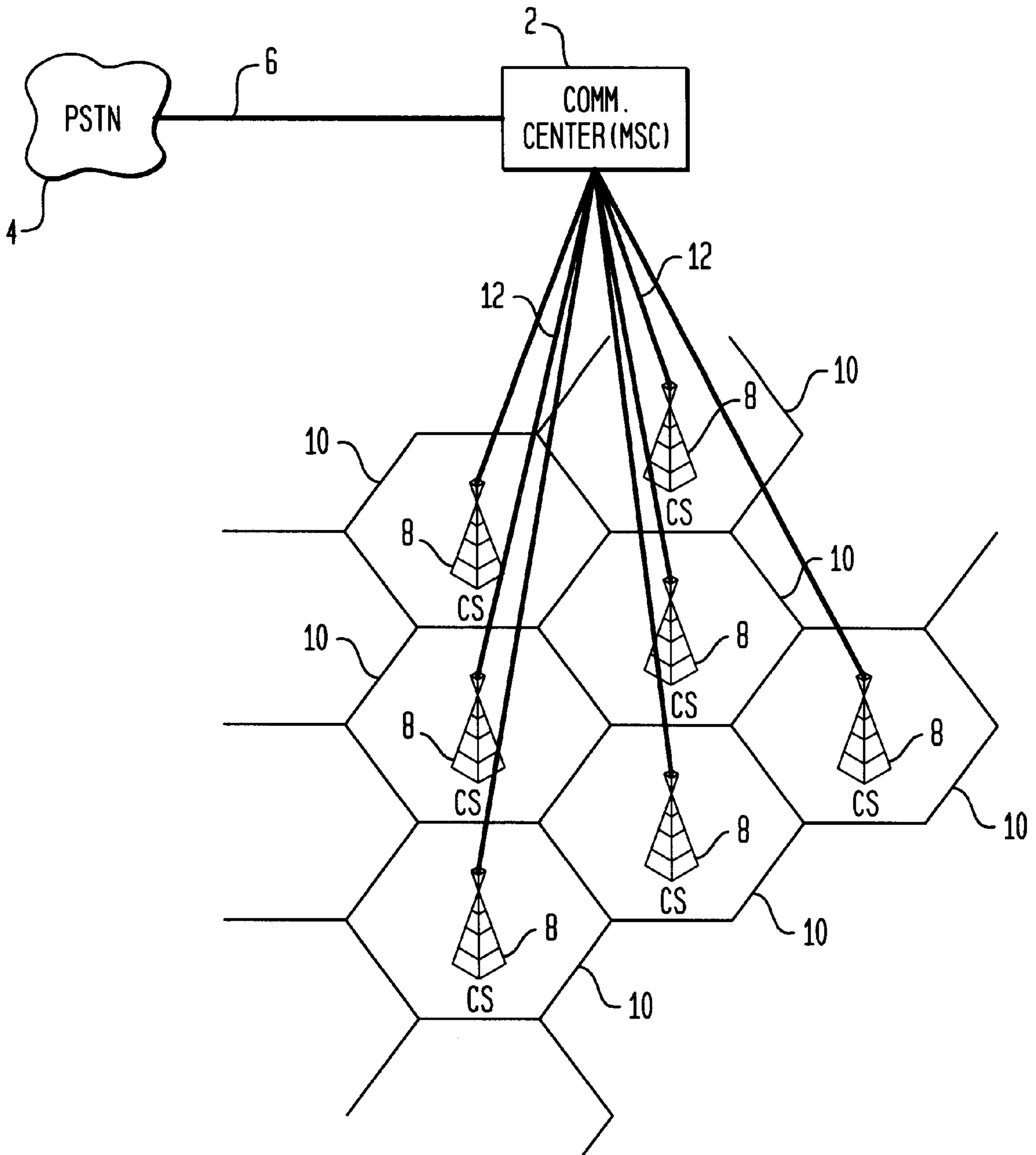
FIG. 1 (PRIOR ART)
