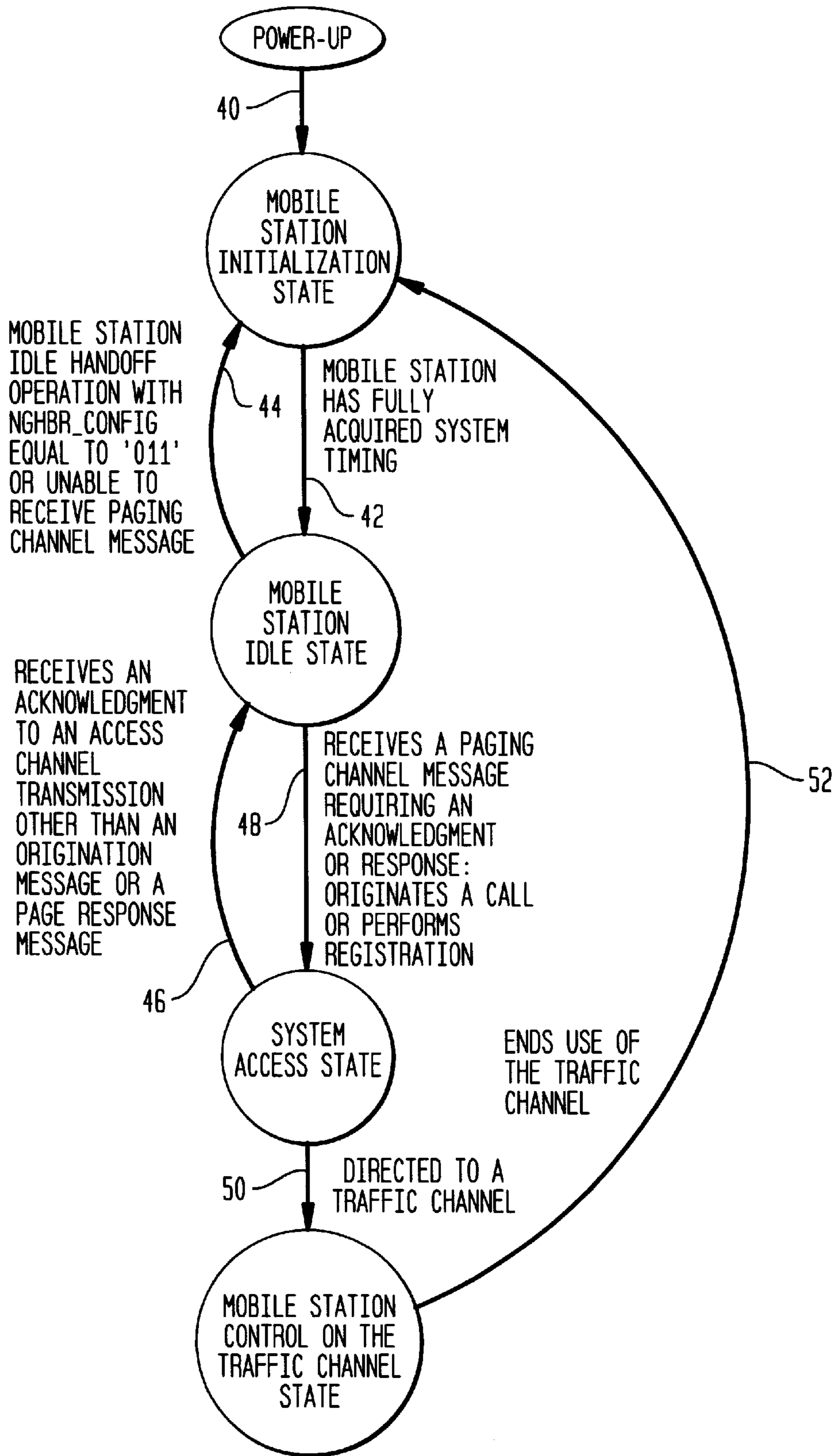
FIG. 4 (PRIOR ART)
