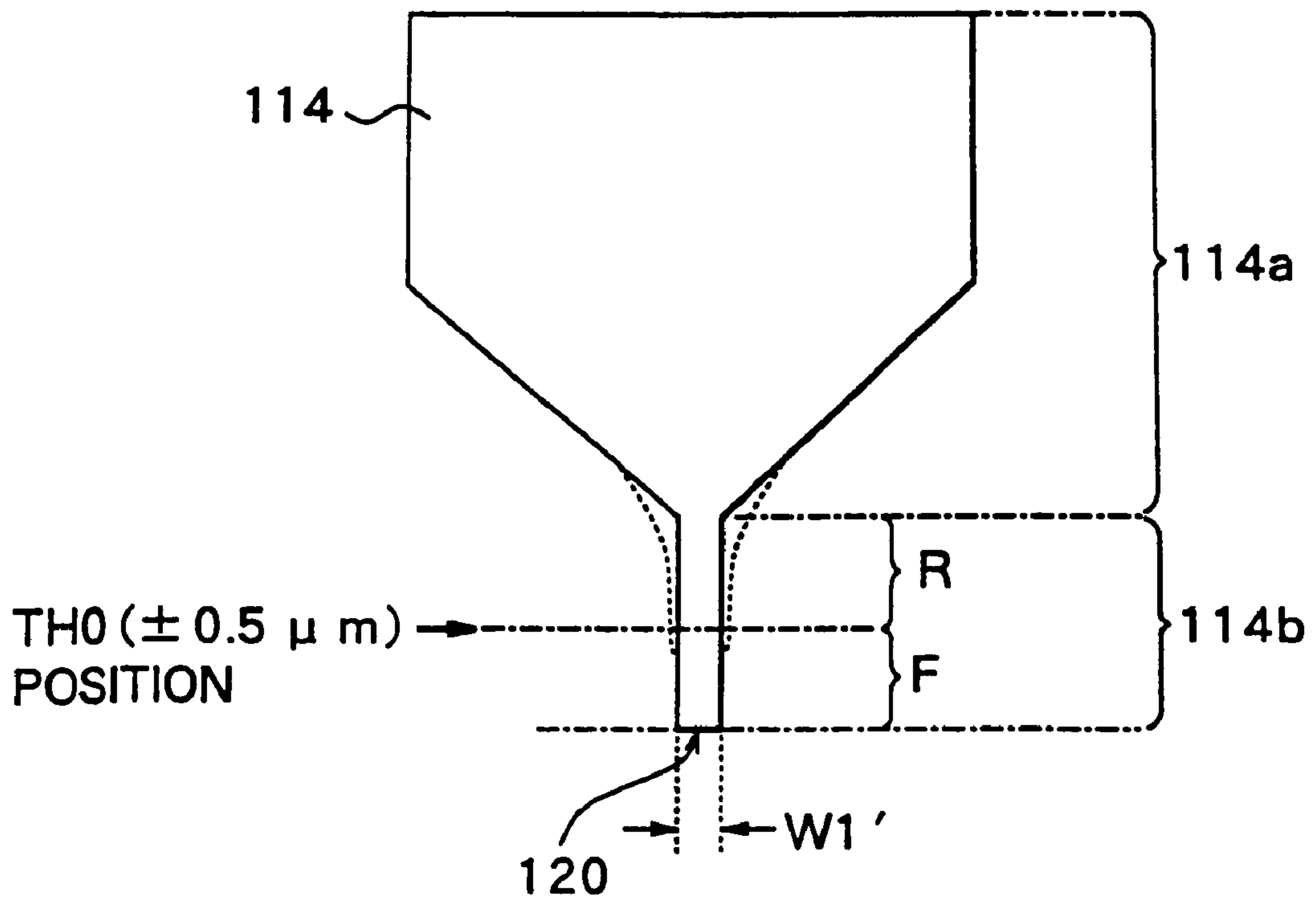
FIG.46 PRIOR ART
