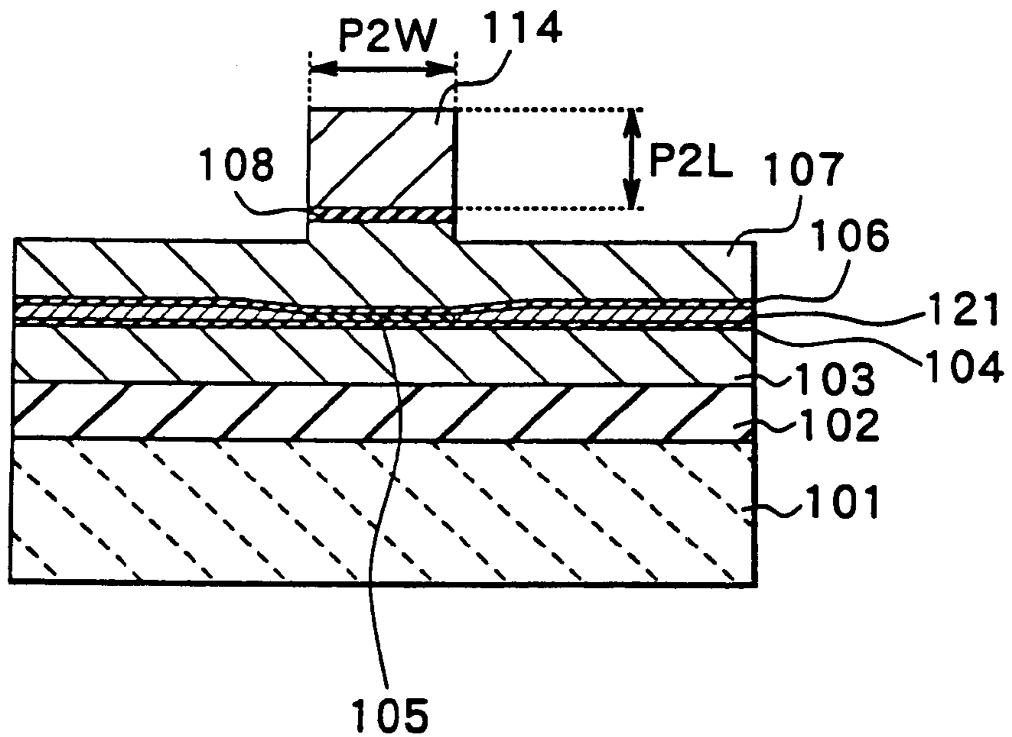
FIG.43 PRIOR ART
