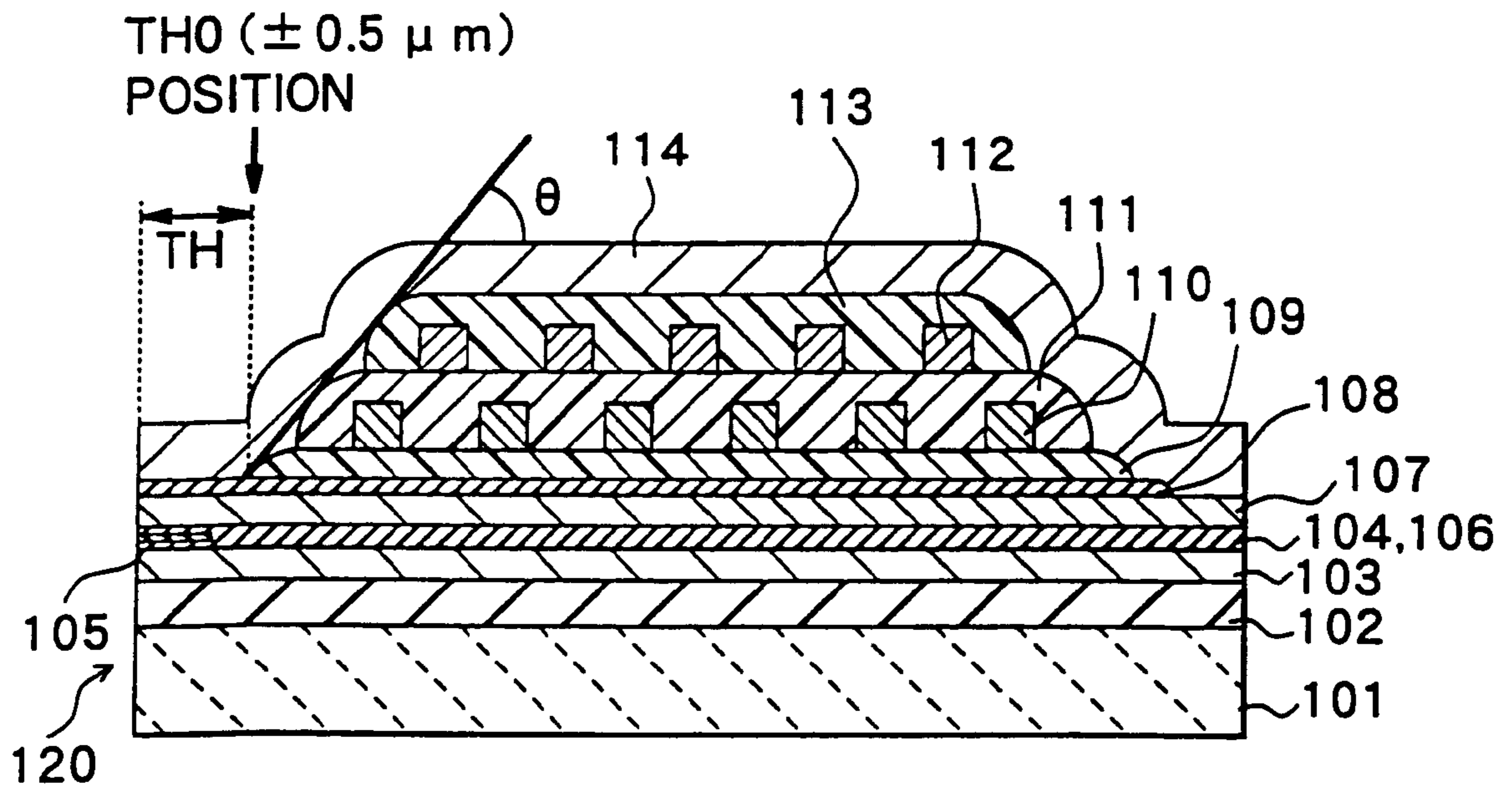
FIG.42 PRIOR ART
