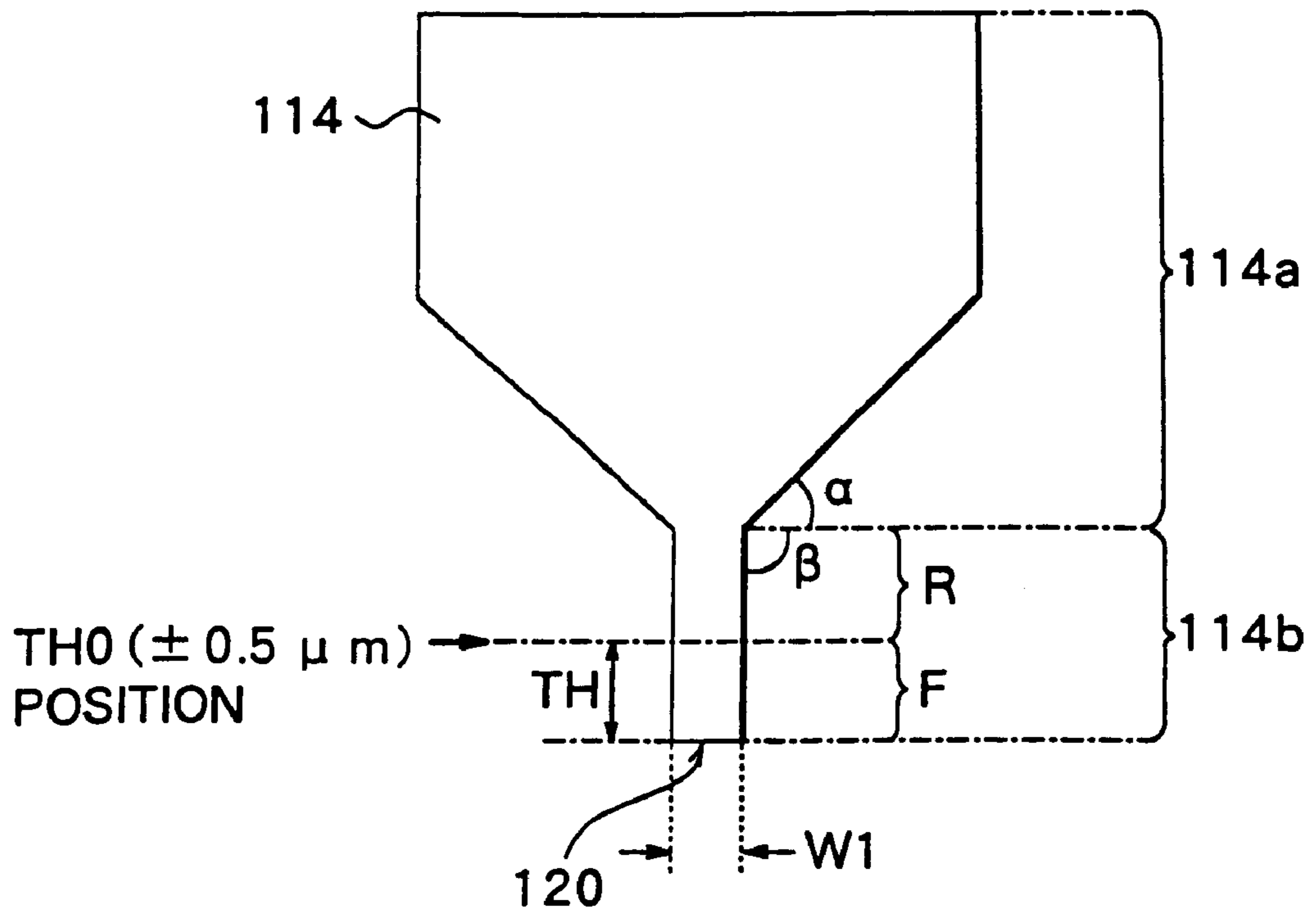
FIG.45 PRIOR ART
