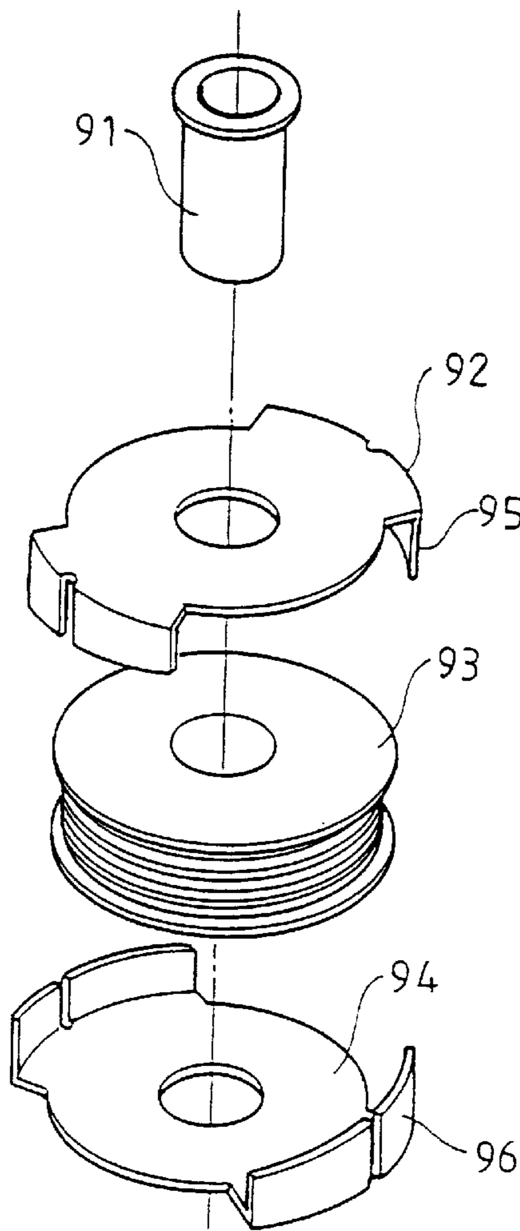
FIG. 11 PRIOR ART
