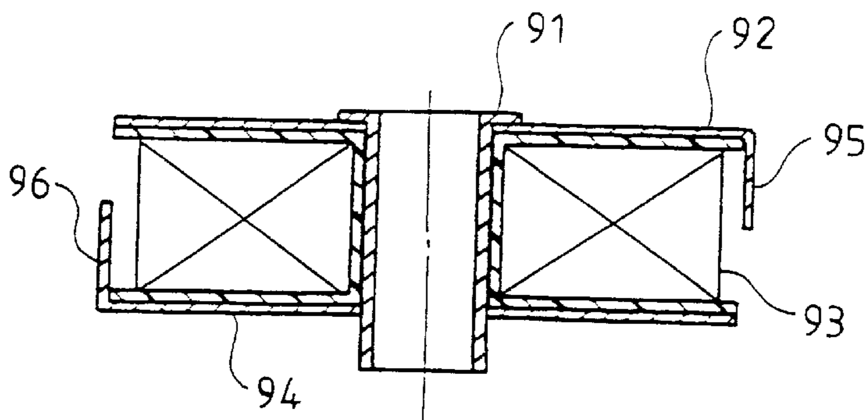
FIG. 12 PRIOR ART
