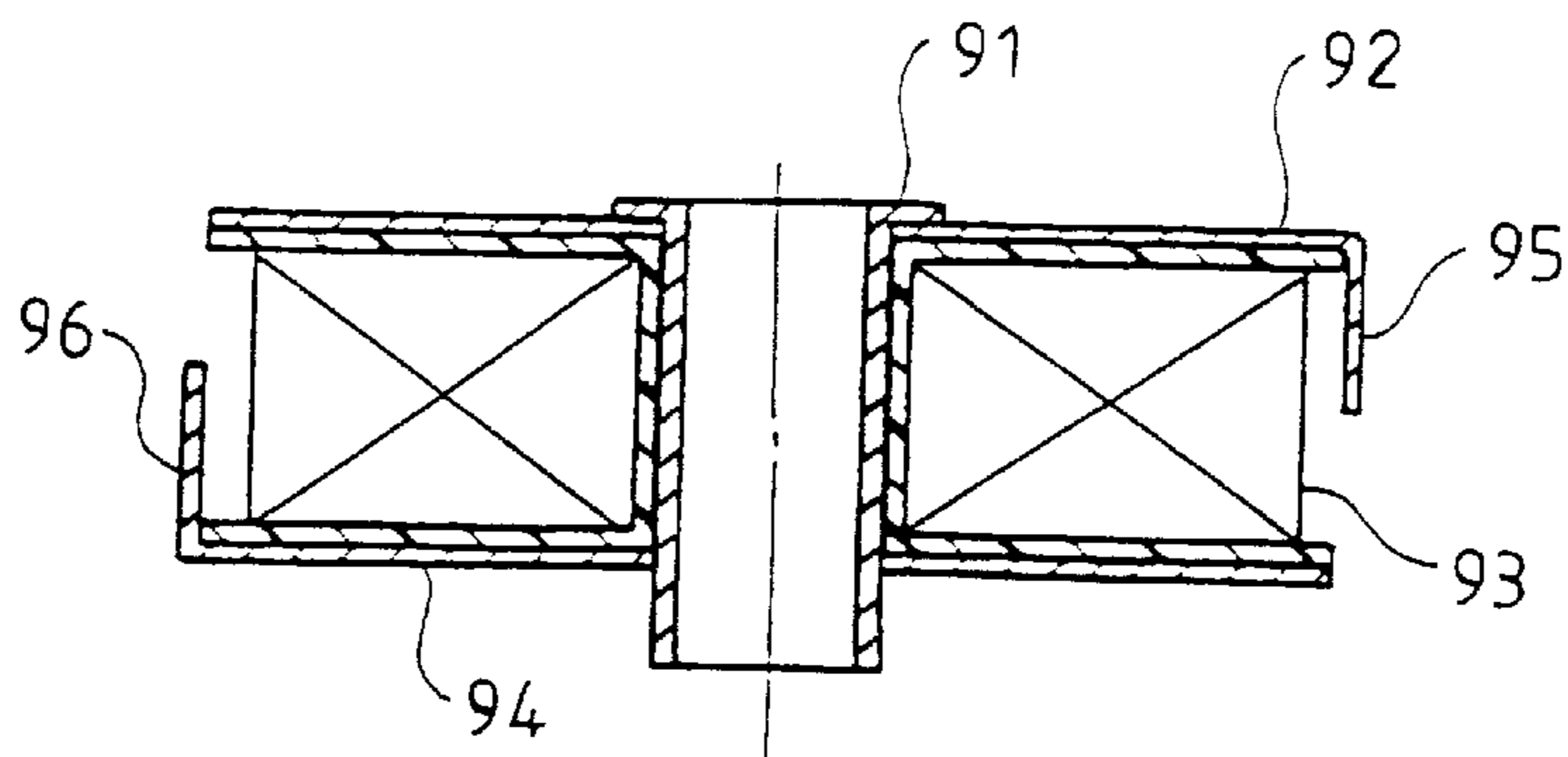
FIG. 12 PRIOR ART
