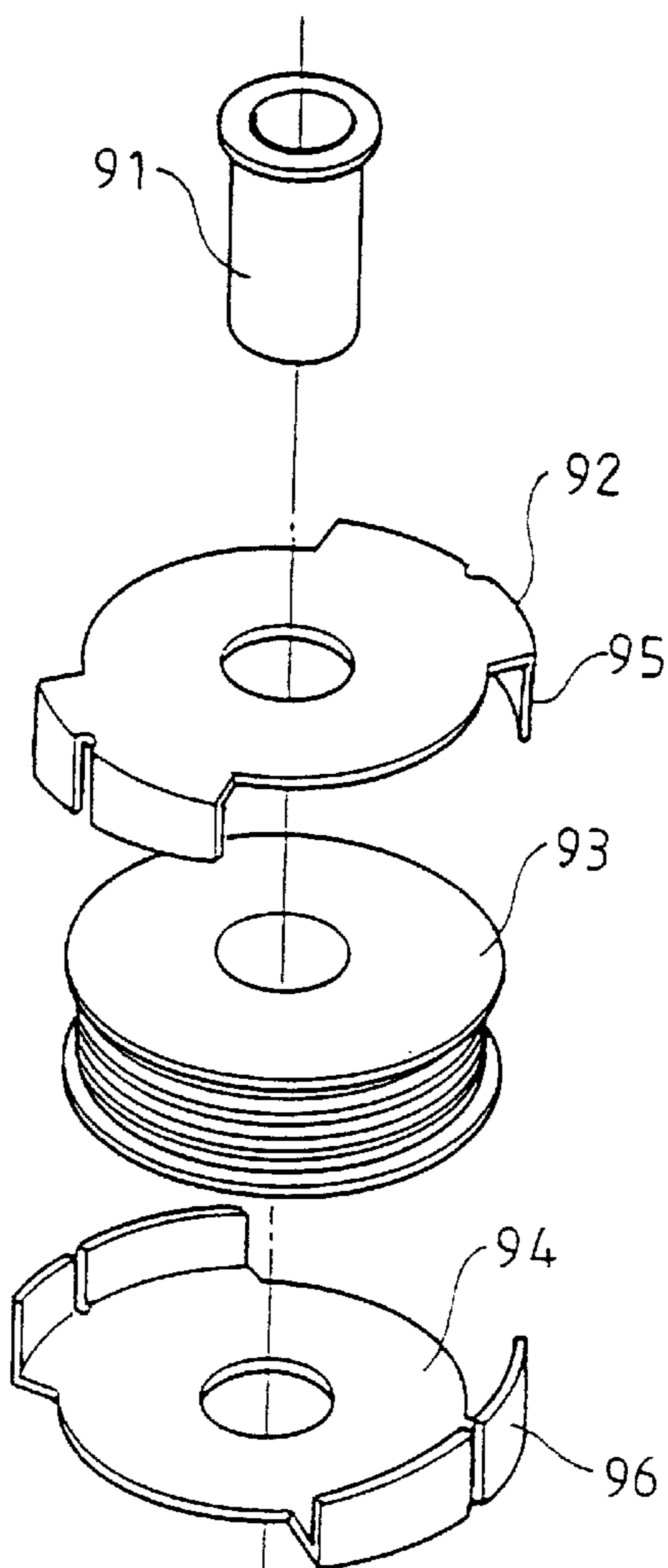
FIG. 11 PRIOR ART
