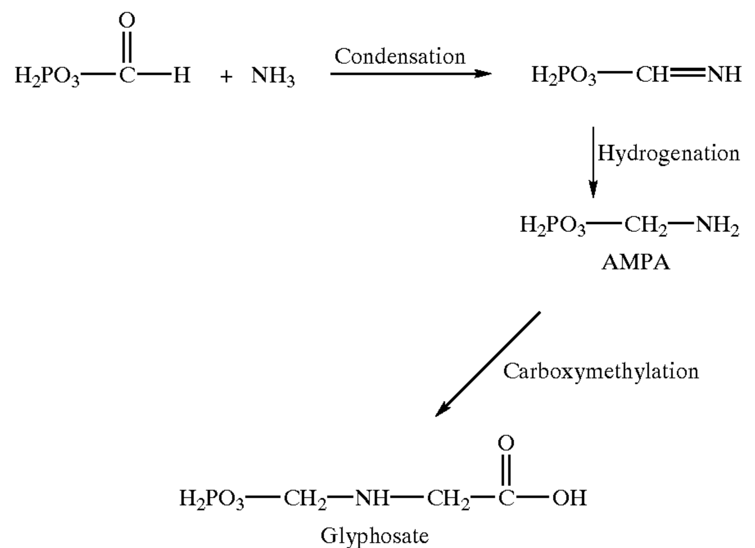
Scheme IV
