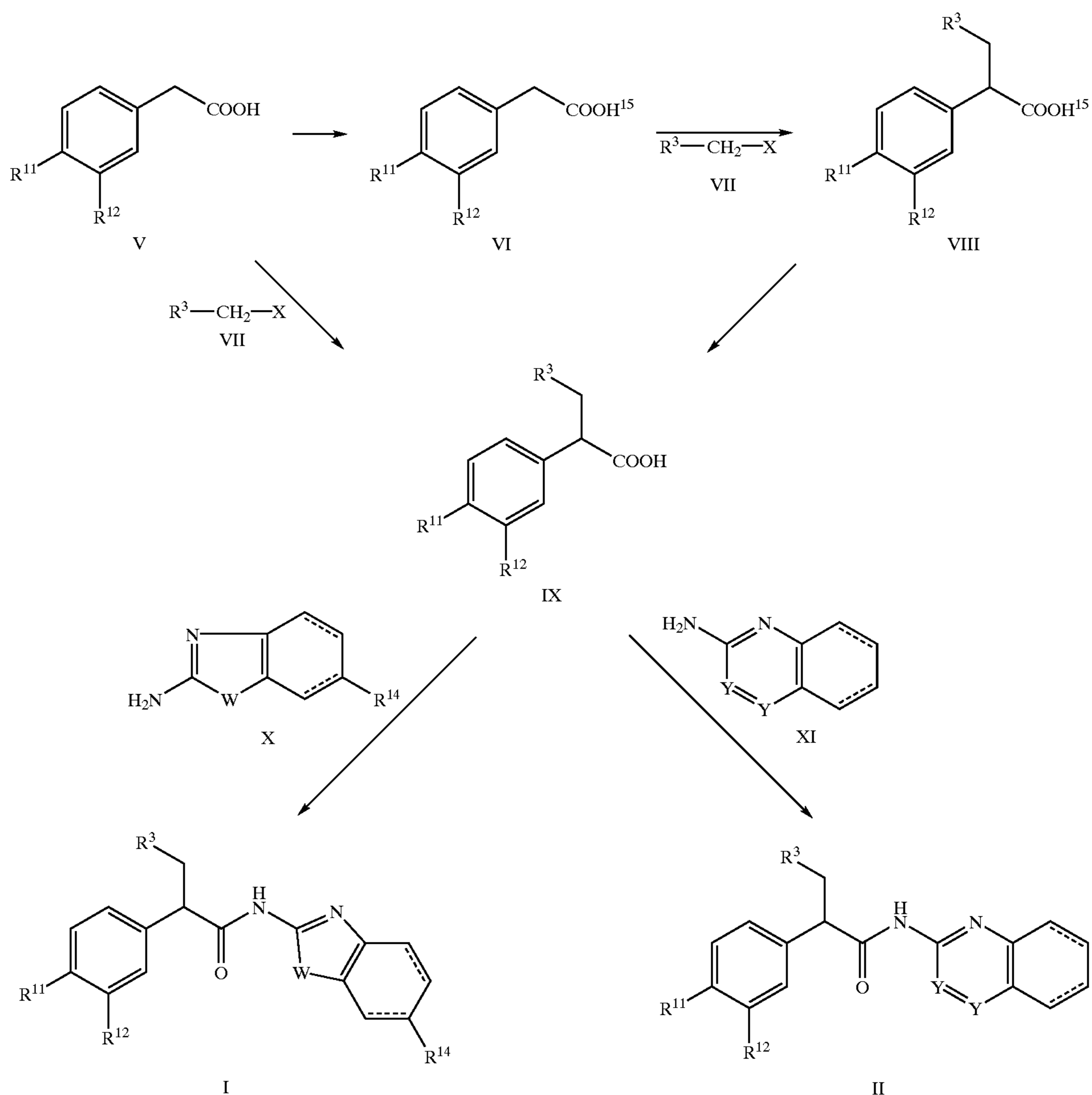
Reaction Scheme
