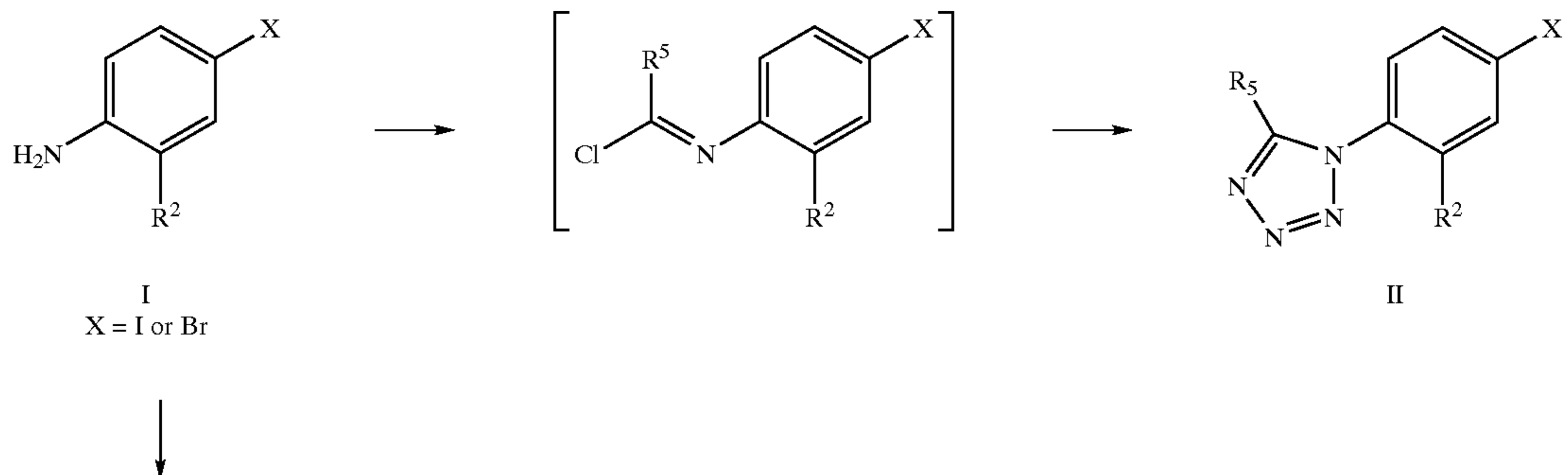
Scheme 1 Tetrazole Starting Materials
