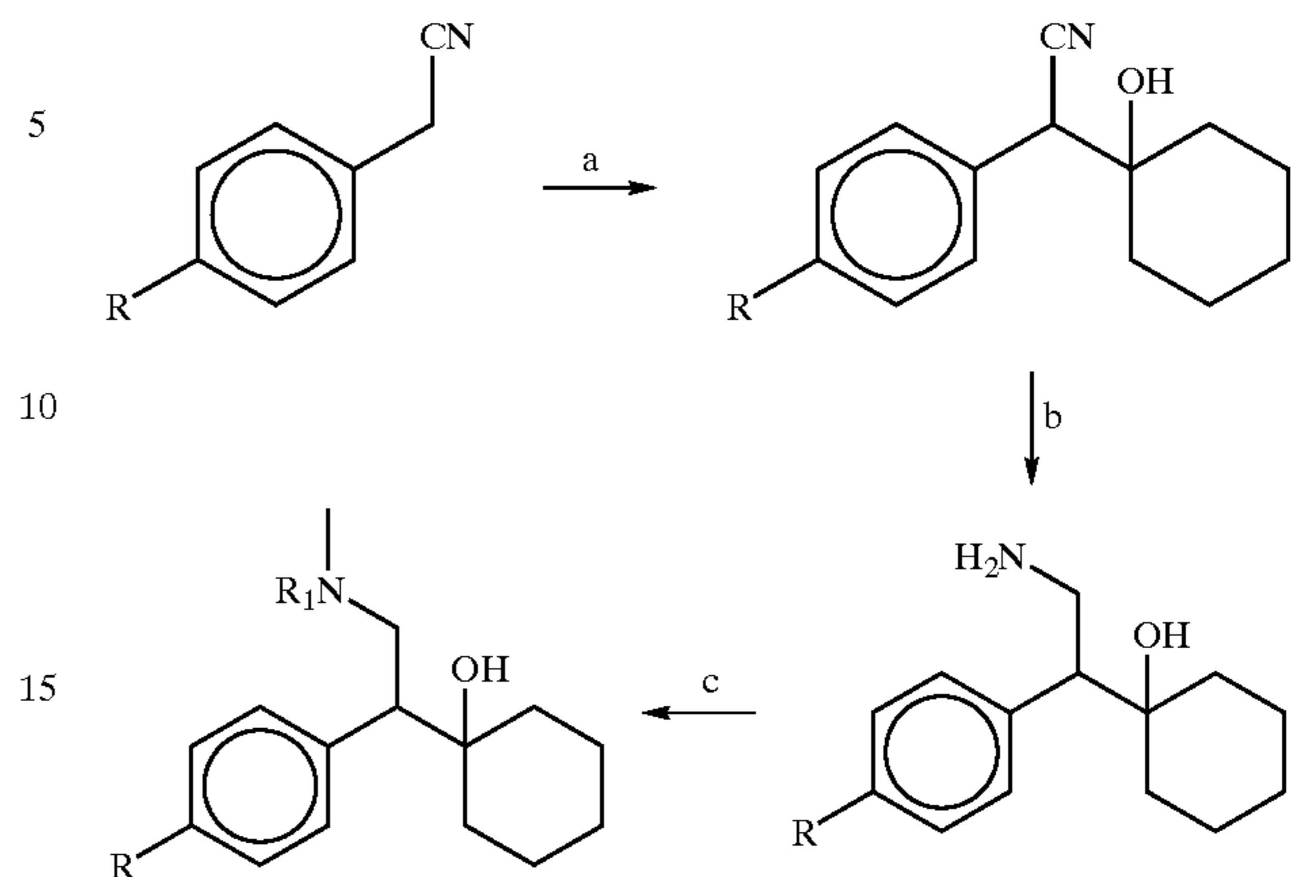
Scheme II
